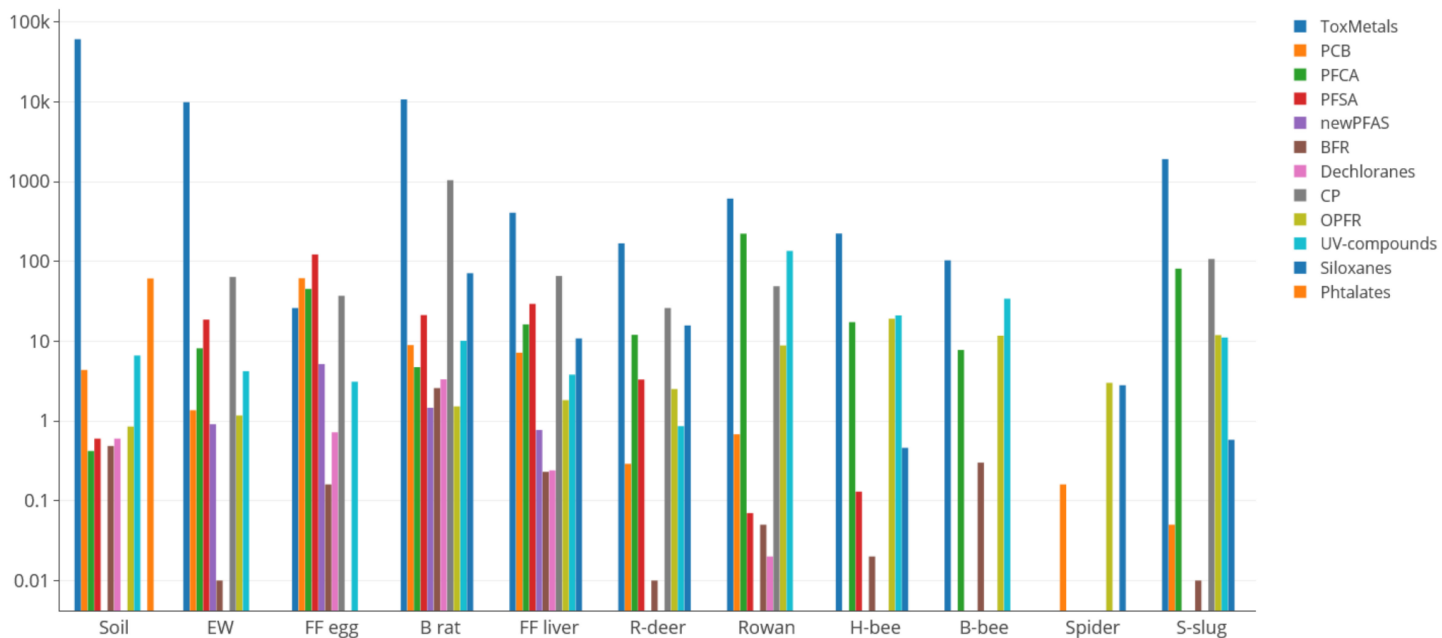
Figure 12: Sum values for contaminant classes in the various samples: Soil, earth worm (EW), fieldfare egg (FF egg), brown rat (B rat), Fieldfare liver (FF liver), R-deer, rowan, honey bee (H-bee), bumble bee (B-bee), spider and Spanish slug (S-slug). Concentrations below LOD are not included. Note log-scale at y-axis. All samples in ng/g ww, except soil in ng/g dw and spider as ng/sample.
