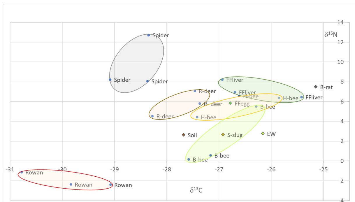
Figure 4: Relationship between the dietary descriptors \delta^{15}\text{N} and \delta^{13}\text{C} in soil and biota samples from urban terrestrial environment in Oslo, 2021; soil (S), earthworm (EW), brown rat (Rat), slug (S-slug), fieldfare egg (FF egg), fieldfare liver (FFliver), Roe deer liver (Roe deer), spider, rowan, honey bee (H-bee) and bumble bee (B-bee). Note that only one sample exist for soil, earthworm, fieldfare egg and rat and slug. These are marked with various colours and diamond symbol.
