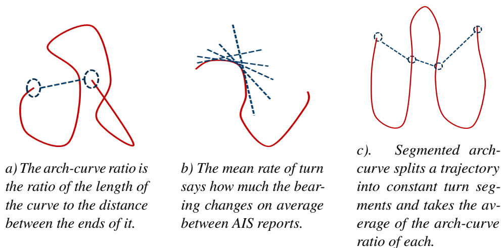
Figure 5.2 Tortuosity measures.
