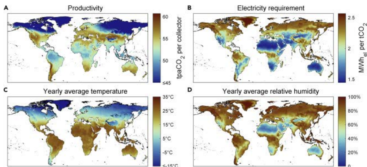
Figure 27 – DAC global performance (A) \text{CO}_2 collector productivity obtained using hourly \text{CO}_2 production averaged over the year, assuming -15^\circ\text{C} as a minimum operating temperature for the DAC plant. (B) The average electricity requirement for the yearly \text{CO}_2 production. The current benchmark DAC solid-sorbent (i.e., Climeworks Lewatit VP OC 1065) is used when calculating global productivity (A) and electricity requirement (B) where future climate-tailored sorbents can be developed, potentially impacting regional differences in DAC performance. Also, it is assumed that when the temperature is below 1^\circ\text{C} , process performance is fixed to the performance of operating at 1^\circ\text{C} . (C) Yearly average temperature. (D) Yearly average humidity (picture reproduced from Sendi et al., Geospatial analysis of regional climate impacts to accelerate cost-efficient direct air capture deployment, One Earth, Volume 5, Issue 10, 1153 – 1164 under Creative Commons Attribution License CC BY 4.0)
