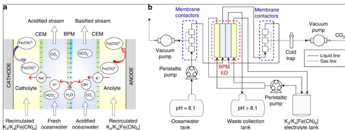
Figure 39 Schematic illustration and the BPM electrodiolysis and \text{CO}_2 capture system (Picture reproduced from Digdaya et al., A direct coupled electrochemical system for capture and conversion of \text{CO}_2 from oceanwater, Nature Communications, 11, 2020, under Creative Commons Attribution License CC BY 4.0)
