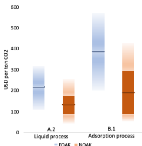
Figure 1 Range for abatement costs for hypothetical cases with different assumptions, for first of a kind (FOAK) and n th of a kind (NOAK) DAC plant, USD per ton of CO 2 captured.
