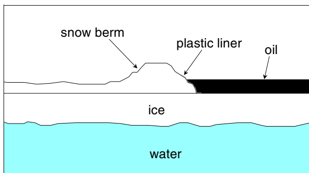
Figure 5 - 10 Snow berm
