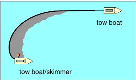
Figure 5 - 4 J-boom configuration
