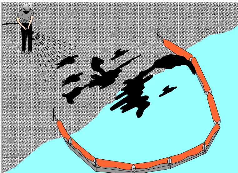
Figure 5 - 33 Low-pressure washing
