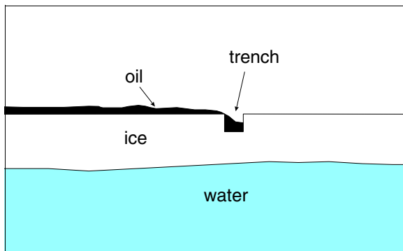
Figure 5 - 11 Ice trench
