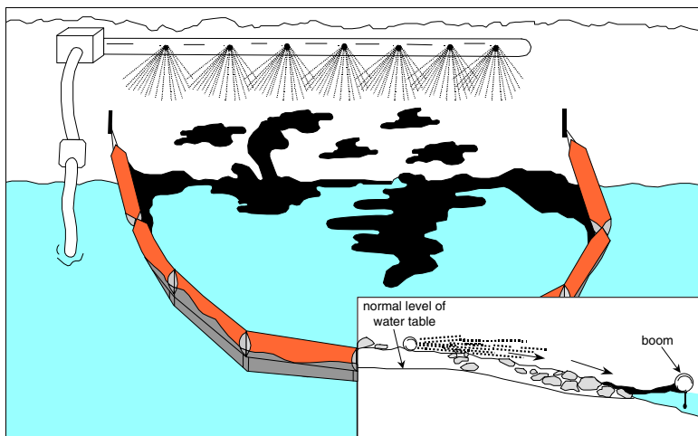
Figure 5 - 32 Flooding technique
