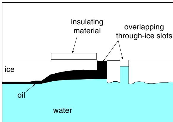
Figure 5 - 13 Ice slots
