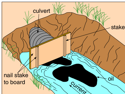
Figure 5 - 6 Culvert block
