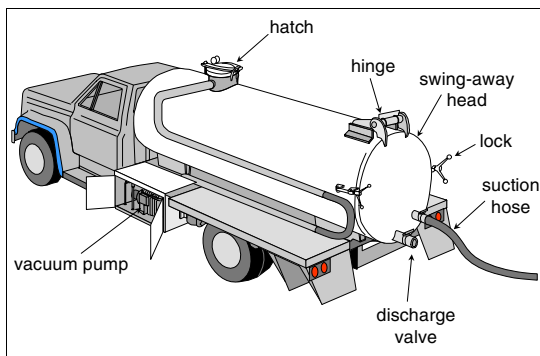
Figure 5 - 23 Vacuum truck
