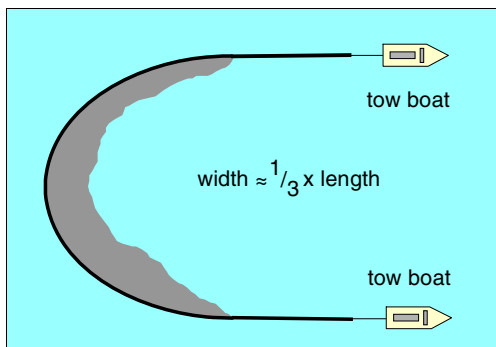
Figure 5 - 2 Catenary boom configuration
