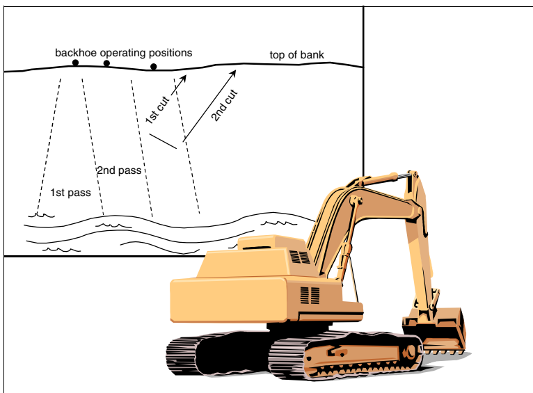
Figure 5 - 37 Direct mechanical removal with backhoe
