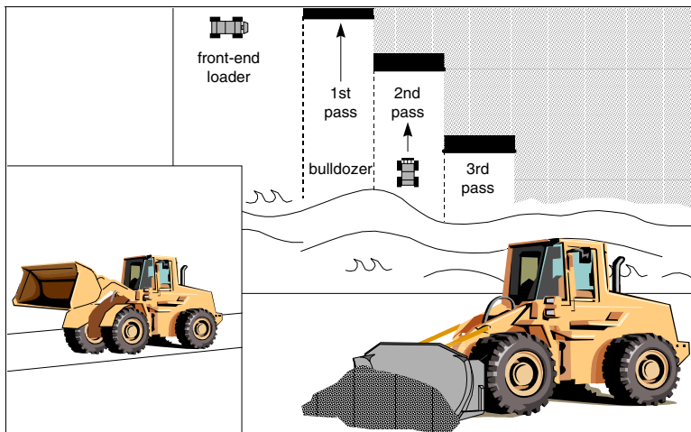
Figure 5 - 40 Two-stage removal with bulldozer supported by front-end loader
