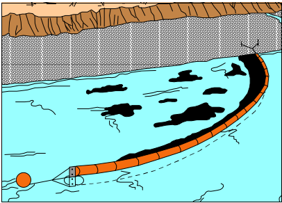
Figure 5 - 17 River booming
