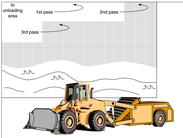
Figure 5 - 36 Direct mechanical removal with elevating scraper
