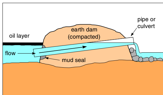
Figure 5 - 7 Inverted weir
