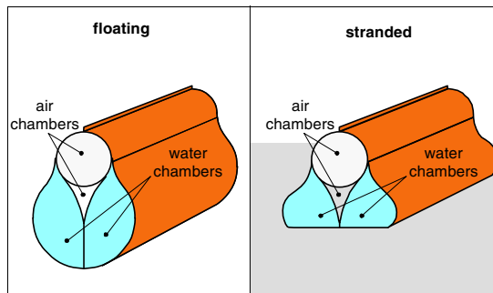
Figure 5 - 19 Boom design
