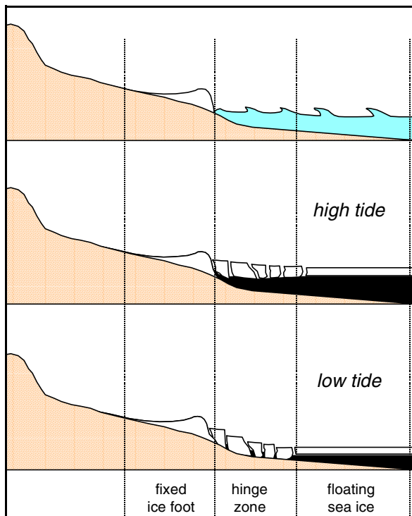
Figure 4 - 3 An ice-foot develops when waves or water freeze at the water line (top). In tidal areas, a zone of cracks separates the fixed ice foot from the nearshore floating ice (middle - at high tide, bottom - at low tide).
