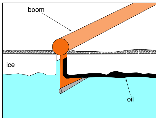
Figure 5 - 14 Boom/ice slot
