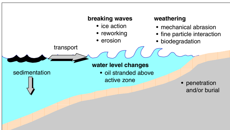
Figure 6 - 3 Oil stranding on shore
