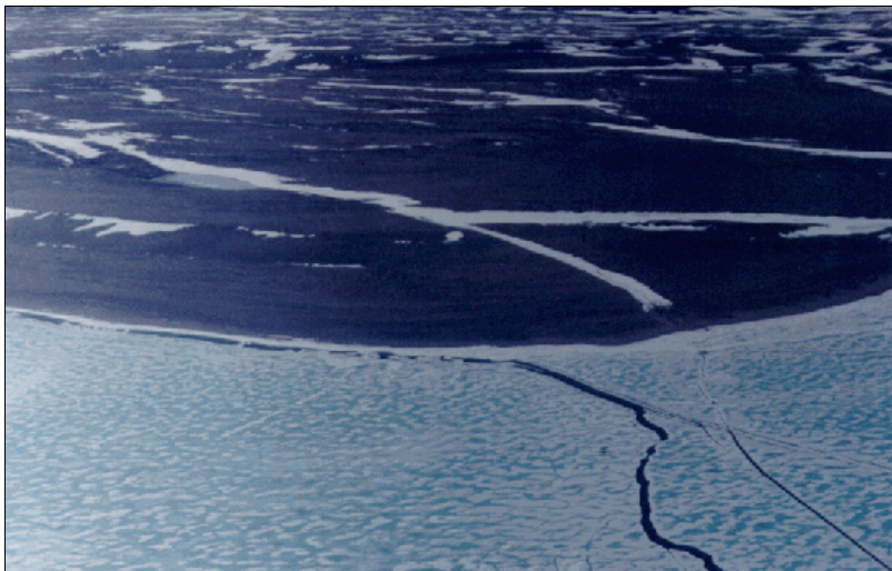
Figure 8 - 28 Leads that often develop in solid ice where pooled oil can be burned or skimmed
