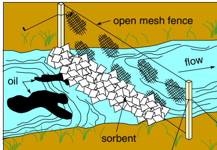
Figure 5 - 5 Filter fence
