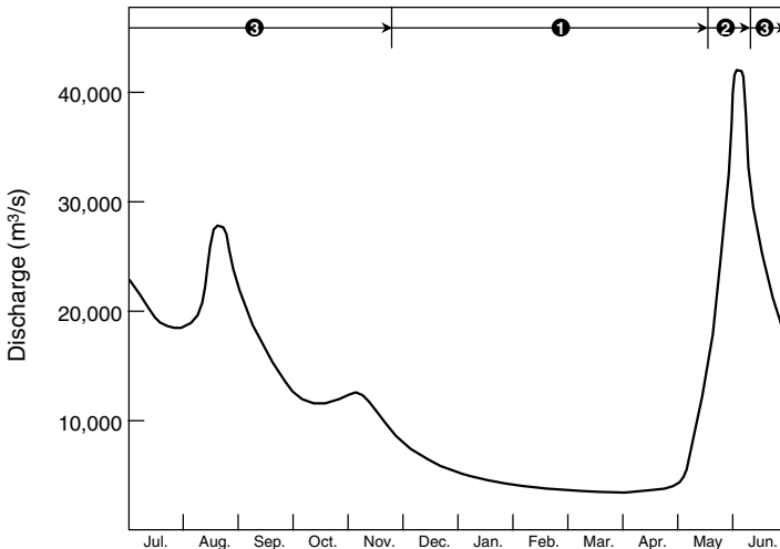
Figure 6 - 5 Typical seasonal variation in river discharge, Mackenzie River, Canada
