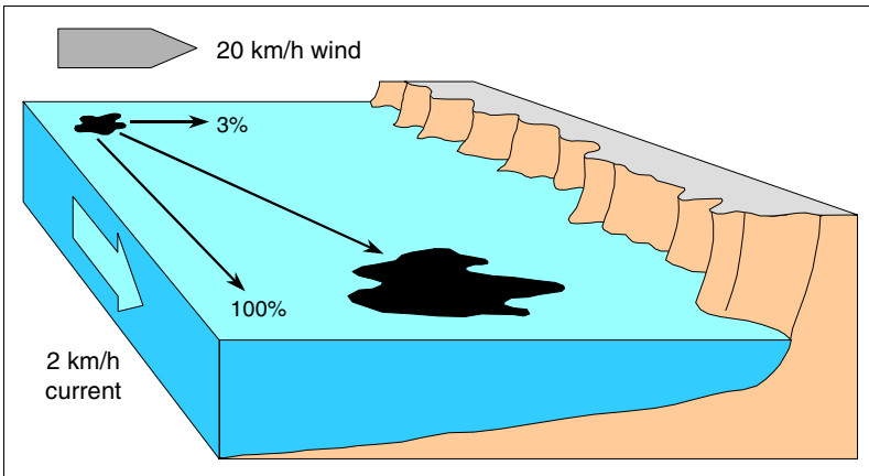
Figure 6 - 4 The movement of oil on water by wind and current (adapted from ITOPF, 1987)
