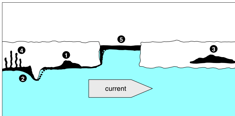
Figure 6 - 2 Oil in and under ice
