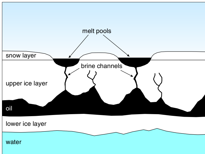
Figure 5 - 26 Melt pools
