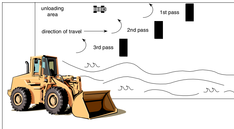
Figure 5 - 38 Direct mechanical removal with front-end loader
