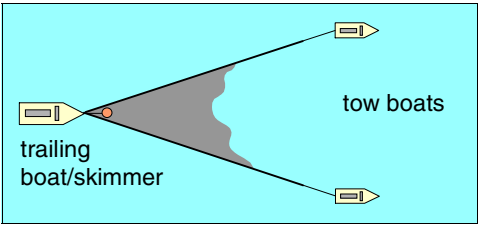
Figure 5 - 3 V-boom configuration
