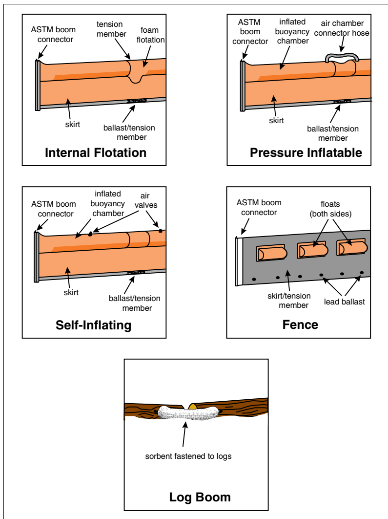
Figure 5 - 1 Mobile floating barrier types
