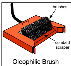
Figure 5 - 22 Stationary skimmer types
