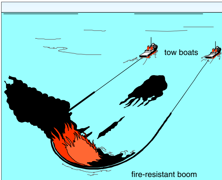
Figure 5 - 24 Open water containment/burning
