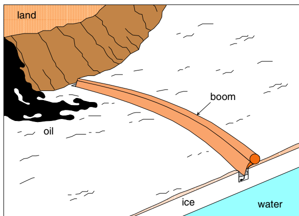
Figure 5 - 12 Boom/ice trench
