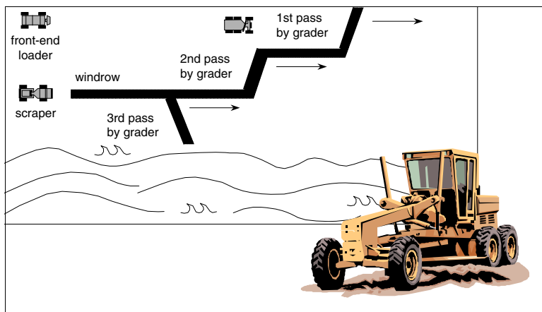
Figure 5 - 39 Two-stage removal with grader supported by loader and/or scraper
