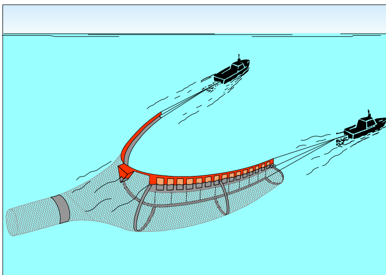
Figure 5 - 9 Oil trawl boom for surface and submerged oil
