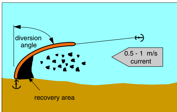
Figure 5 - 15 Diversion booming
