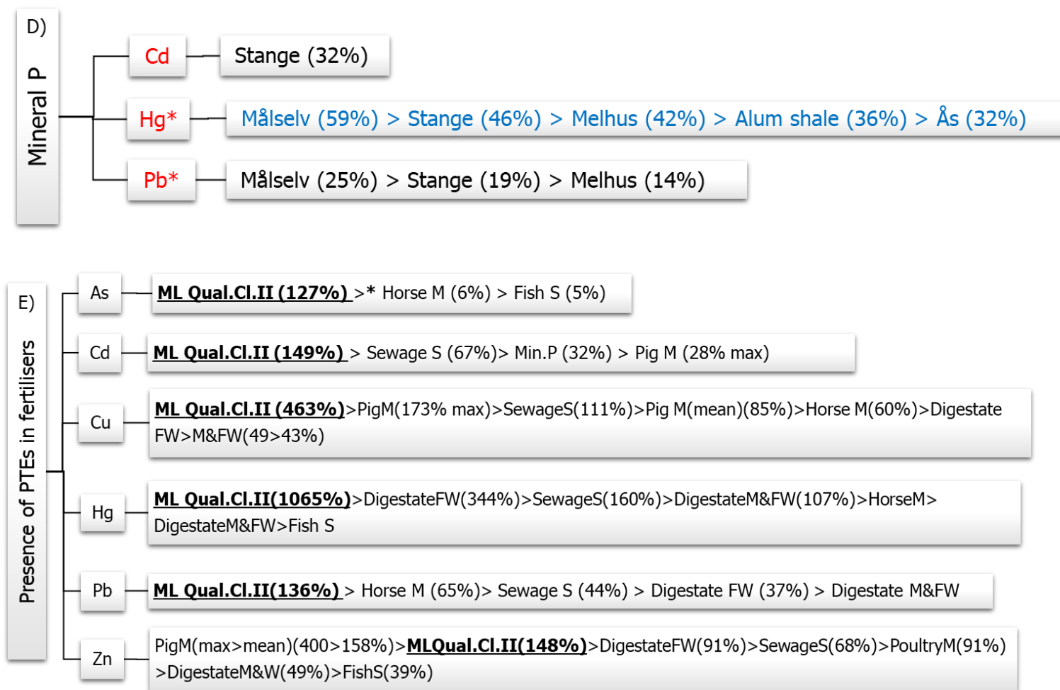
Figure 11.2-4. Estimated accumulation of PTEs in soil over 100 years, given as percent (%) from present soil concentration, after application of (A) fertiliser products according to Norwegian regulation of organic fertilisers, 2000 kg ha -1 yr -1 and MLs quality class II; (B) sewage sludge,
