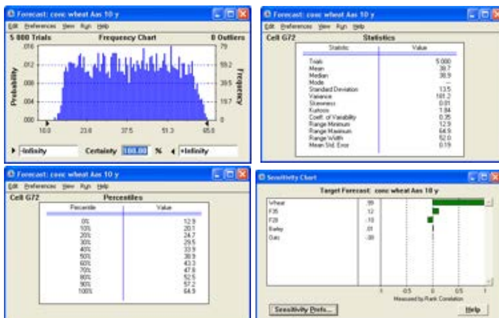
Figure AVIII-6 a,b,c,d. Forecast of concentration in wheat ( \mu\text{g/kg fw} ). a) Frequency distribution b) statistics c) percentiles d) sensitivity chart. F28 is precipitation, F35 is Kd; oats, wheat and barley are the transfer factors for these plants.
