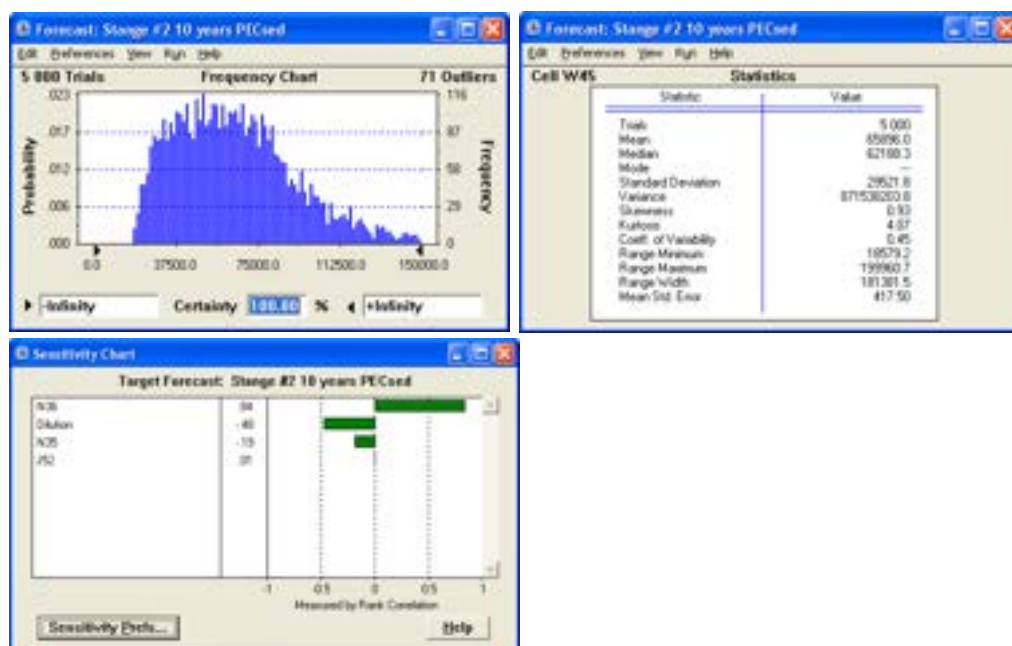
Figure AVIII-31 a,b,c,d. Forecast of PEC_{\text{sed}} for Cu, Stange, #2, 10 years. a) Frequency distribution b) statistics c) percentiles d) sensitivity chart, where N35 is Kp_{\text{susp}} , N36 is Kp_{\text{sed}} , J52 is E_{\text{tot}} (in Stange) and Dilution is dilution factor. Default value of PEC_{\text{sed}} Cu in Stange is 58177 \mu\text{g kg}^{-1} .
