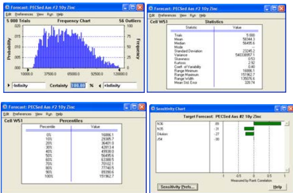
Figure AVIII-20 a,b,c,d. Forecast of PEC_{sed} for Zn, Ås, #2, 10 years. a) Frequency distribution b) statistics c) percentiles d) sensitivity chart, where N35 is Kp_{susp} , N36 is Kp_{sed} , J54 is E_{tot} (in Ås) and Dilution is dilution factor. Default value of PEC_{sed} 40803 \mu g\ kg^{-1} .
