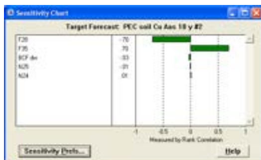
Figure AVIII-23 a,b,c,d. Forecast of PEC soil for Cu. a) Frequency distribution b) statistics c) percentiles d) sensitivity chart, where N25 is TF wheat, N24 is TF oats, BCF DW is TF barley, F28 is precipitation, F35 is Kd. Default PEC soil value Cu is 15.89 mg kg -1 DW.
