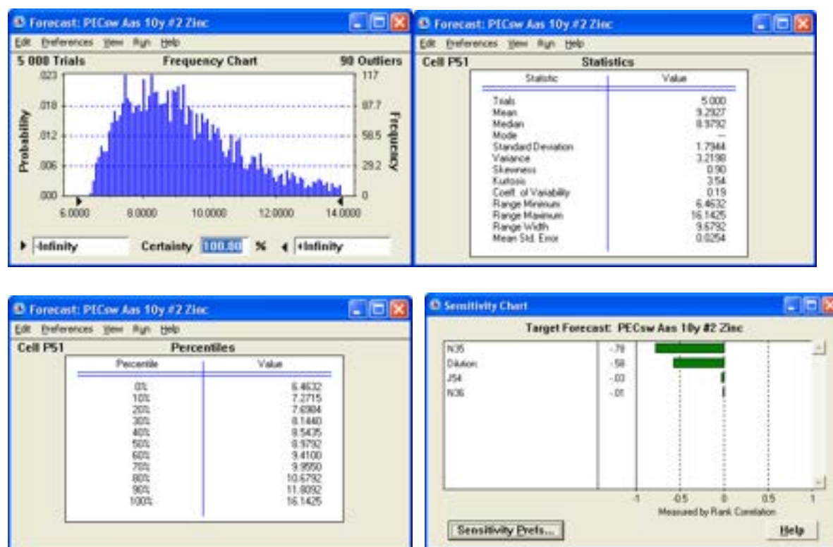
Figure AVIII-19 a,b,c,d. Forecast of PEC_{sw} for Zn, Ås, #2, 10 years. a) Frequency distribution b) statistics c) percentiles d) sensitivity chart, where N35 is Kp_{susp} , N36 is Kp_{sed} , J54 is E_{tot} (in Ås) and Dilution is dilution factor. Default value of PEC_{sw} is 8.14 \mu g L^{-1} .
