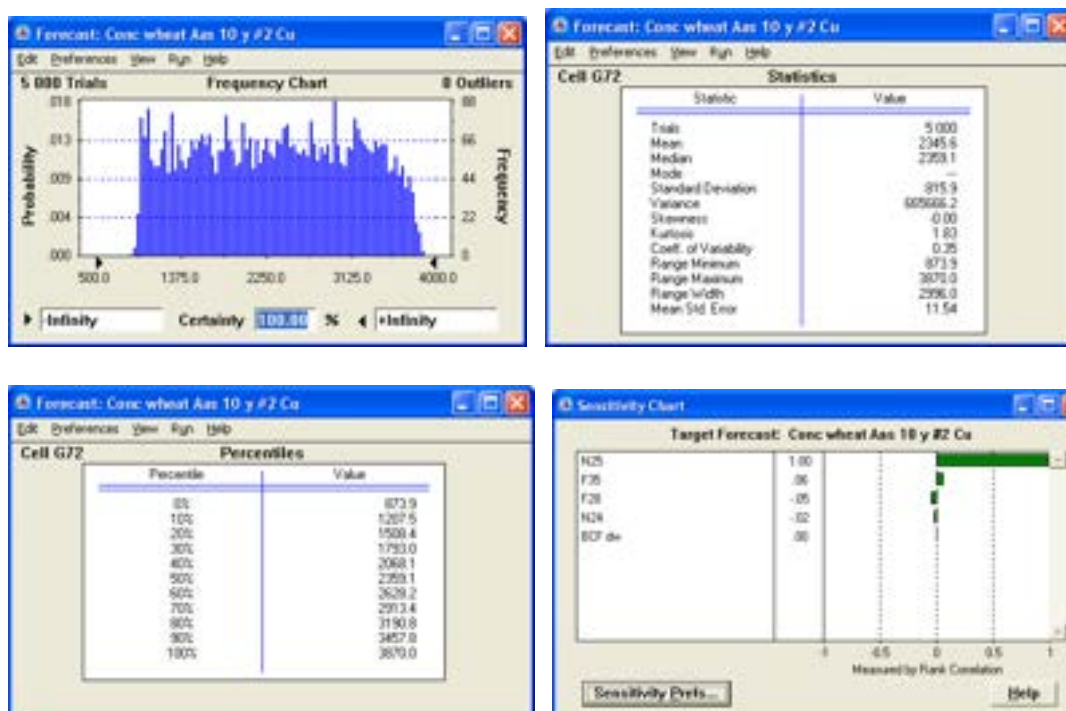
Figure AVIII-24 a,b,c,d. Forecast of Cu concentration in wheat (Zn \mu\text{g/kg fw} ). a) Frequency distribution b) statistics c) percentiles d) sensitivity chart, where N25 is TF wheat, N24 is TF oats, BCF DW is TF barley, F28 is precipitation, F35 is Kd. Default value: 1891 \mu\text{g/kg fw} .
