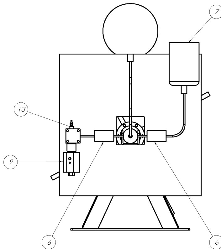
Figure 4.3 Complete system for conformal calibration, back-view.
