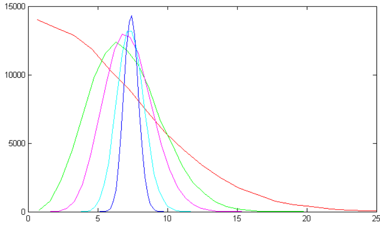
Figure C.3 Biased sample standard deviation distribution from an underlying normal distribution. Sample sizes are N = 2 (red), 5 (green), 10 (magenta), 30 (cyan) and 100 (blue).
