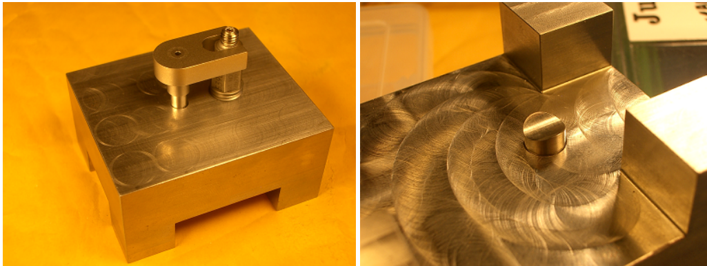
Figure 7.6 Device for measuring sensor seating depth change, top and bottom view.
