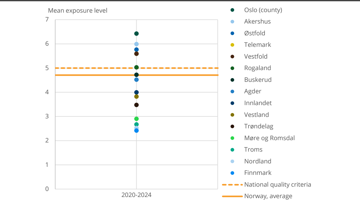
11.6.2. a) Annual mean levels of fine particulate matter PM2.5) in Norwegian regions, 2020-2024 (population weighted)
