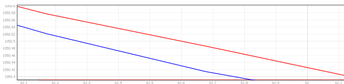
Figure 3.3.2-7: Selected part of elevation profile. Deviations of +/-2 cm along the transect. Red line: RTK georeferencing. Blue line: GCP georeferencing. x- and y-axis in meters.
