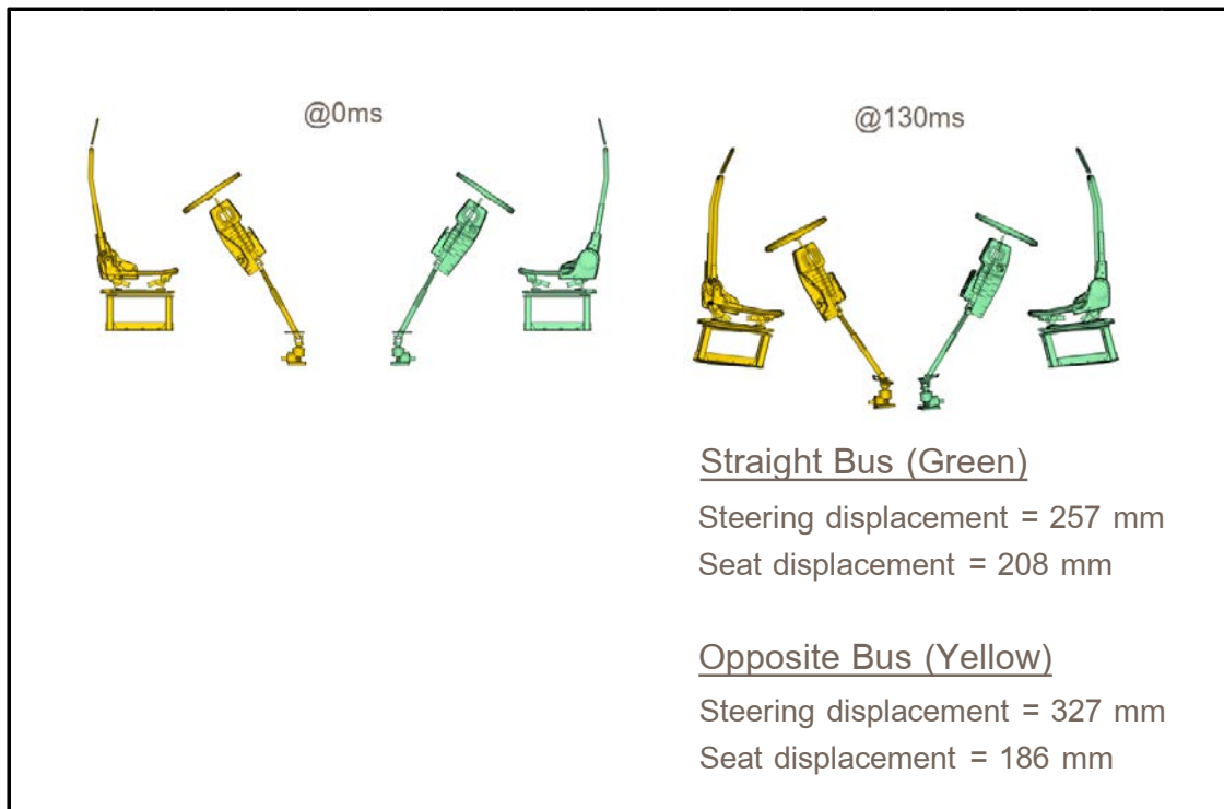
Figure 6.10: Illustration of steering column and seat displacement in an accident with frontal impact between 2 buses, with a 15% contact overlap, 0° angle orientation (straight), at 30 km/h, with Crash box.
