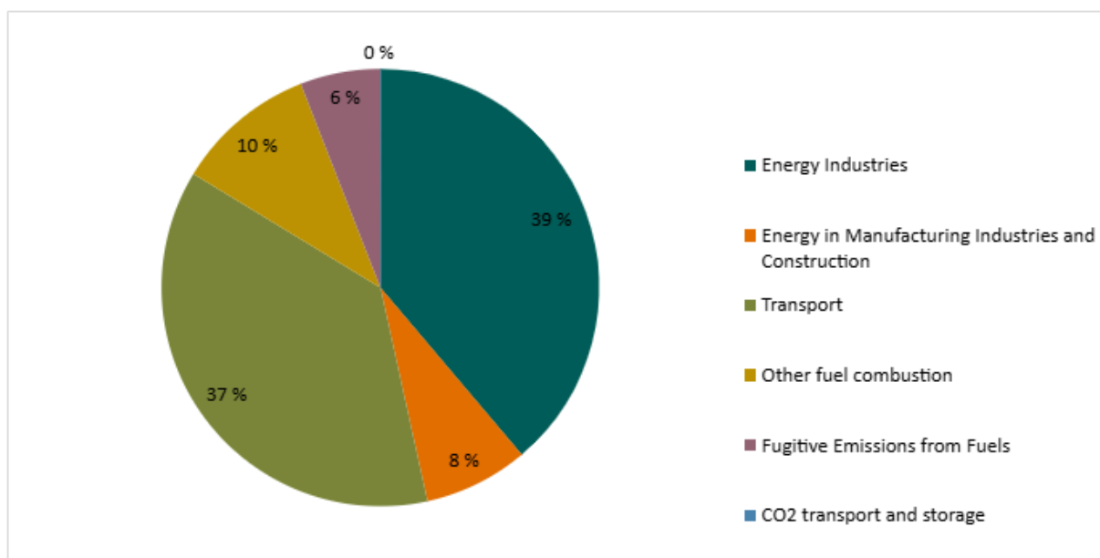
Figure 2.5: Greenhouse gas emissions in 2024 from the energy sector distributed among the different main source categories. Source: Statistics Norway/Norwegian Environment Agency.
