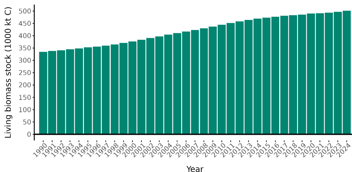
Figure 6.8: Development of the carbon stock in tree living biomass on forest land from 1990 to the latest reporting year. Source: Norwegian Institute of Bioeconomy Research.
