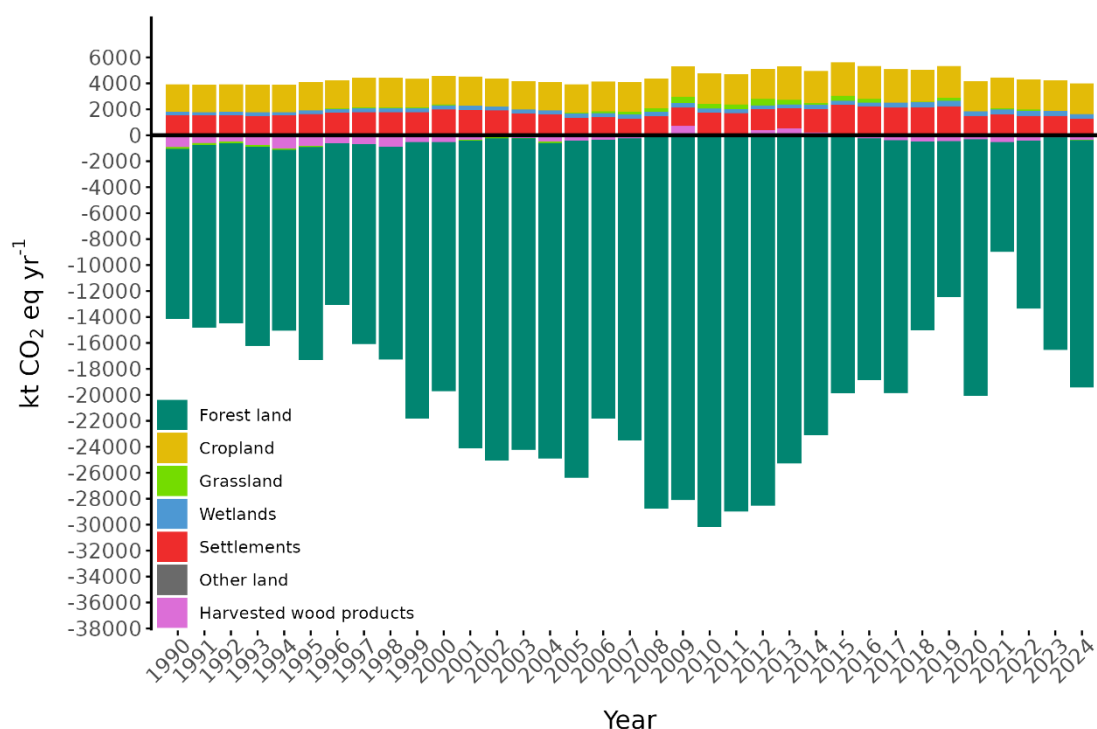
Figure 2.11: Net CO 2 emissions and removals (kt CO 2 equivalents per year) from the LULUCF sector by land-use category from 1990 to 2024, including emissions of N 2 O and CH 4 . Negative values are net removals, positive values are net emissions. Source: Norwegian Institute of Bioeconomy Research.
