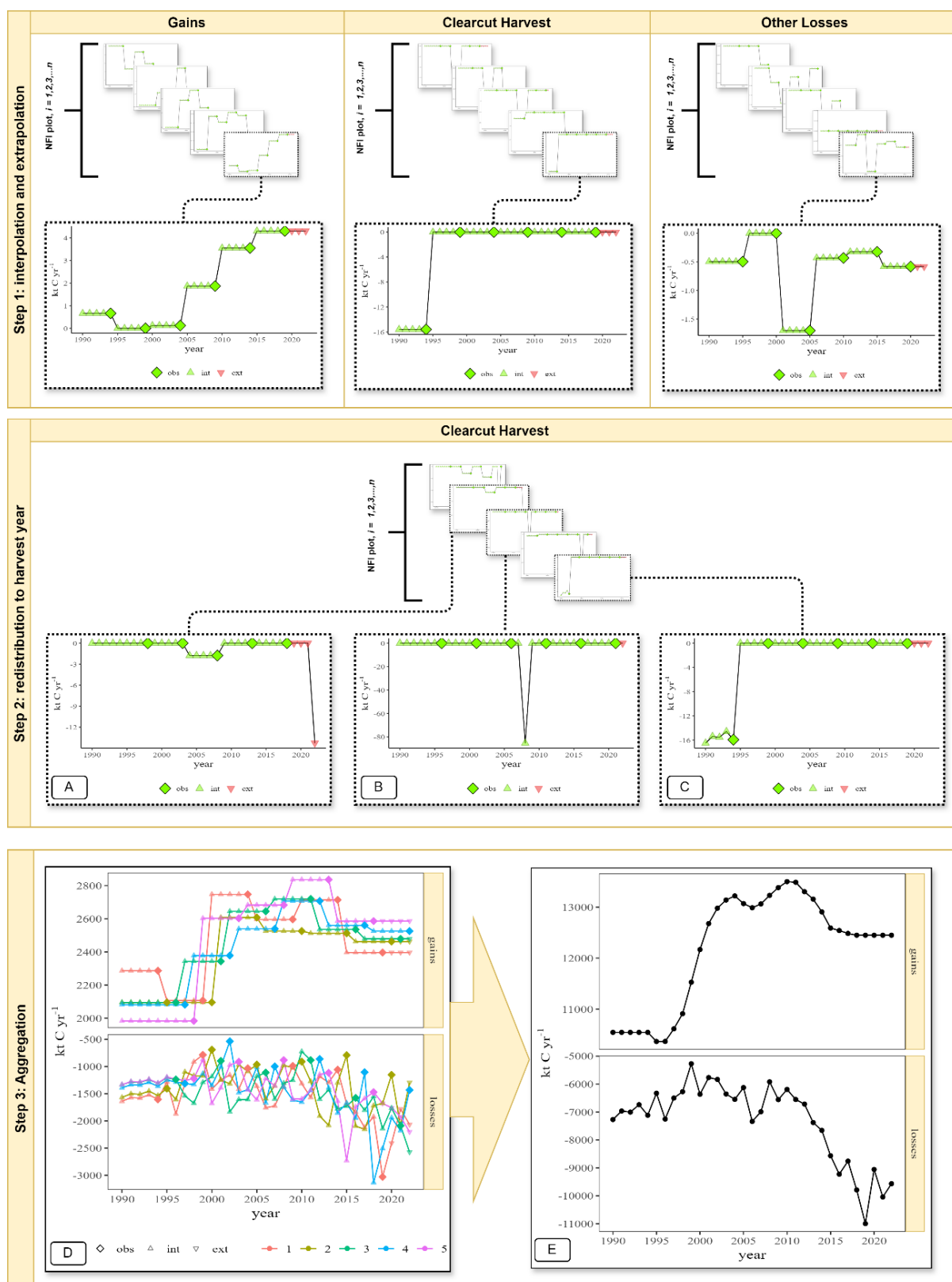
Figure 6.20: Workflow of interpolation-extrapolation processing steps. Step 1: linear interpolation (green triangles) is applied to observation (green diamonds) gains and losses for each NFI plot between each observation (green diamonds). Extrapolation (red upside-down triangle) is the average of the last 5 years (gains and other losses), except for plots with observed clear-cut harvest in the time series,
