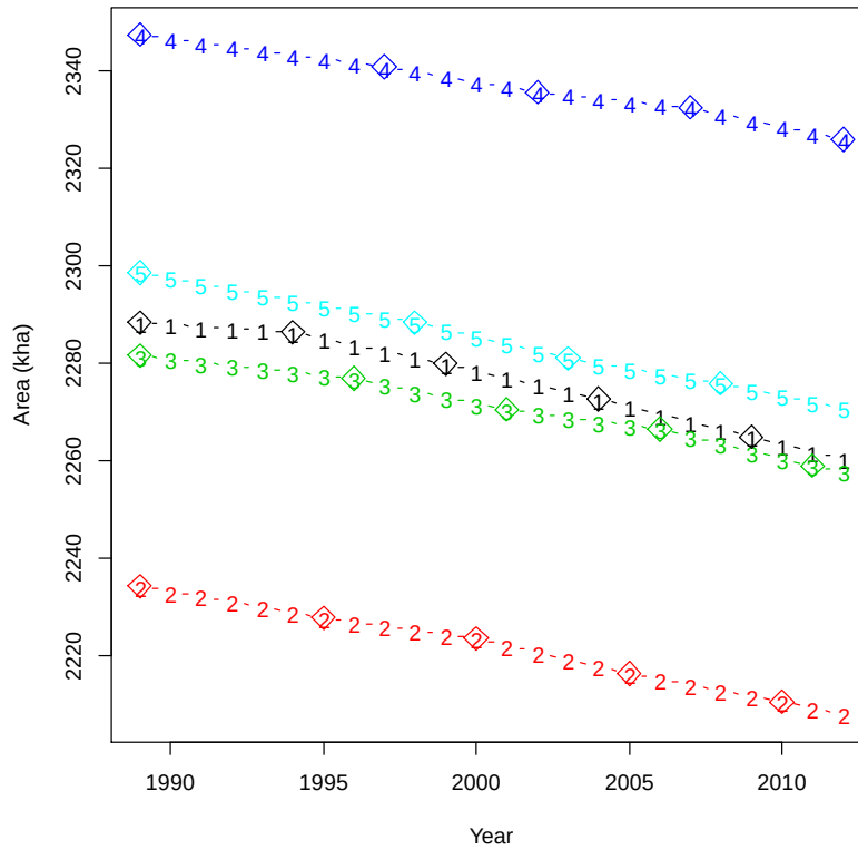
Figure 6.19: Estimated forest land remaining forest land area covering mineral soils within the five NFI panels, illustrated with data from 1989 until 2012. Diamonds indicate the measurement year of the sample plots in the respective panel (1 – 5). The estimated area was the sum of interpolated plots between two measurement years and extrapolated in the years after the last measurement year in each panel. Areas of land converted to forest land that will change their category to forest land remaining forest land after 2009, are not considered in the graphic.
