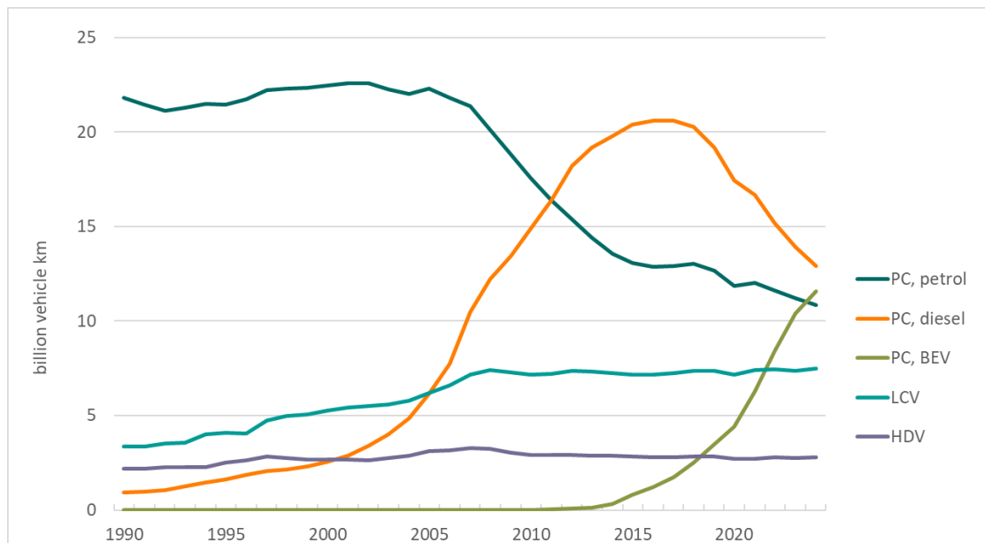
Figure 3.11: Vehicle kilometres. PC gasoline and diesel, LCV and HDV. BEV = Battery electric vehicles. Billion vehicle km. Source: Statistics Norway/Norwegian Environment Agency.
