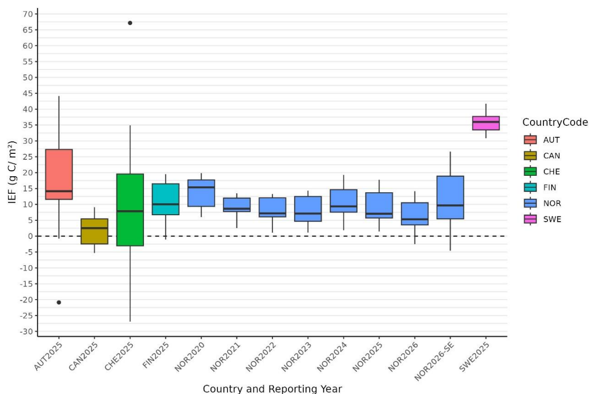
Figure.6.23: Boxplot of the sum of implied emission factors (IEF) 53 for dead wood, litter, and mineral soil for forest land remaining forest land from CRT tables for the countries Austria (AUT), Canada (CAN), Switzerland (CHE), Finland (FIN), Sweden (SWE), and Norway (NOR). Except for Sweden and Canada, all countries presented in the graph use the Yasso model (v07 or v20), either for dead wood, litter, and/or mineral soil CSC. Canada uses a carbon budget model, CBM-CFS3 (Kurz 2009), and Sweden uses soil and dead wood measurements. Each boxplot consists of IEF for all the years for a given reporting year (the number after the country abbreviation). For Norway reporting years 2020, 2021, 2022, 2023, 2024, 2025, and 2026 are presented for the whole country, and south-eastern Norway only for the year 2026.
