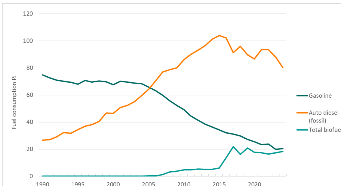
Figure 3.15: Consumption of gasoline, diesel and biofuel for road transportation. PJ. Source: Statistics Norway.
