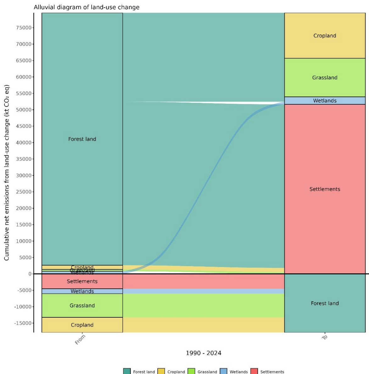
Figure 6.10: Distribution of cumulative net emissions and removals from land use transitions among IPCC land use categories from 1990 to the latest reporting year. Land-use changes with cumulative net emissions and removals less than 500 kt CO 2 equivalents are excluded from the figure as they are relatively small and not very visible. Source: Norwegian Institute of Bioeconomy Research.
