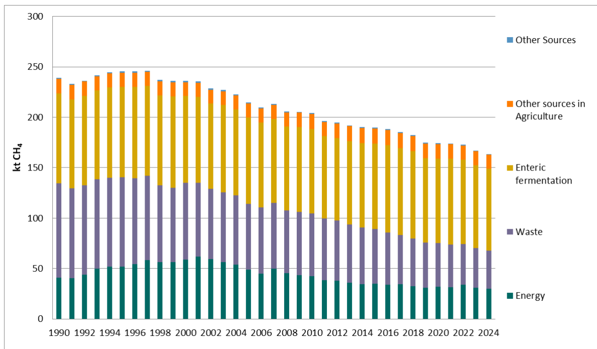
Figure 2.18: CH 4 emissions (ktonnes) in Norway, 1990-2024, without LULUCF. Source: Statistics Norway/Norwegian Environment Agency.
