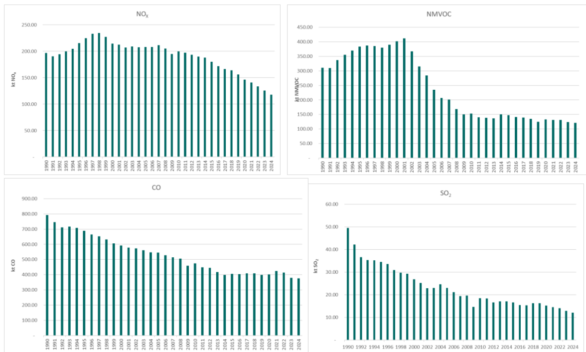
Figure 2.24: Emissions (ktonnes) of NO x , NMVOC, SO 2 , and CO in Norway, 1990-2024. Source: Statistics Norway/ Norwegian Environment Agency.
