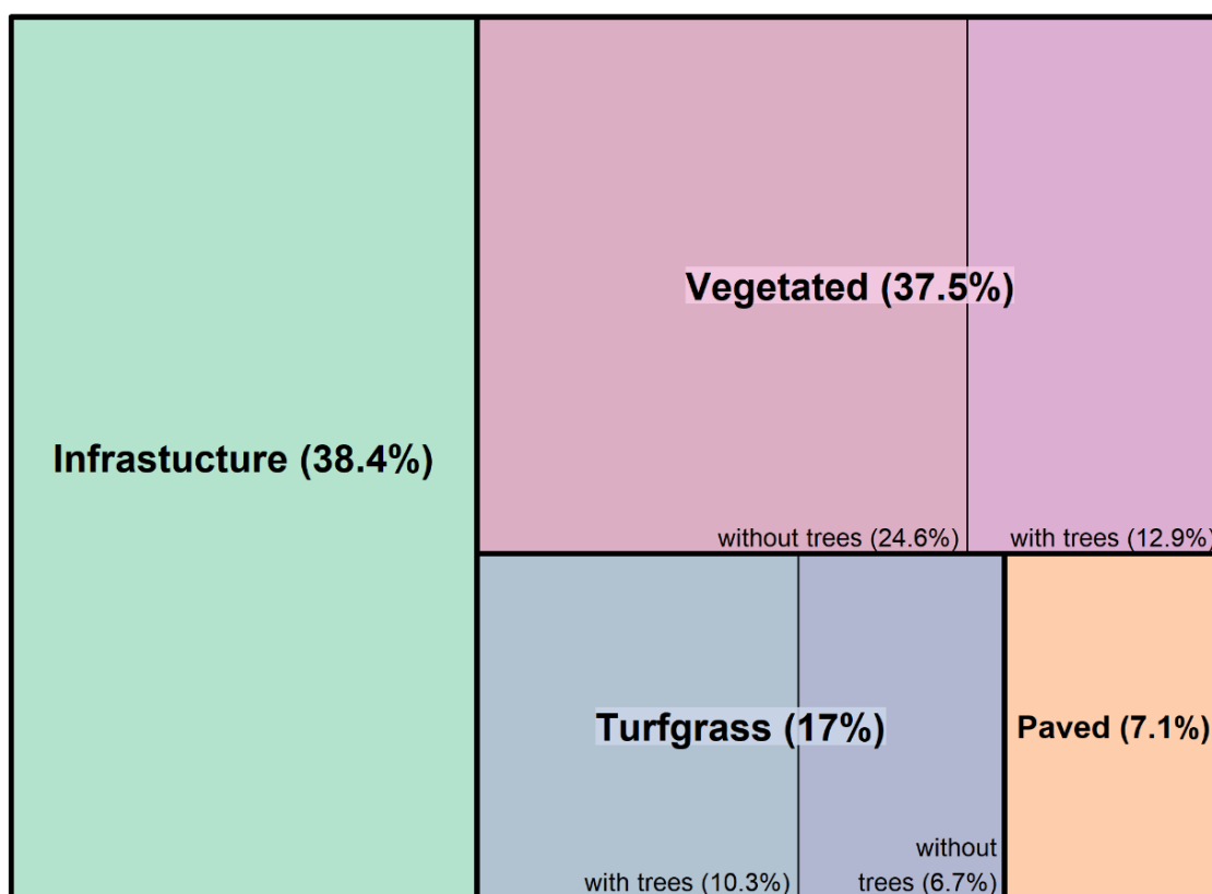
Figure 6.32: Settlement subcategory area distribution (2020 to the latest reporting year).
