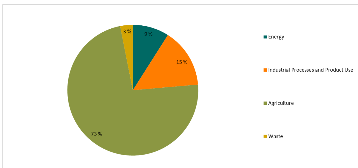
Figure 2.19: Distribution of Norwegian N 2 O emissions by major sources in 2024. Source: Statistics Norway/Norwegian Environment Agency.
