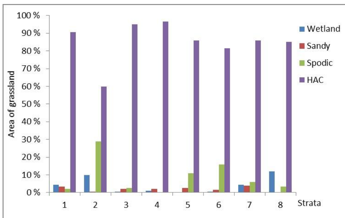
Figure 6.30: Distribution of soil types in intensive grassland areas for the eight strata. The IPCC soil types are high-activity clay soils (HAC): leptosols, fluvisol, phaeosem, albeluvisol, luvisol, umbrisol, cambisol, regosol; wetland soils: gleysols; sandy soils: arenosols; and spodic soils: podzol.
