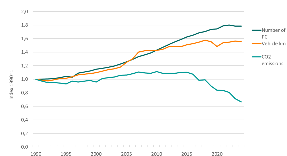
Figure 3.14: Relative change to 1990 in number of passenger cars, CO 2 emissions and vehicle kilometres. Index 1990=1. Source: Statistics Norway/Norwegian Environment Agency.
