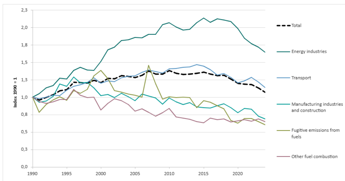
Figure 2.6: Development in emissions of greenhouse gases, relative to 1990, for the main sub-sectors within the energy sector, 1990-2024. Index 1990 = 1. Source: Statistics Norway/Norwegian Environment Agency.
