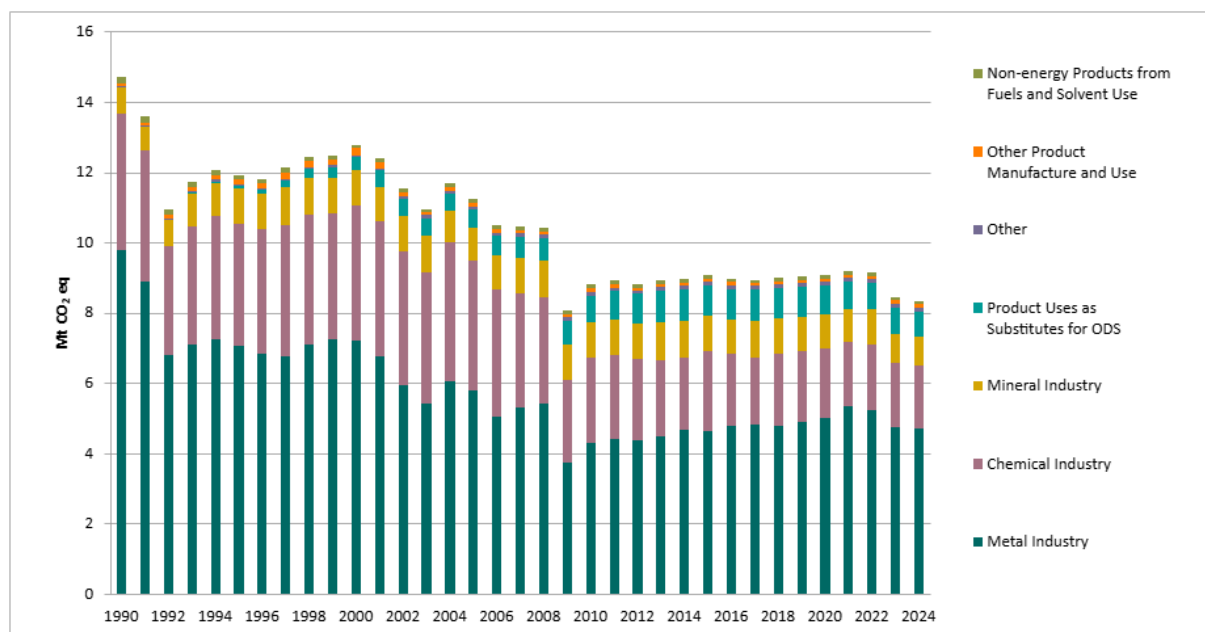
Figure 2.8: Total greenhouse gas emissions (Mtonnes CO 2 eq.) in the IPPU sub-sector in Norway, 1990-2024 11 . Source: Statistics Norway/Norwegian Environment Agency.
