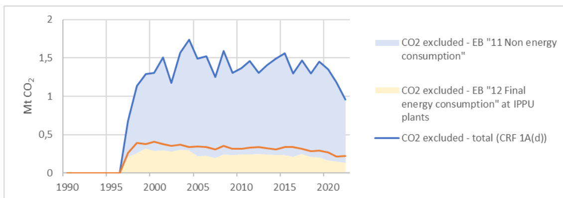
Figure 3.9: Natural gas . CO 2 amounts excluded from the reference approach (shaded areas, blue line) and reported as IPPU emissions (orange line). IPPU sectors reported in the inventory include:
