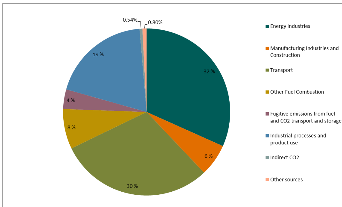
Figure 2.15: Distribution of CO 2 emissions in Norway by various source categories in 2024 (by mass). Source: Statistics Norway/Norwegian Environment Agency.
