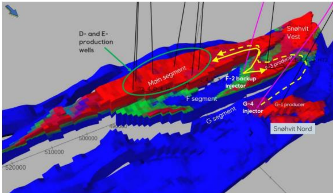
Figure 3.33: The reservoir simulation model shows how injected CO 2 is expected to move (indicated by yellow arrows) towards shallower areas and zones where the reservoir pressure has been reduced due to production of natural gas.
