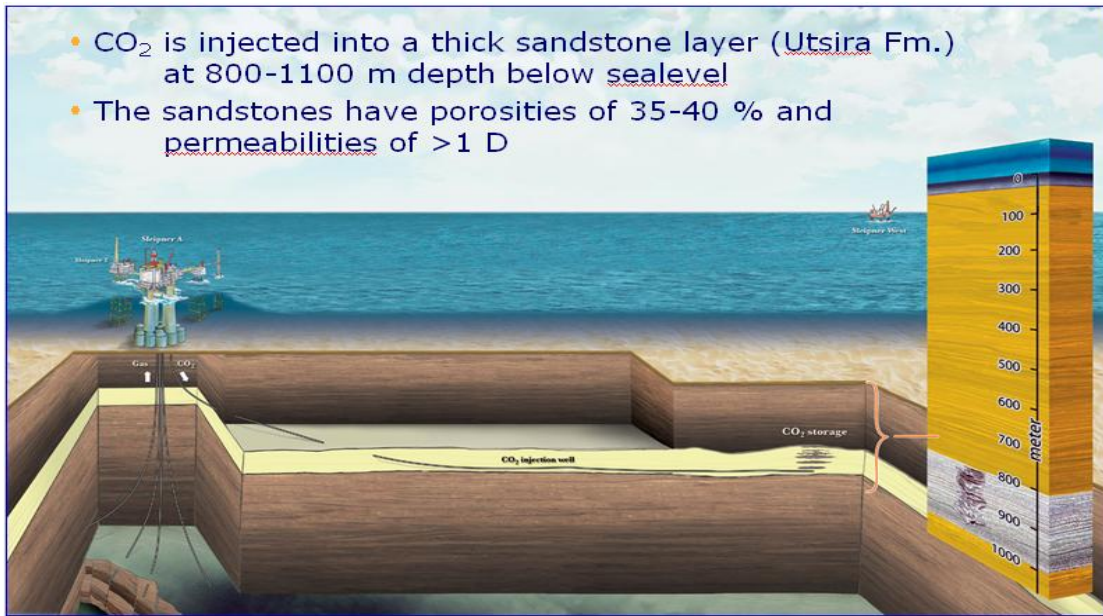
Figure 3.25: CO 2 capture from Sleipner Vest well stream and storage at Sleipner. Source: Equinor.
