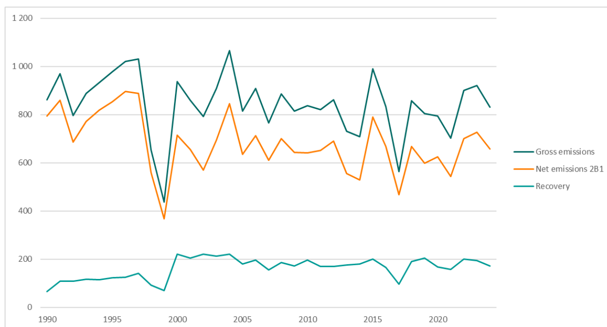
Figure 4.2: CO 2 emissions from production of ammonia. Source: Norwegian Environment Agency.
