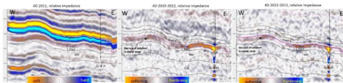
Figure 3.32: 4D relative impedance section from west to G-4 H in east for 2012, 4D difference 2019-2012 and 2022-2012. It is the upper parts of Stø2 Fm that take most of the injected CO 2 volumes in G-4 H.
