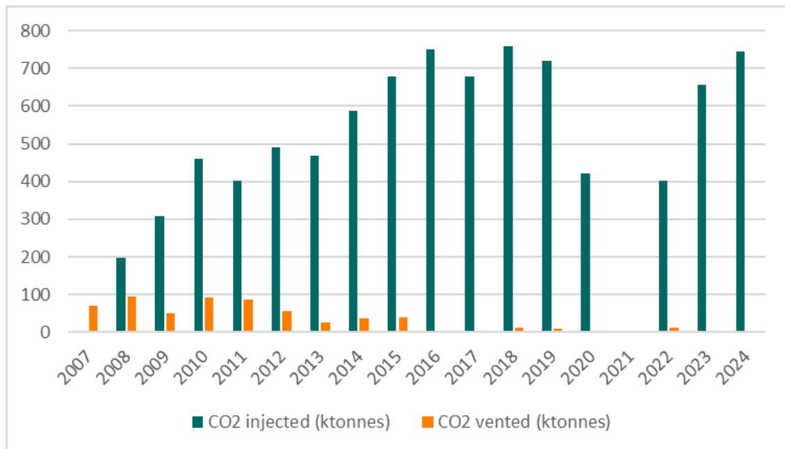
Figure 3.28: Injected and vented CO 2 at the Snøhvit field and Hammerfest LNG. Source: Equinor.
