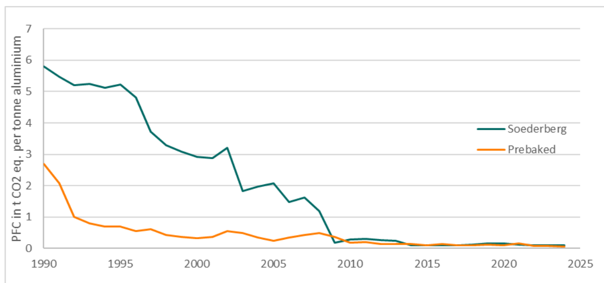
Figure 4.5: PFC in tonne CO 2 equivalent per tonne primary aluminium. Source: Norwegian Environment Agency.
