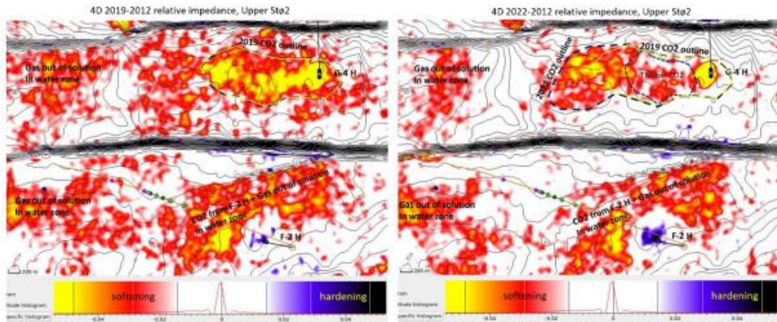
Figure 3.31: 4D relative acoustic impedance from 4D seismic inversion for 2019-2012 and 2022-2012 for upper parts of Stø2 Fm.
