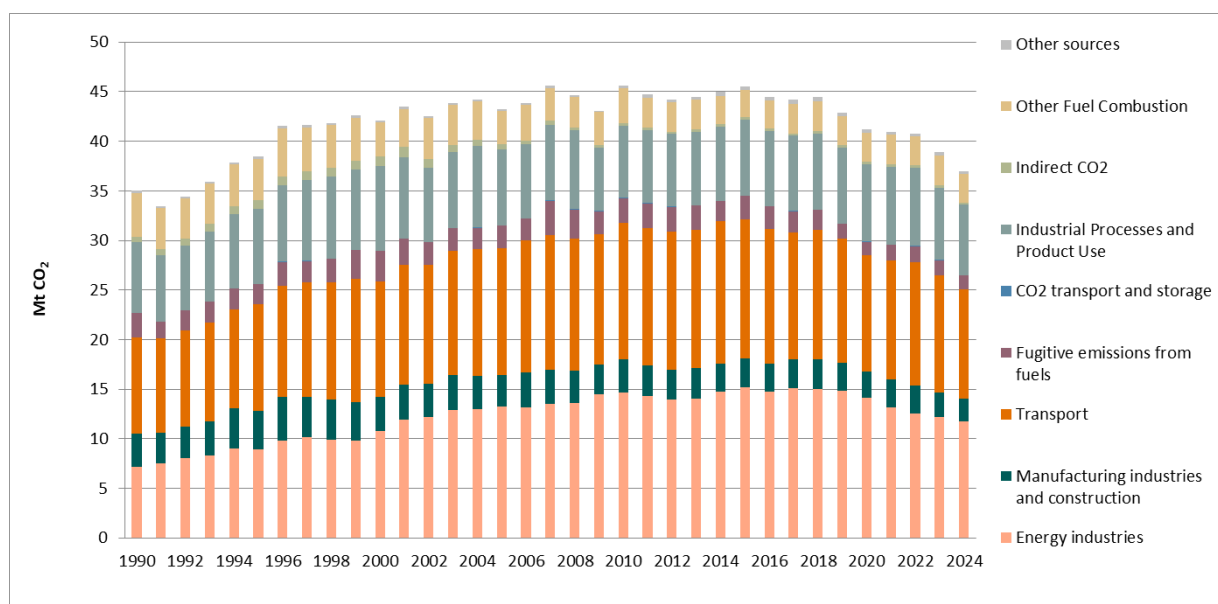
Figure 2.16: CO 2 emissions (Mtonnes) in Norway, 1990-2024. Source: Statistics Norway/Norwegian Environment Agency.
