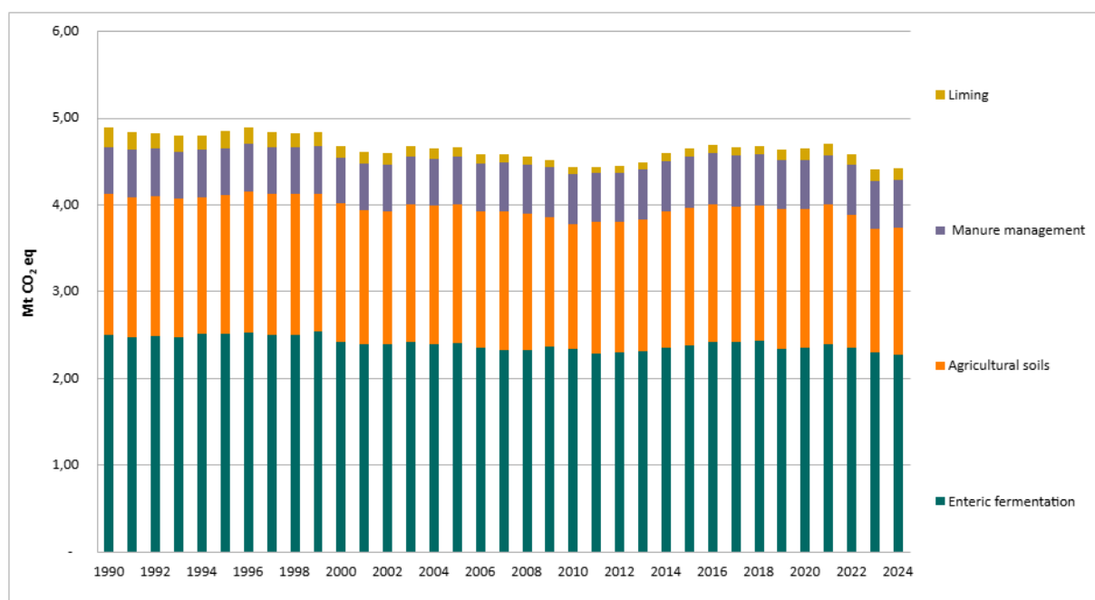
Figure 2.9: Total greenhouse gas emissions (Mtonnes CO 2 eq.) in the agriculture sub-sectors in Norway, 1990-2024. Source: Statistics Norway/Norwegian Environment Agency.
