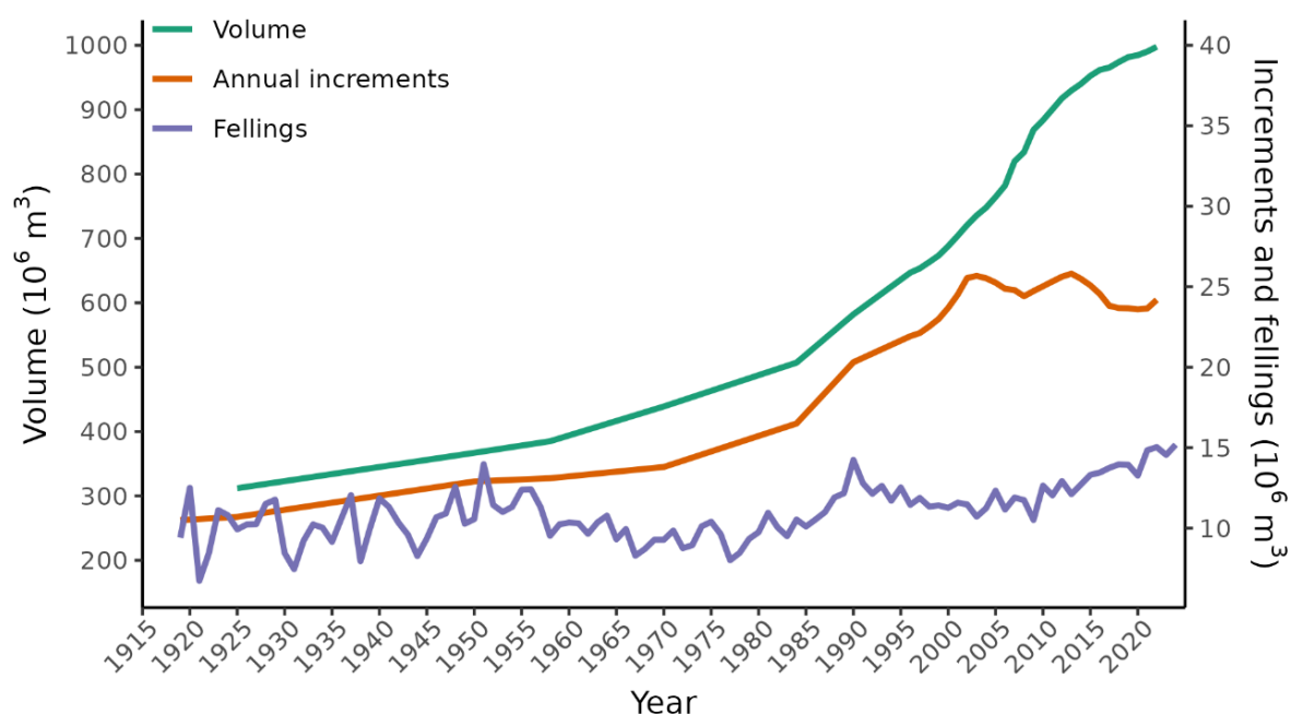
Figure 6.9: Forest felling, annual increments, and volume (without bark) from 1919 to the latest reporting year. Source: Norwegian Institute of Bioeconomy Research and Statistics Norway.
