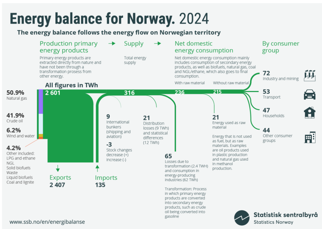
Figure 3.5: Energy balance for Norway.
