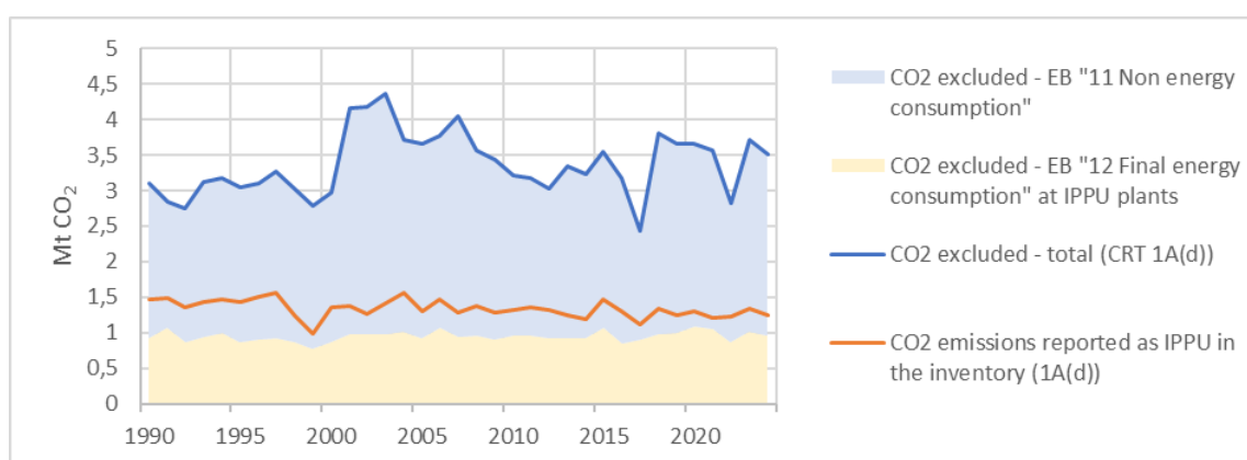
Figure 3.6: LPG. CO 2 amounts excluded from the reference approach (shaded areas, blue line) and reported as IPPU emissions (orange line). IPPU sectors reported in the inventory include:
