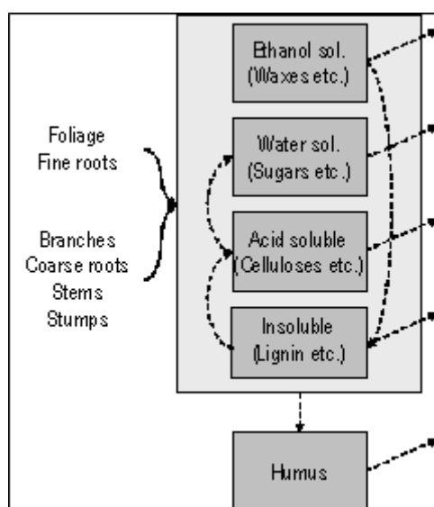
Figure 6.21: Flow diagram for chemical soil carbon pools in the Yasso model. Fluxes significantly different from 0 are indicated by the arrows (Liski et al. 2009).
