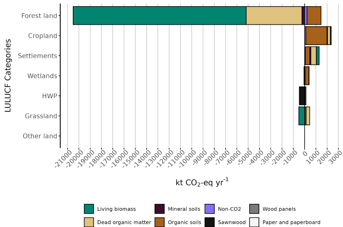
Figure 6.7: Net CO 2 emissions and removals (kt CO 2 equivalents per year) by land-use category (forest land, cropland, grassland, wetlands, settlements, other land, and harvested wood products) for the latest reporting year, including emissions of N 2 O and CH 4 . Negative values are net removals, and positive values are net emissions. Land-use categories are ordered from highest to lowest impact on the LULUCF sector. Source: Norwegian Institute of Bioeconomy Research.
