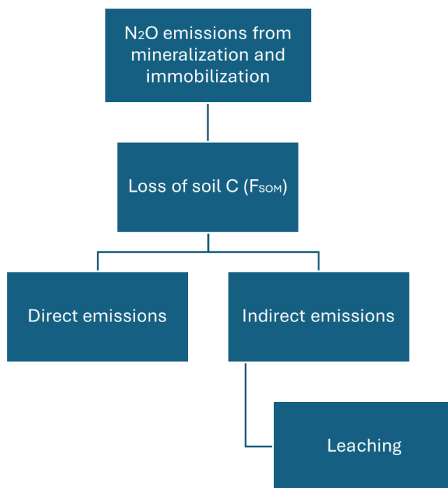
Figure 6.36: Reporting structure for Direct and Indirect N 2 O emissions from nitrogen mineralization and immobilization.
