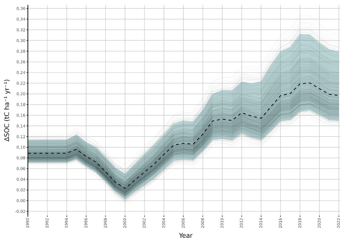
Figure 6.22: Uncertainty for CSC for SOC-derived Monte Carlo simulations ( n = 1\,000 , faint grey lines). The cyan band indicates the 95% confidence interval derived for each year from the 2.5 th and 97.5 th percentiles of the 1 000 simulations. The dashed line indicates the mean of the 1 000 simulations. Due to technical challenges with Yasso20, uncertainty estimates are still based on estimates from 2024 with the Yasso07 model.
