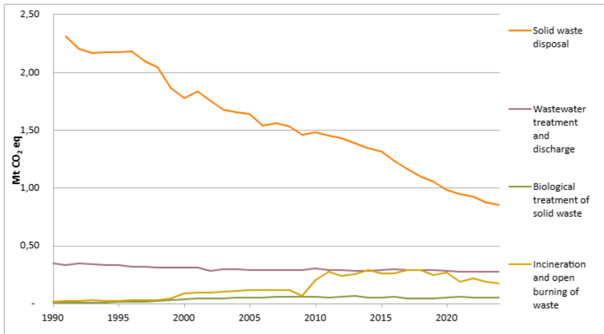
Figure 2.12: Total emissions of greenhouse gases (Mtonnes CO 2 eq.) in Norway from the waste categories, 1990-2024. Source: Statistics Norway/Norwegian Environment Agency.
