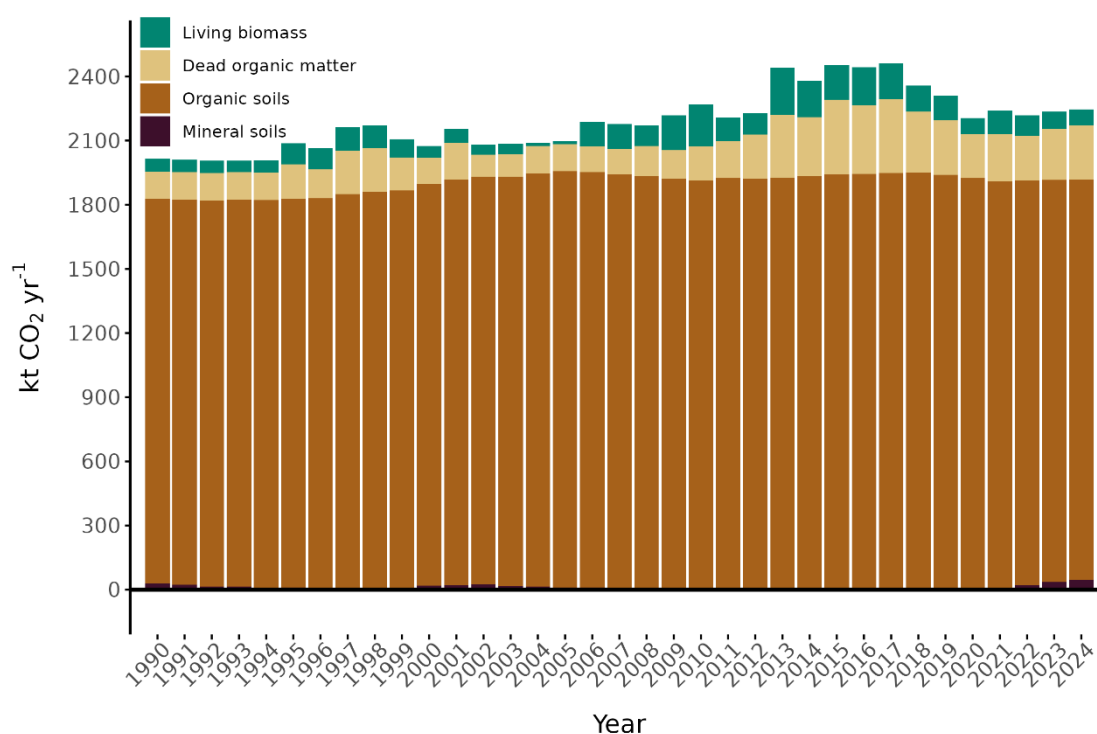
Figure 6.3: Net emissions and removals of CO 2 on cropland, including both remaining and land converted to cropland. The graph shows the aggregated net emissions and removals for both categories. Carbon pools can either act as a source or sink of CO 2 , depending on the category, although this might not always be visible in the graph. Non-CO 2 emissions and removals are not included in the graph. Source: Norwegian Institute of Bioeconomy Research.
