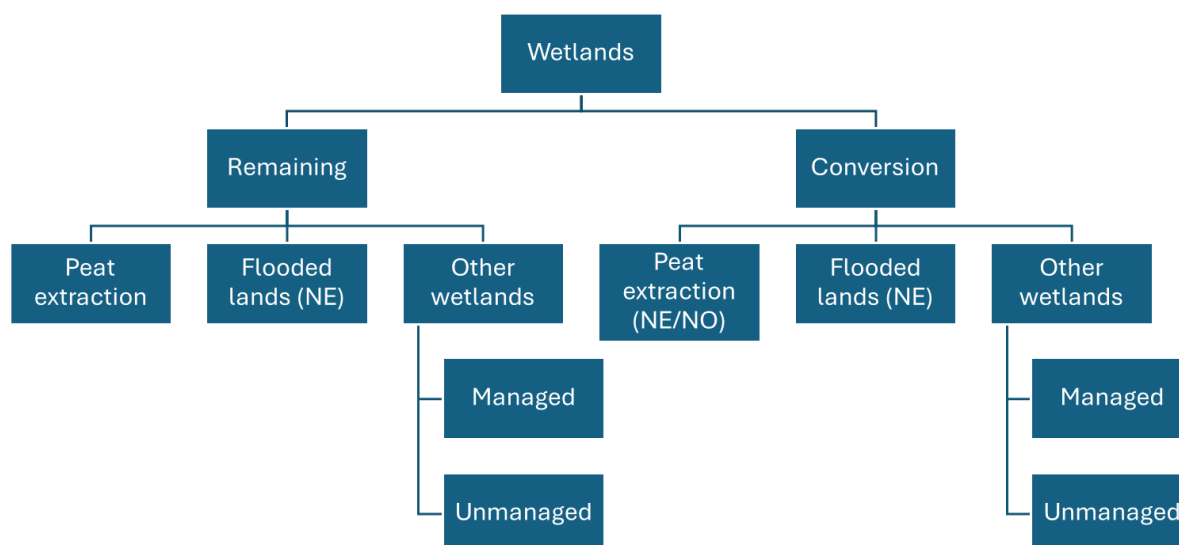
Figure 6.31: Reporting structure under Wetlands. The notation key NE “not estimated” is used for flooded land, as reporting is not mandatory for this category. The notation key NO means “not occurring”, which is the case of peat extraction in mineral soils.
