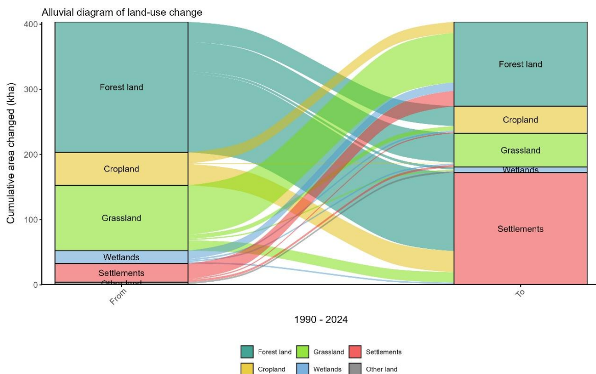
Figure 6.12: Distribution of cumulative area for land use transitions among all IPCC land use categories from 1990 to the latest reporting year. Source: Norwegian Institute of Bioeconomy Research.
