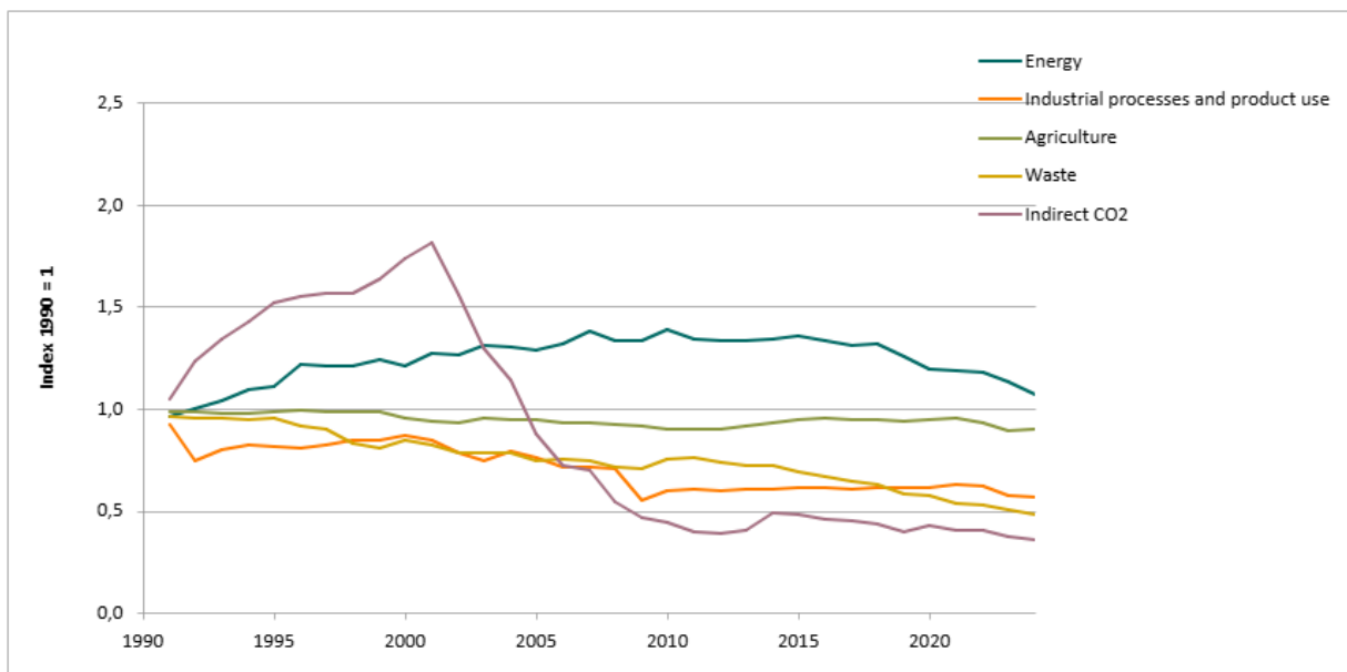
Figure ES.3: Changes in GHG emissions, relative to 1990, by IPCC sector 1990-2024. Index 1990 = 1. Source: Statistics Norway/Norwegian Environment Agency.
