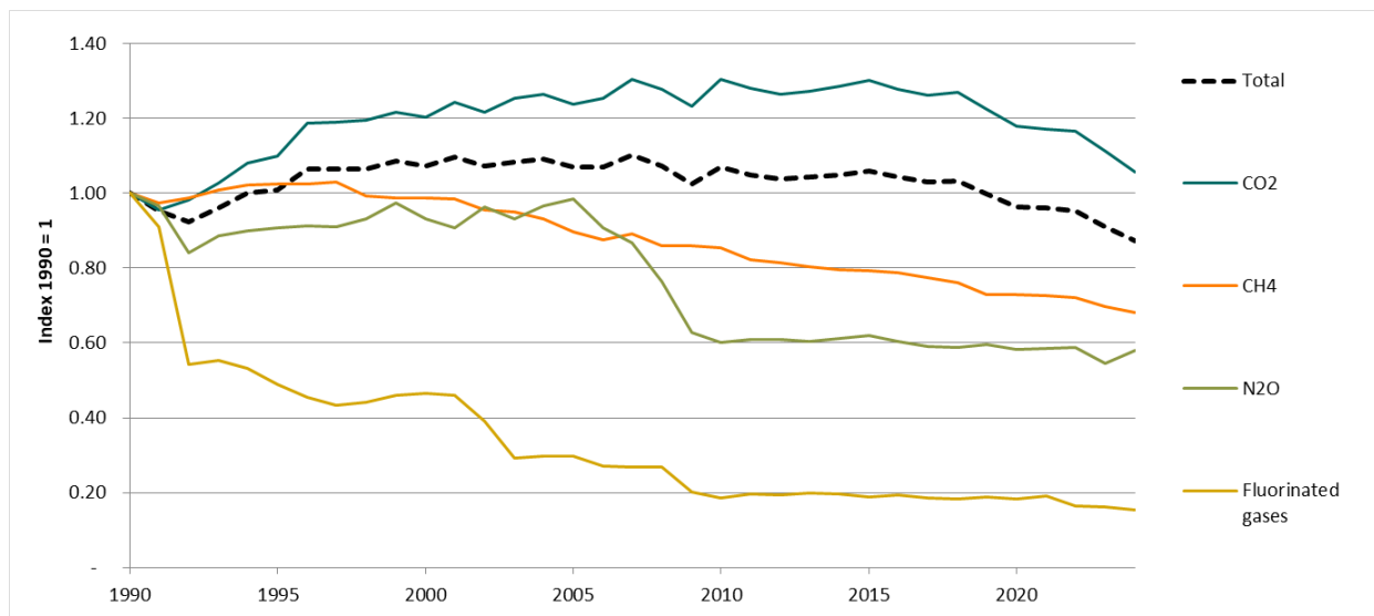
Figure 2.14: Changes in emissions of greenhouse gases, relative to 1990, by gas, 1990-2024. 'CO 2 ' and 'Total' includes indirect CO 2 . Index 1990 = 1. Source: Statistics Norway/Norwegian Environment Agency.
