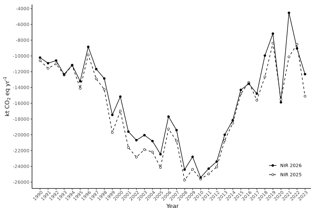
Figure 10.2: Recalculations illustrated for total emissions (kt CO 2 equivalents per year) estimated for the LULUCF sector in the latest submission compared to the previous submission
