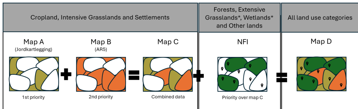
Figure 6.16: Hierarchical approach used to determine soil type in Norway. White areas represent land-use categories not covered by the respective maps. Pin symbols indicate plot locations. *Only wooded areas within these two land-use categories are surveyed by the NFI.
