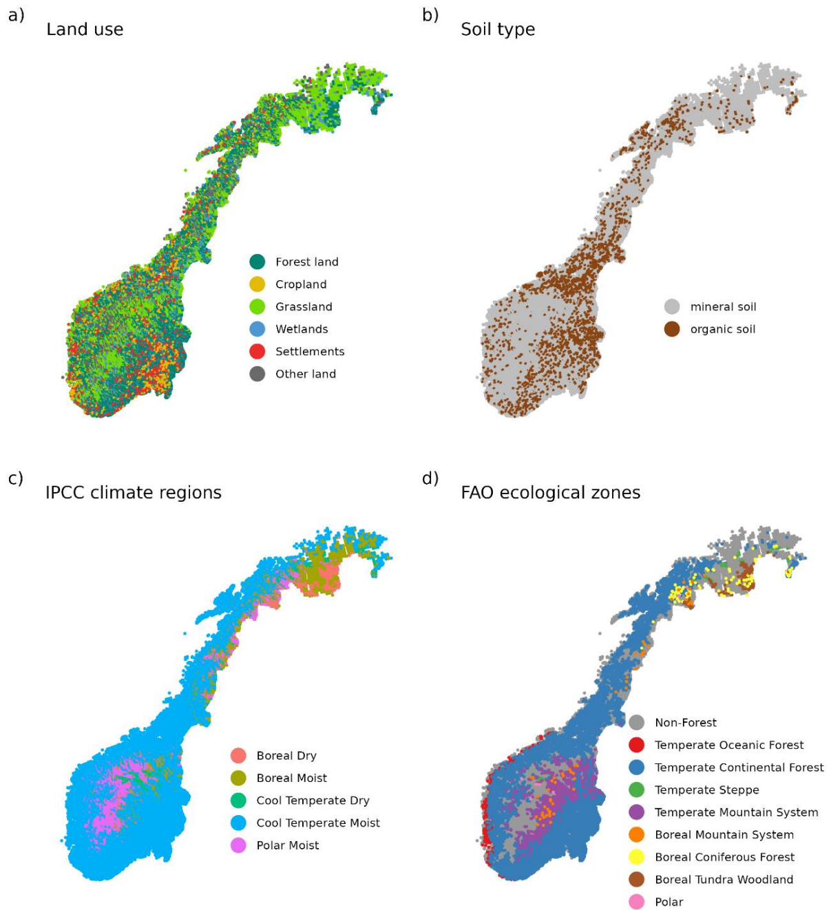
Figure 6.18: Map overview of NFI plot stratification: a) Current Land use categories; b) soil types; c) IPCC climate regions; d) FAO ecological zones for forest lands. The visual representation of each plot on the maps is altered to ensure the visibility of all categories, as the plotting order affects the visibility.
