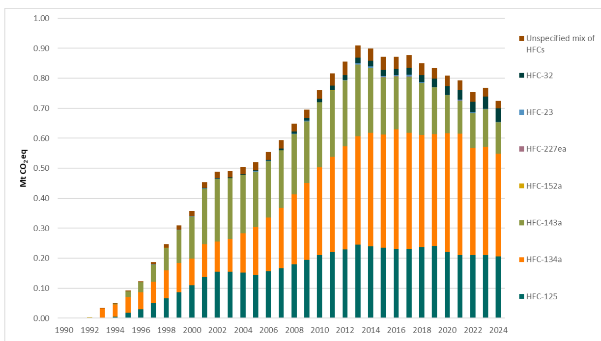
Figure 2.23: Emissions of HFCs (Mtonnes CO 2 eq.) in Norway, 1990-2024. Source: Statistics Norway/Norwegian Environment Agency.
