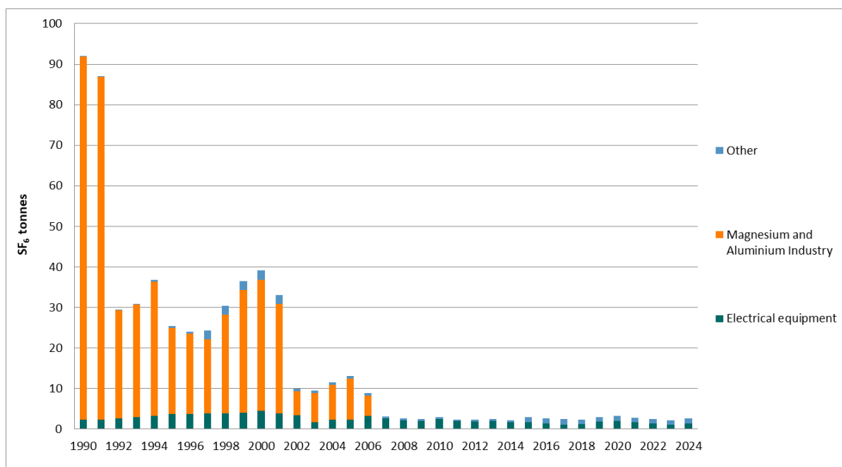
2.22: Emissions of SF 6 (tonnes) in Norway 1990-2024. Source: Statistics Norway/Norwegian Environment Agency.
