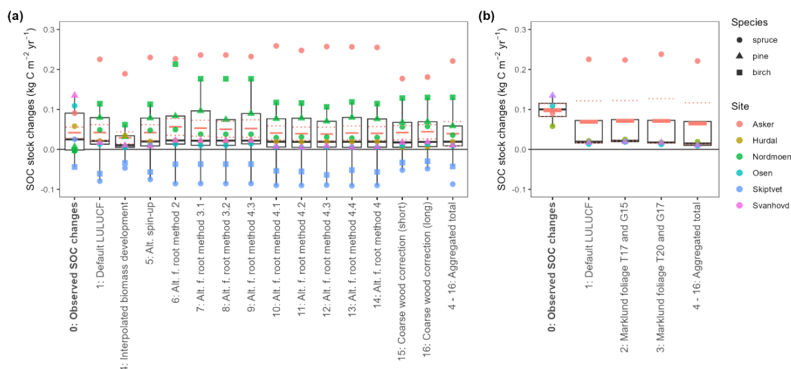
Figure 6.27: Boxplot of soil organic carbon (SOC) stock change for all sites grouped by observations, simulations (no. 1-16), and the aggregated total of simulations 4-16. Simulated SOC CSC are based on the Yasso20 model of SOC dynamics, while implementing (15) different methodologies for computing model input. The black and red lines in the boxplot indicate the median (50th percentile) and mean of estimates from plots across all sites, respectively. Each box represents the interquartile range of the data, spanning from the 25th percentile (Q1) to the 75th percentile (Q3). The lower and upper whiskers extend to the smallest and largest values within 1.5 times the interquartile range from Q1 and Q3, respectively. Data points beyond this range are considered outliers. The horizontal broken red lines in the boxes indicate \pm one standard error of the mean (SEM). Each plot is represented as a point on top of each boxplot, with color grouped for each site, and shape for the dominant tree species. Boxplots for simulations 2 and 3 only include data for Asker, Hurdal, Osen, and Svanhovd, and are therefore separated out in plot (b) together with observations and the default simulation. The remaining simulations are found in plot (a) together with the observations and the default simulation.
