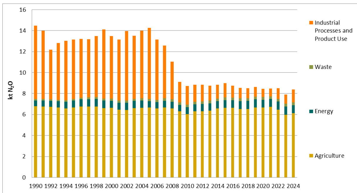
Figure 2.20: N 2 O emissions in Norway, 1990-2024, without LULUCF. Source: Statistics Norway/Norwegian Environment Agency.
