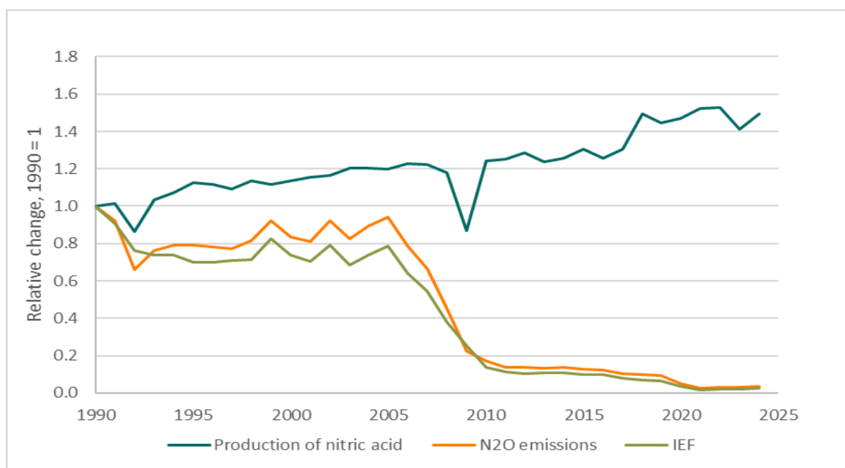
Figure 4.4: Relative change in total emissions, total production and IEF for nitric acid production. 1990=1. Source: Norwegian Environment Agency.
