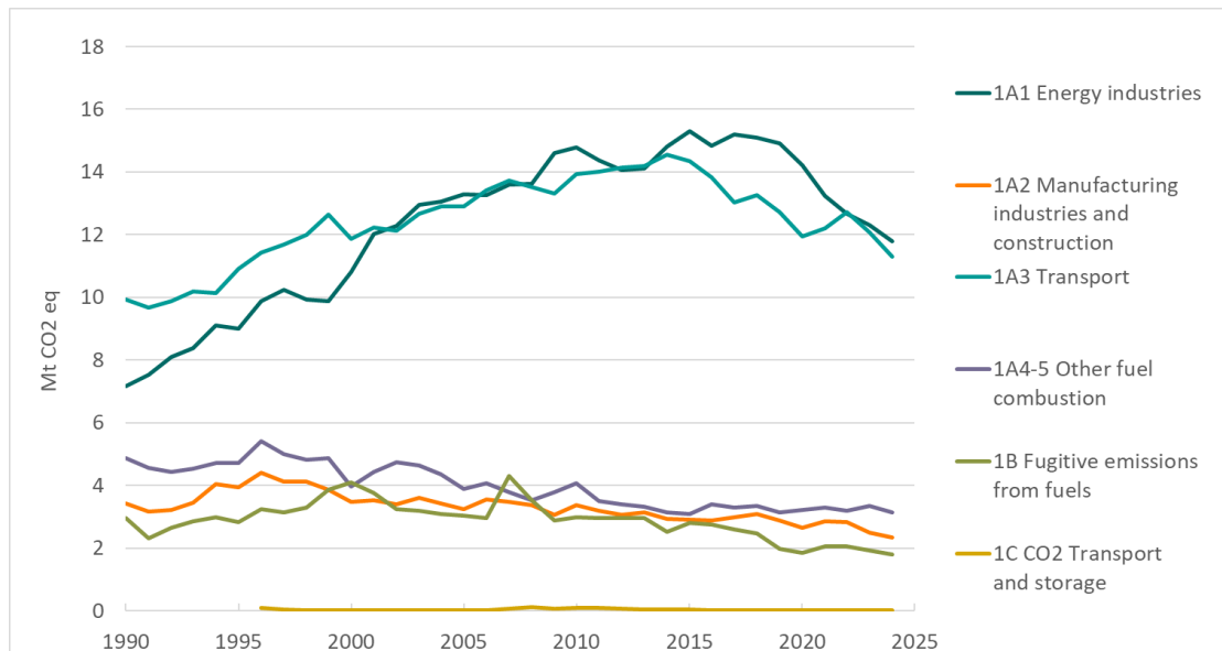
Figure 3.1: Greenhouse gas emissions from energy sectors and fugitive emissions. Million tonne CO 2 equivalents. Source: Statistics Norway/Norwegian Environment Agency.
