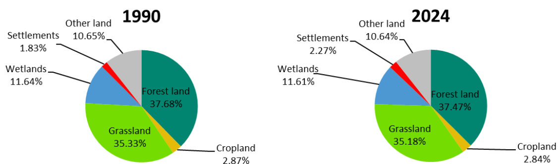
Figure 6.11: Area distribution of the IPCC land-use categories for 1990 and the latest reporting year. Source: Norwegian Institute of Bioeconomy Research.
