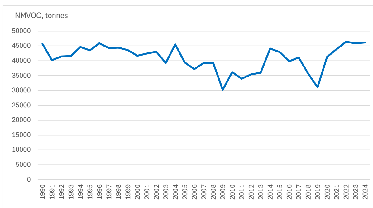
Figure 4.6: Emissions from solvent use illustrating inter-annual changes, emissions in tonnes NMVOC.
