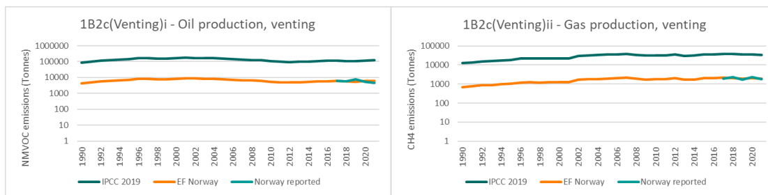
Figure 3.23: NMVOC emissions using IPCC default factors and country specific emission factors, respectively.
