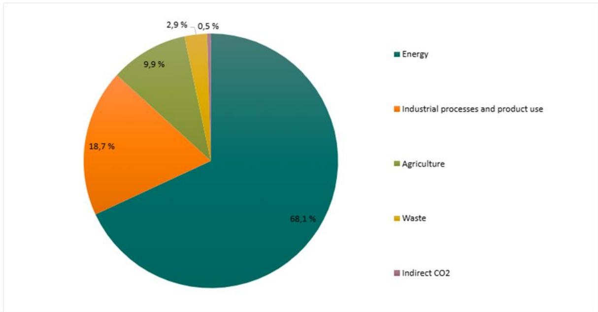
Figure ES.2: Emissions by IPCC sector in 2024, excluding LULUCF. Source: Statistics Norway/Norwegian Environment Agency.
