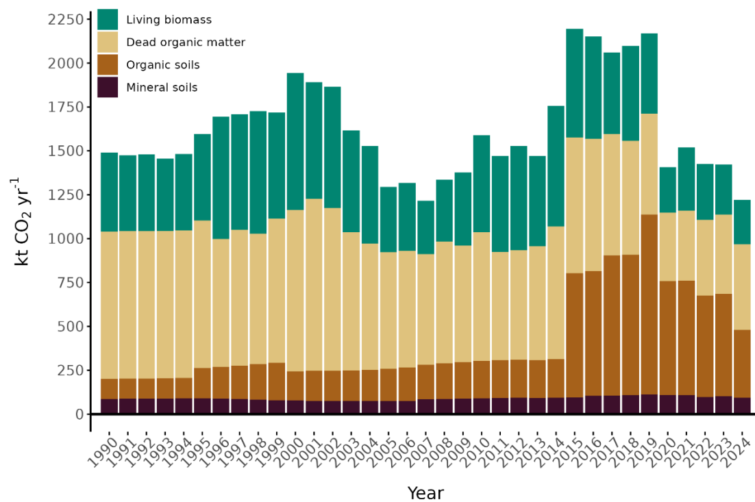
Figure 6.6: Net emissions and removals of CO 2 on settlements, including both remaining and land converted to settlements. The graph shows the aggregated net emissions and removals for both categories. Carbon pools can either act as a source or sink of CO 2 , depending on the category, although this might not always be visible in the graph. Non-CO 2 emissions and removals are not included in the graph. Source: Norwegian Institute of Bioeconomy Research.
