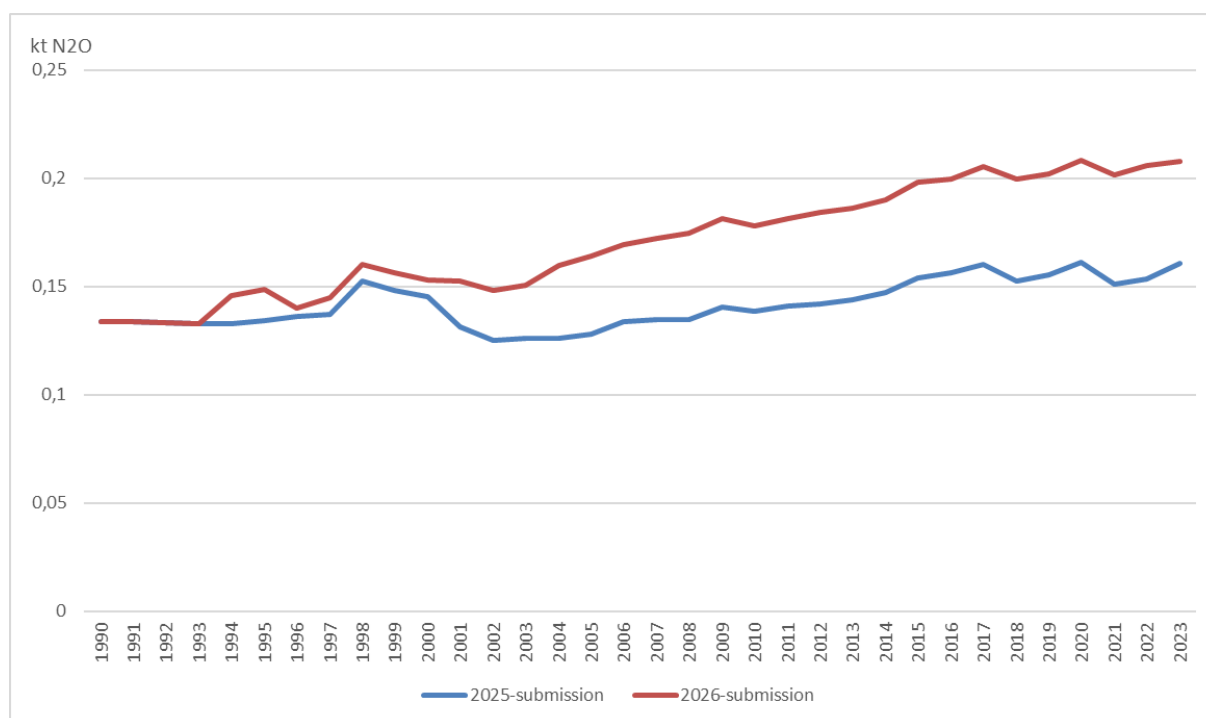
Figure 10.3: Comparison of N 2 O emissions from domestic wastewater between the 2025- and 2026-submissions.
