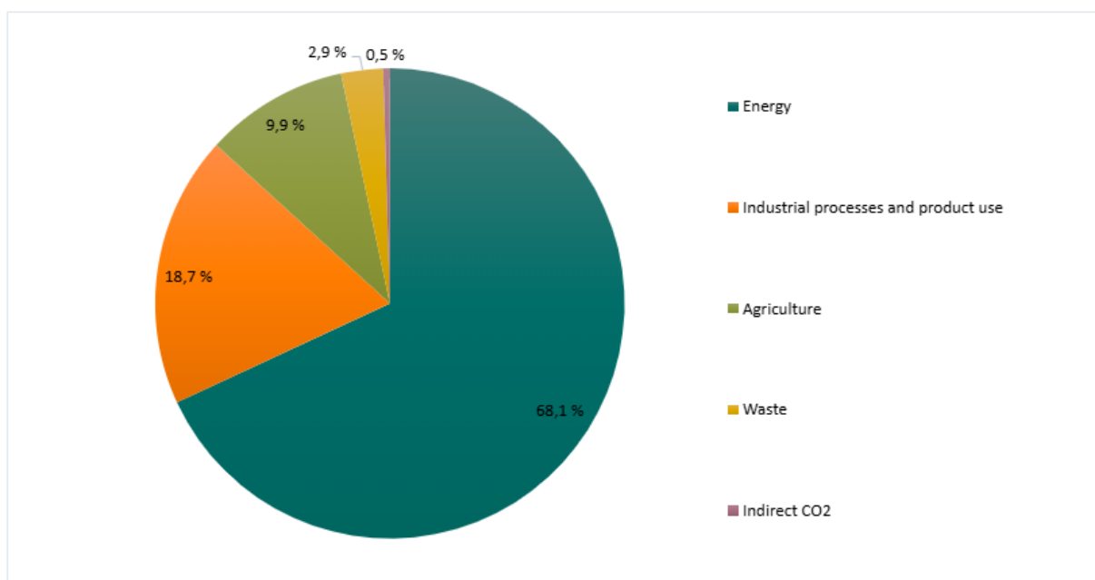
Figure 2.3: Distribution of GHG emissions (without LULUCF) in Norway in 2024 by sector. Indirect CO 2 emissions is also shown. Source: Statistics Norway/Norwegian Environment Agency.
