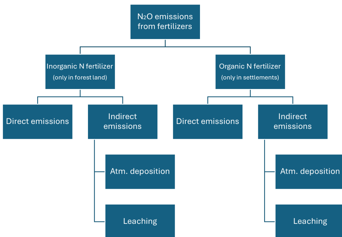
Figure 6.35: Reporting structure under Direct and Indirect N 2 O emissions from fertilizers.
