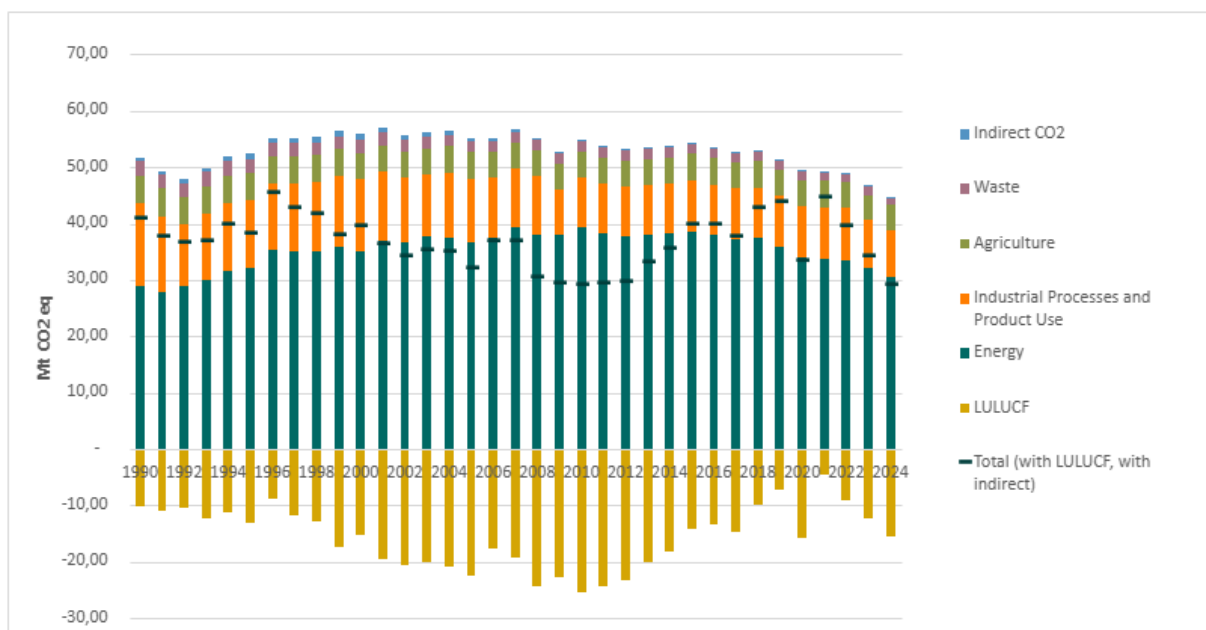
Figure 2.1: Total emissions of greenhouse gases by sources and removals from LULUCF in Norway, 1990-2024 (Mtonnes CO 2 equivalents). Source: Statistics Norway/Norwegian Environment Agency/Norwegian Institute of Bioeconomy Research.
