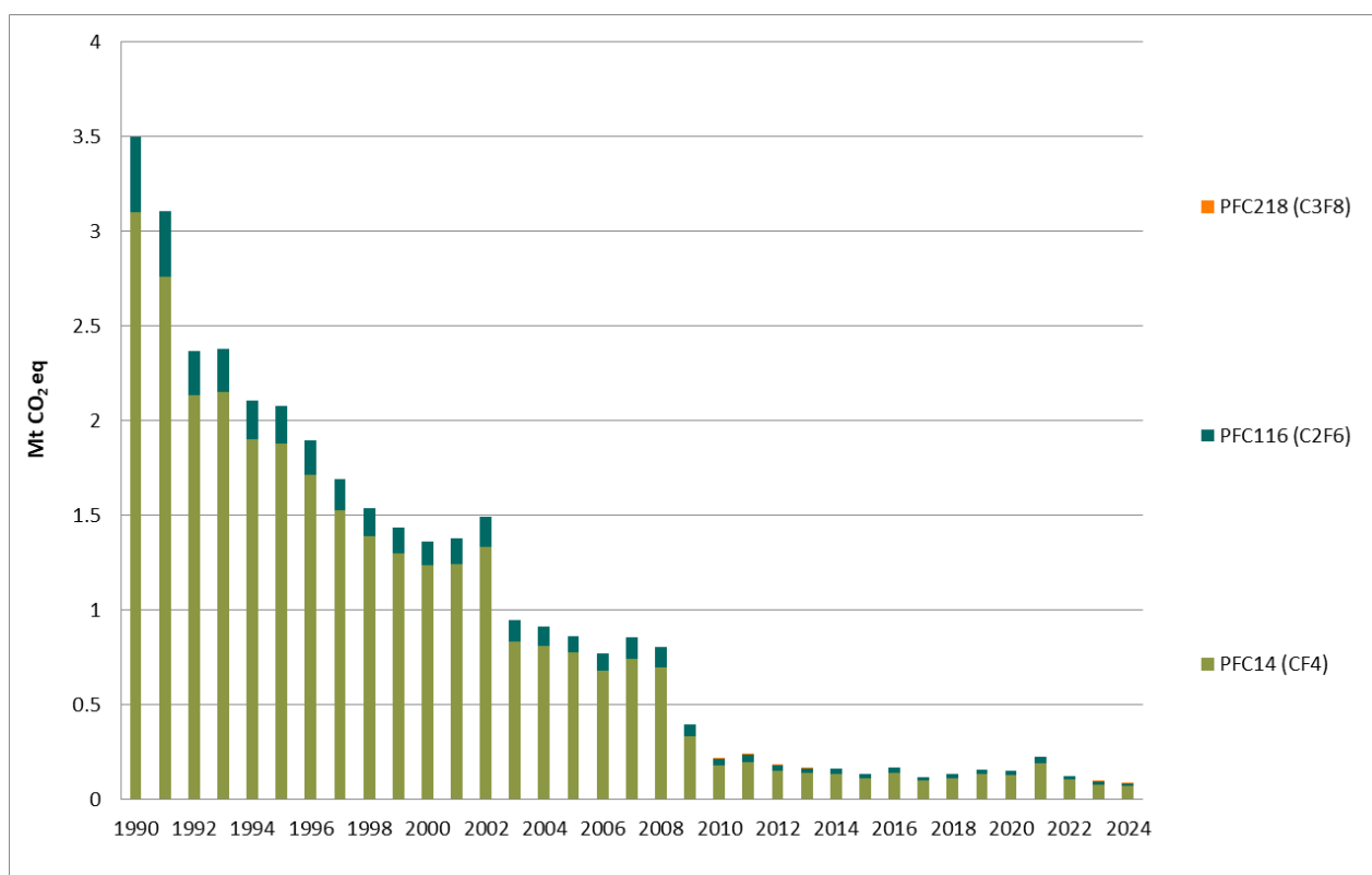
Figure 2.21: Emissions (million tonnes CO 2 eq.) of PFCs in Norway, 1990-2024. Source: Statistics Norway/Norwegian Environment Agency.
