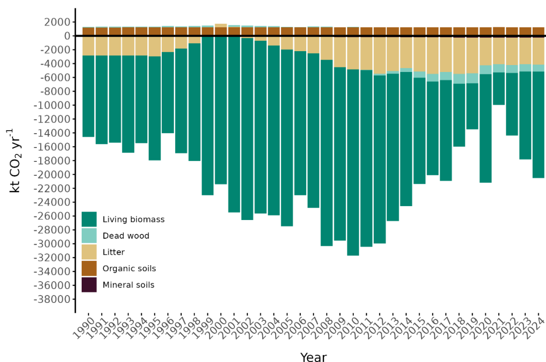
Figure 6.2: Net emissions and removals of CO 2 on forest land, including both remaining and land converted to forest land. The graph shows the aggregated net emissions and removals for both categories. Carbon pools can either act as a source or sink of CO 2 , depending on the category, although this might not always be visible in the graph. Non-CO 2 emissions and removals are not included in the graph. Source: Norwegian Institute of Bioeconomy Research.
