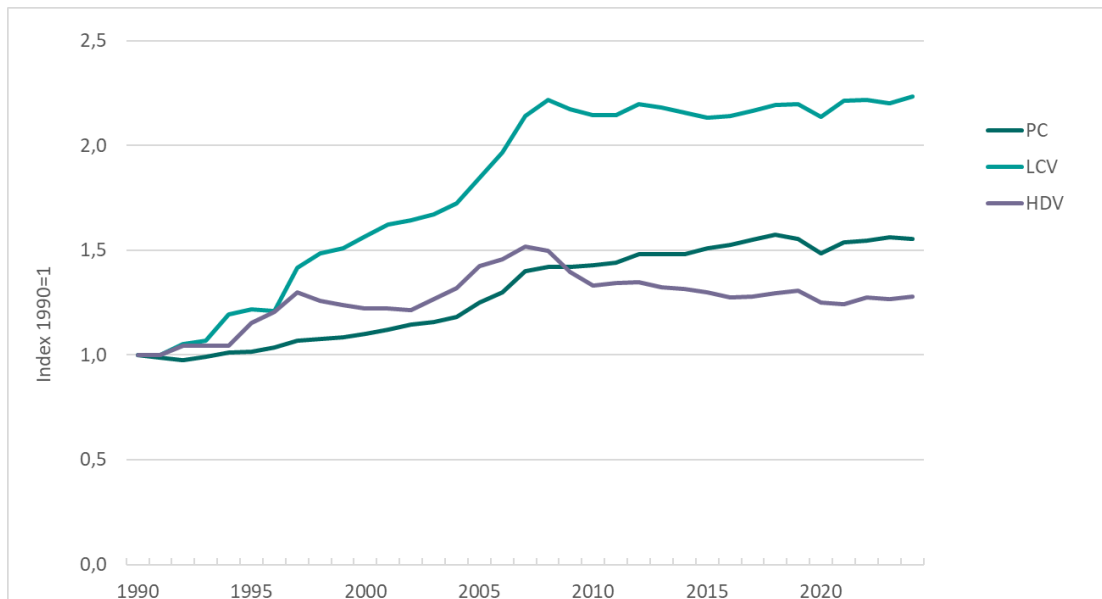
Figure 3.13: Relative change to 1990 in total vehicle kilometres. PC, LCV, HDV. Index 1990=1. Source: Statistics Norway/Norwegian Environment Agency.
