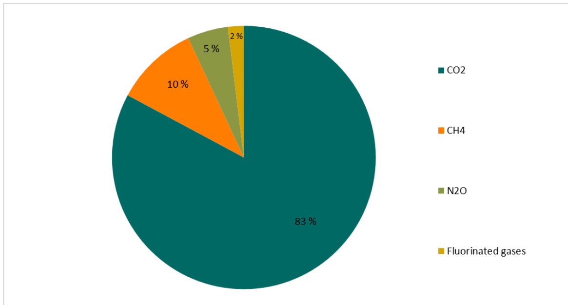
Figure 2.13: Distribution of emissions of greenhouse gases in Norway by gas (in CO 2 equivalents), 2024. Source: Statistics Norway/Norwegian Environment Agency.
