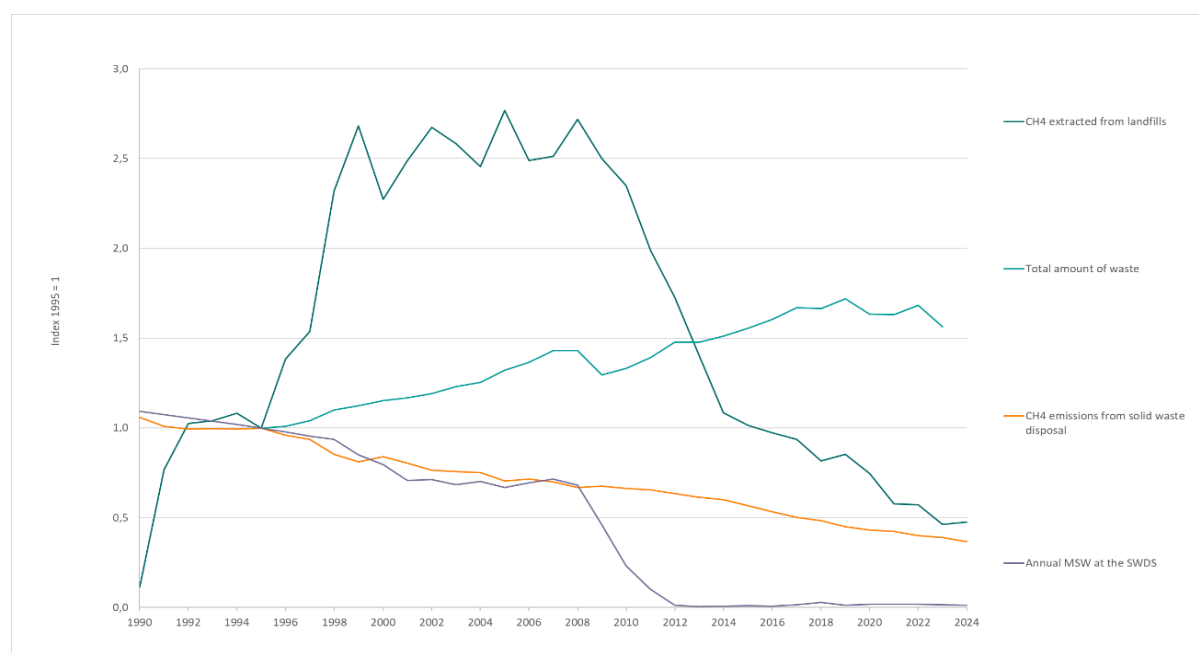
Figure 7.1: Relative change in methane emissions from solid waste disposal, annual MSW at the SWDS, methane extracted from landfills and total amount of waste generated in Norway. 1990-2024 Index
