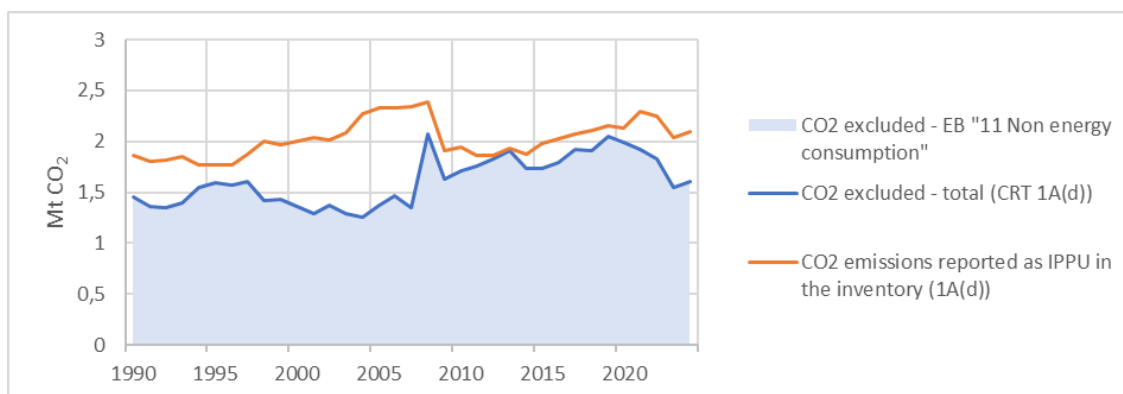
Figure 3.7: Petroleum coke. CO 2 amounts excluded from the reference approach (shaded areas, blue line) and reported as IPPU emissions (orange line). IPPU sectors reported in the inventory include:
