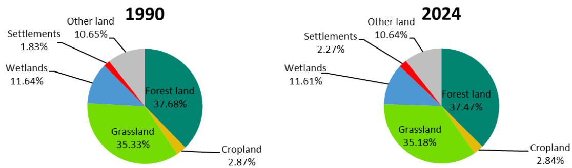
Figure 2.10: Area (%) distribution between the IPCC land-use categories, 1990 and 2024. Source: The Norwegian Institute of Bioeconomy Research.
