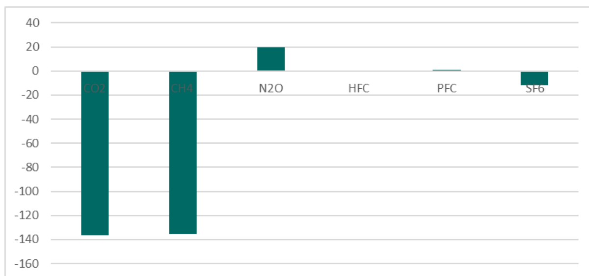
Figure 1-4: Difference in total emissions for 2023 per gas, excluding LULUCF, between latest and previous submission. 1000 tonnes CO 2 equivalents.
