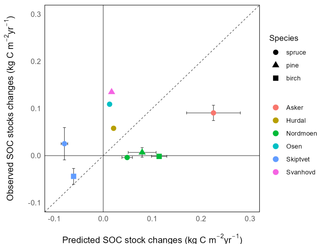
Figure 6.28: Relationship between observed and simulated changes in soil organic carbon (SOC) stocks for six forest sites. Simulated SOC CSC are based on the Yasso20 model of SOC dynamics and according to the default methodology of the LULUCF reporting (DEFAULT). Error bars represent the standard errors (SEM) of observed and simulated SOC CSC. In the plot, changes for the sites are shown separately for different dominant tree species by the shape of the point. For sites Osen, Hurdal, and Svanhovd, only the mean of pseudo-replicates is shown (mean over pseudo-replicates). The dashed line represents the line of equality: a 1:1 relationship between observed and simulated SOC changes.
