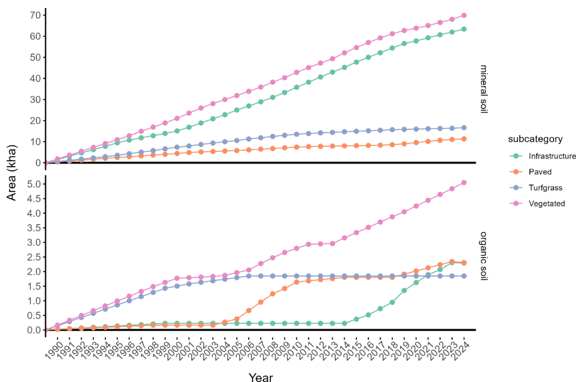
Figure 6.33: Cumulative land-use change area to settlement subcategories since 1990 (excluding 20-year transition rule to remaining category). The area separation between mineral and organic soil is based on what the soil of the area was originally classified as before the conversion, and not the classification after land-use change.
