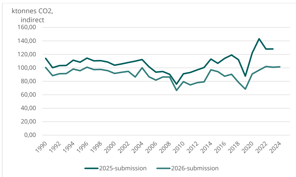
Figure 10.1: Illustration of recalculated indirect CO 2 emissions from solvent use due to updated activity data. Emissions reported in CRT Table 6.
