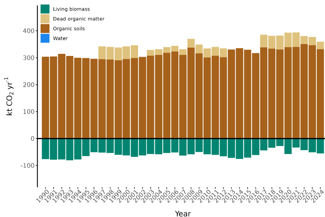
Figure 6.5: Net emissions and removals of CO 2 on wetland, including both remaining and land converted to wetland. The graph shows the aggregated net emissions and removals for both categories. Carbon pools can either act as a source or sink of CO 2 , depending on the category, although this might not always be visible in the graph. Non-CO 2 emissions and removals are not included in the graph. Source: Norwegian Institute of Bioeconomy Research.
