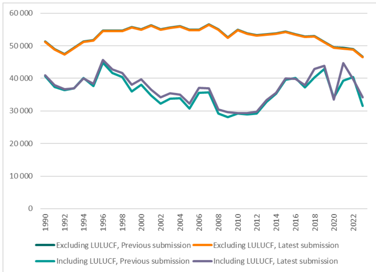
Figure 10.4: Total emissions with and without LULUCF. Previous and latest submission. 1000 tonnes CO 2 equivalents.
