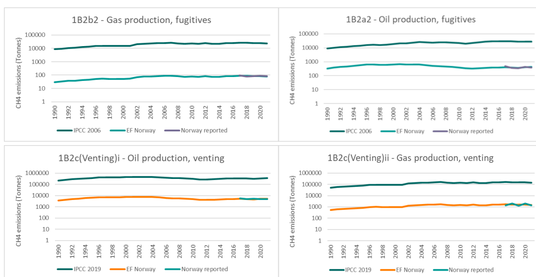
Figure 3.22: CH 4 emissions IPCC default factors and country specific emission factors, respectively.
