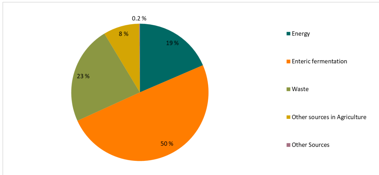
Figure 2.17: Distribution of Norwegian CH 4 emissions by major sources in 2024. Source: Statistics Norway/Norwegian Environment Agency.
