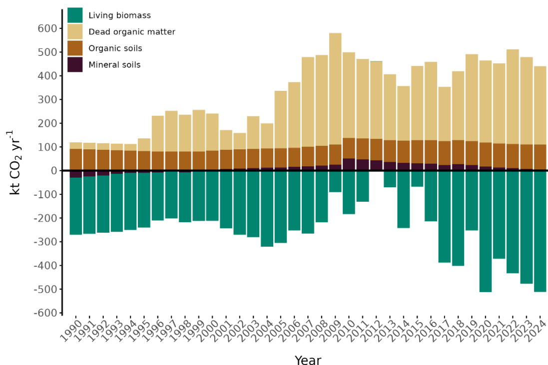
Figure 6.4: Net emissions and removals of CO 2 on grassland, including both remaining and land converted to grassland. The graph shows the aggregated net emissions and removals for both categories. Carbon pools can either act as a source or sink of CO 2 , depending on the category, although this might not always be visible in the graph. Non-CO 2 emissions and removals are not included in the graph. Source: Norwegian Institute of Bioeconomy Research.
