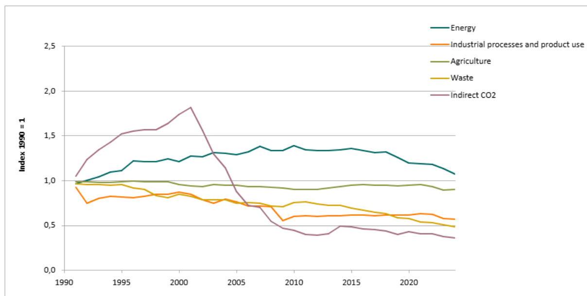
Figure 2.2: Changes in emissions of greenhouse gases, relative to 1990, by sectors, 1990-2024. The development in indirect CO 2 emissions is also shown. Index 1990 = 1. Source: Statistics Norway/Norwegian Environment Agency.
