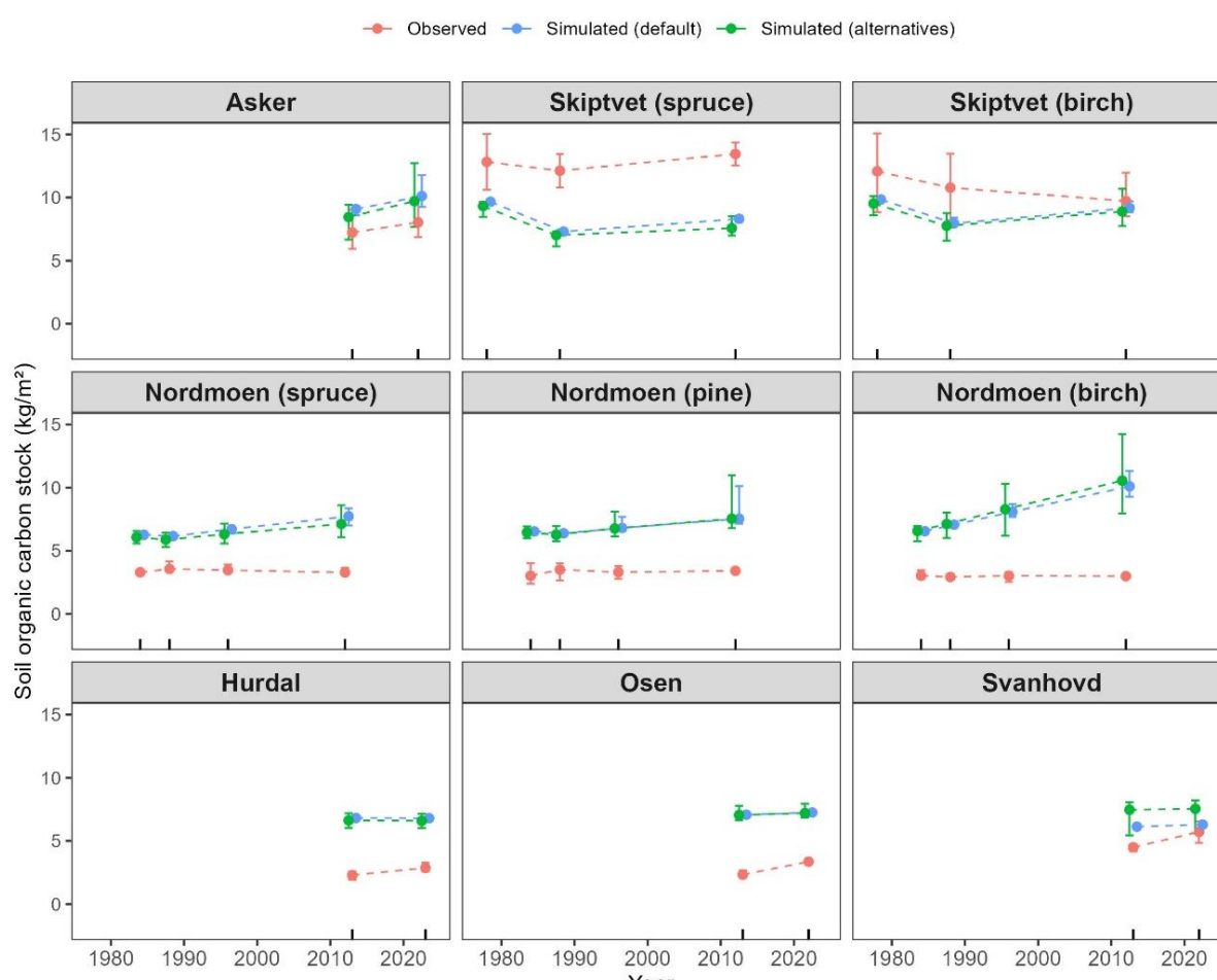
Figure 6.26: Development of soil organic carbon (SOC) stock for forest sites based on observed data and simulated predictions. Red data points represent the observed SOC stock, while blue data points show simulated SOC predictions based on the Yasso20 model of SOC dynamics, following the default methodology as used in the LULUCF reporting. Green data points represent SOC predictions using 15 alternative simulation methodologies (see text). Each data points indicate the median (50th percentile) SOC stock at the site-level. Error spans range from the 25th percentile (Q1) to the 75th percentile (Q3). Data points and error bars for Hurdal, Osen, and Svanhovd are based on bulked soil samples in four
