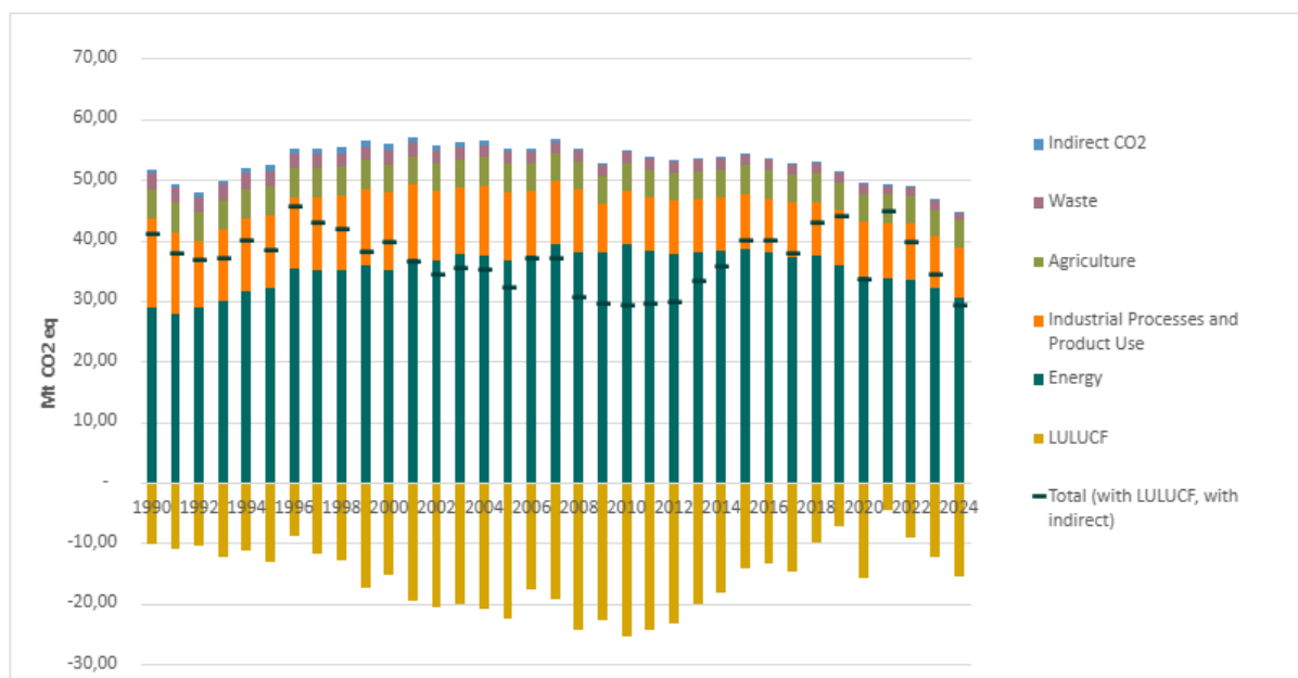
Figure ES.1: Total emissions of greenhouse gases by sources, and removals from LULUCF in Norway, 1990-2024 (Mtonnes CO 2 equivalents). Source: Statistics Norway/Norwegian Environment Agency/Norwegian Institute of Bioeconomy Research.
