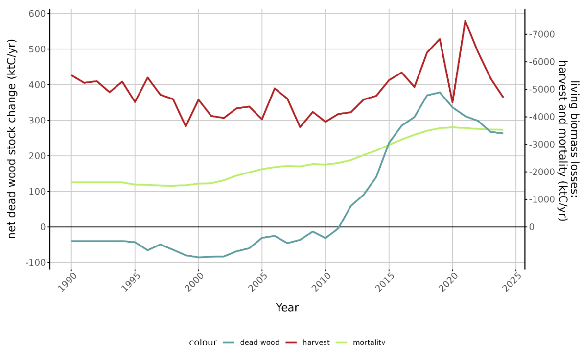
Figure.6.24: Temporal dynamics in mortality and harvest and Yasso20-simulated carbon stocks in the dead wood pool.
