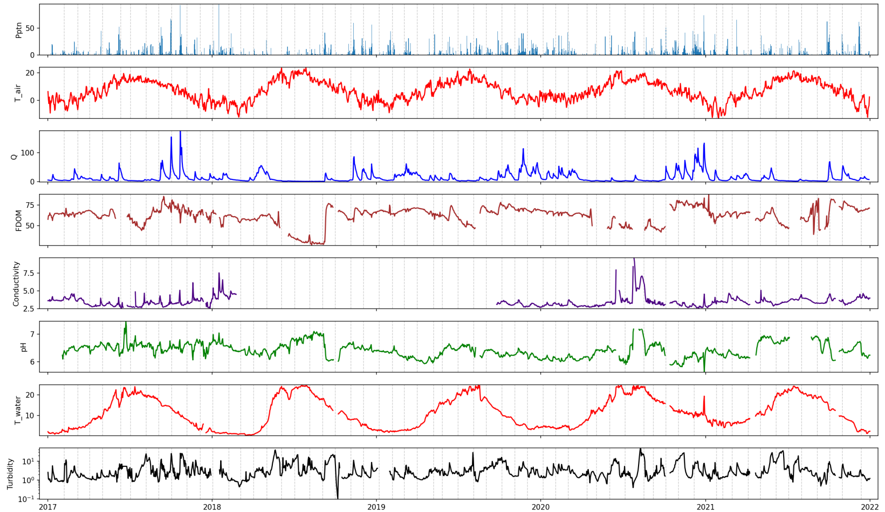
Figure 2. Time series for weather variables (Pptn: precipitation, T air : air temperature), discharge (Q) and in situ sensor observations for Storelva (T water is water temperature). Vertical lines show grab sampling dates.
