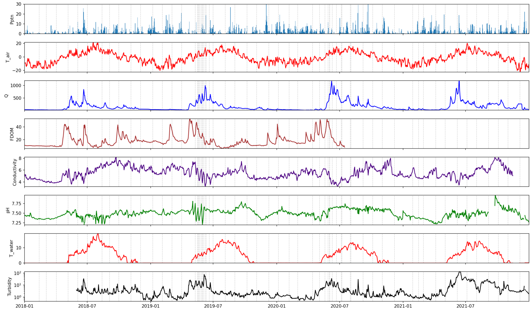
Figure 3. Time series for weather variables (Pptn: precipitation, T air : air temperature), discharge (Q) and in situ sensor observations for Målselva (T water is water temperature). Vertical lines show grab sampling dates, including extra high frequency sampling during spring 2019 and 2020.
