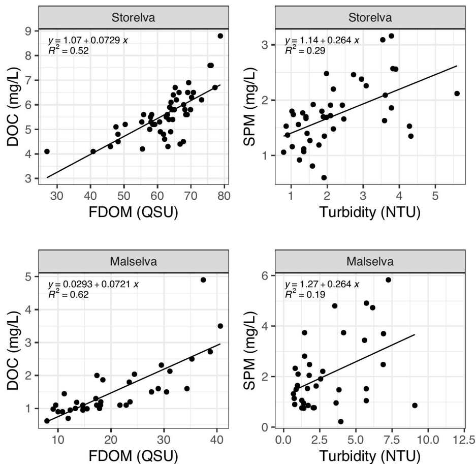
Figure 12. Relationships between in situ sensor-based measurements and discrete grab samples for DOC vs. FDOM and SPM vs. turbidity in Storelva (top left and right, respectively), and Målselv (bottom left and right, respectively). Regressions include all available paired data. Results of linear regression are shown in the figures. All regressions were significant ( p < 0.001 ) except for SPM vs. turbidity relationship in Målselv ( p = 0.42 ).
