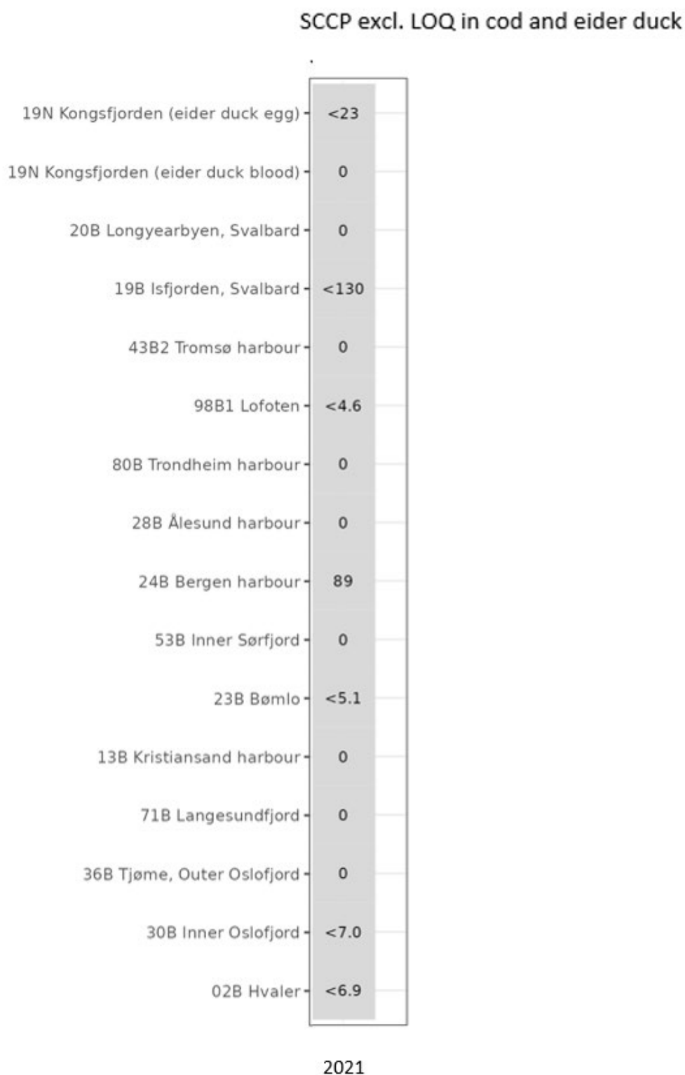
Figure 82. Heatmaps of MSCP and SCCP in blue mussel and cod/eider. For full explanation of figure see example Figure 23. NB: In these heatmaps, only data from 2021 are shown. For these data, the median concentrations are set to 0 when all samples for a station were below LOQ. When there were one or more samples above LOQ, the median concentrations were set to < "the lowest of the quantified values". This also applies to Figure 83 .
