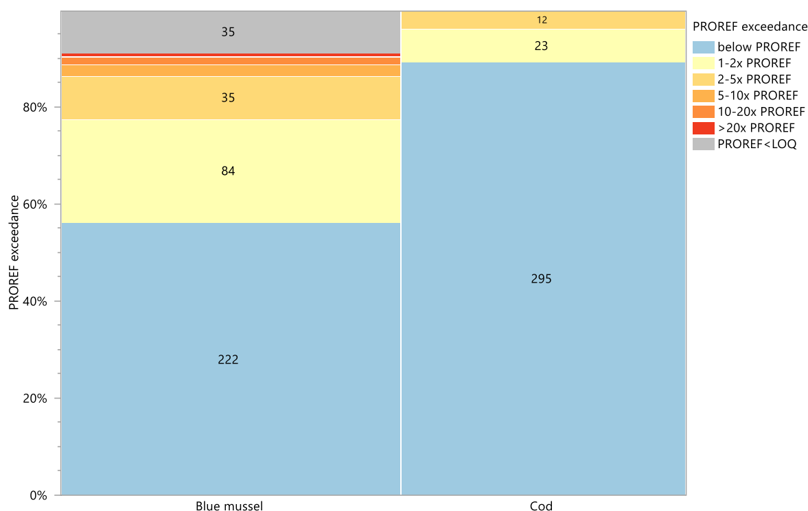
Figure 11. Exceedances of PROREF in a mosaic plot. The cells are labelled by the number of datapoints (stations × contaminants). The exceedances are considered by the median for each station and species. The colours represent below (blue) or above PROREF (darker yellow to red), or that the PROREF was below LOQ, and therefore could not be classified (grey).
