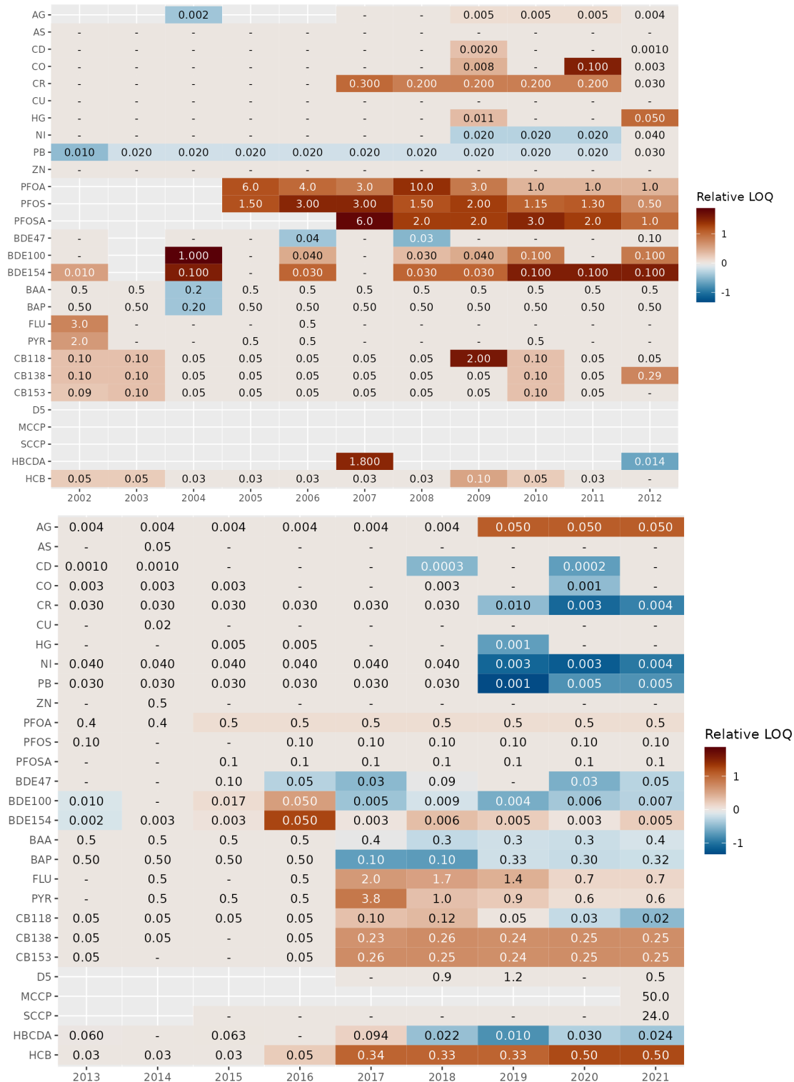
Figure 3. Changes in LOQ values over time. The numbers in the table show observed LOQ (median values, mg/kg ww for metals incl. Hg, and ug/kg ww for others). In blue mussel for various compounds in the periods 2002-2012 (a) and 2013-2021 (b). The colors indicate the “relative LOQ” on a logarithmic scale compared to the reference period 2013-2015 (median LOQ versus the median LOQ during the years 2013-2015), with blue colors showing lower (better) LOQ, and brown colors showing higher LOQ compared to the reference period. For some groups, e.g. PFAS, there were no measurements in the reference period (shown in light grey).
