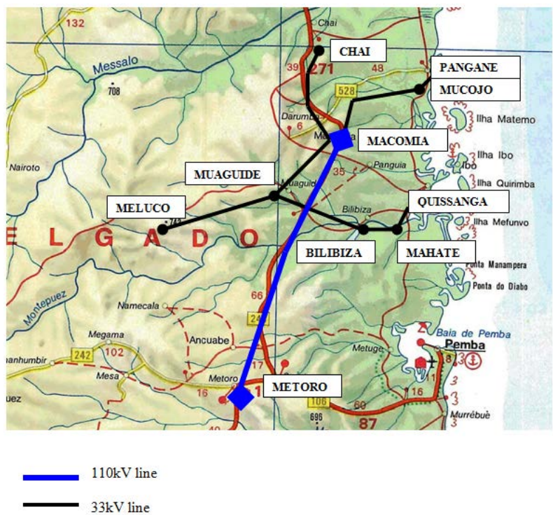
Figure 1. Map of the Cabo Delgado rural electrification project, Lot 1 (EDM)
