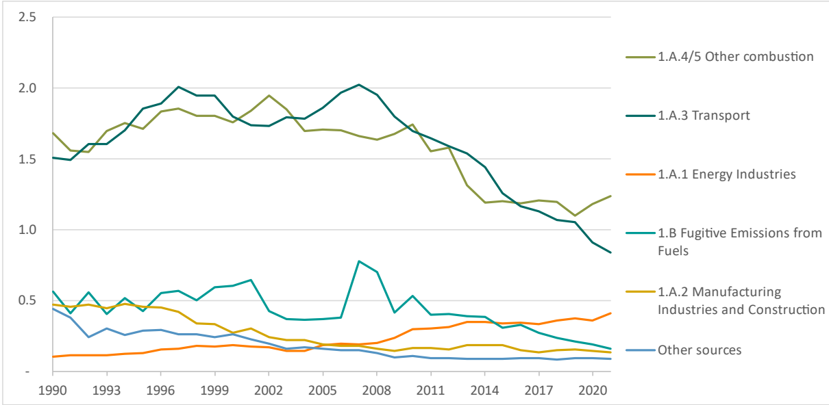
Figure 2.17. Trends in BC emissions, 1990-2021. 1000 tonnes
