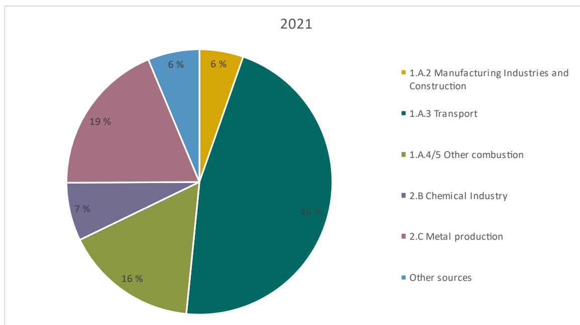
Figure 2.31. Distribution of lead emissions between emission sources, 2021. Per cent
