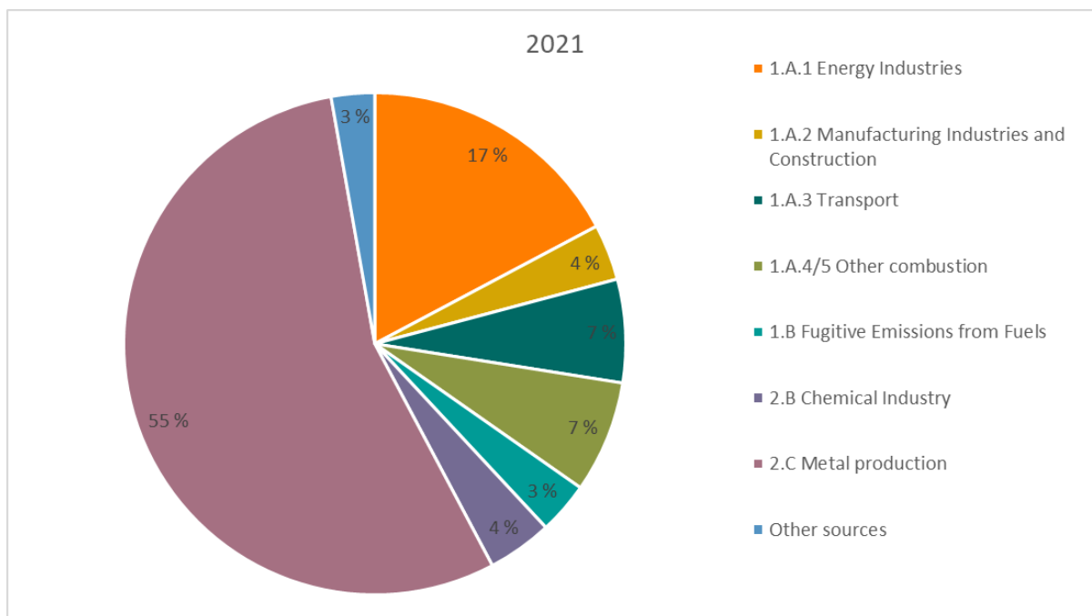
Figure 2.5. Distribution of SO 2 emissions between emission sources, 2021. Per cent
