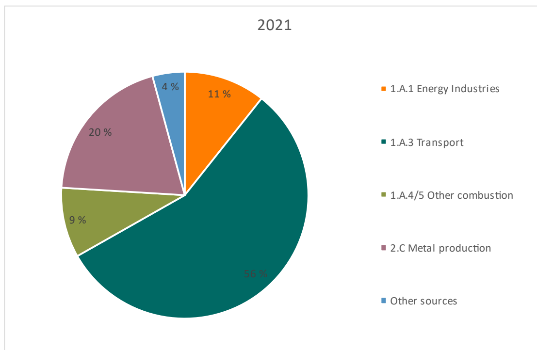
Figure 2.26. Distribution of HCB emissions between emission sources, 2021. Per cent
