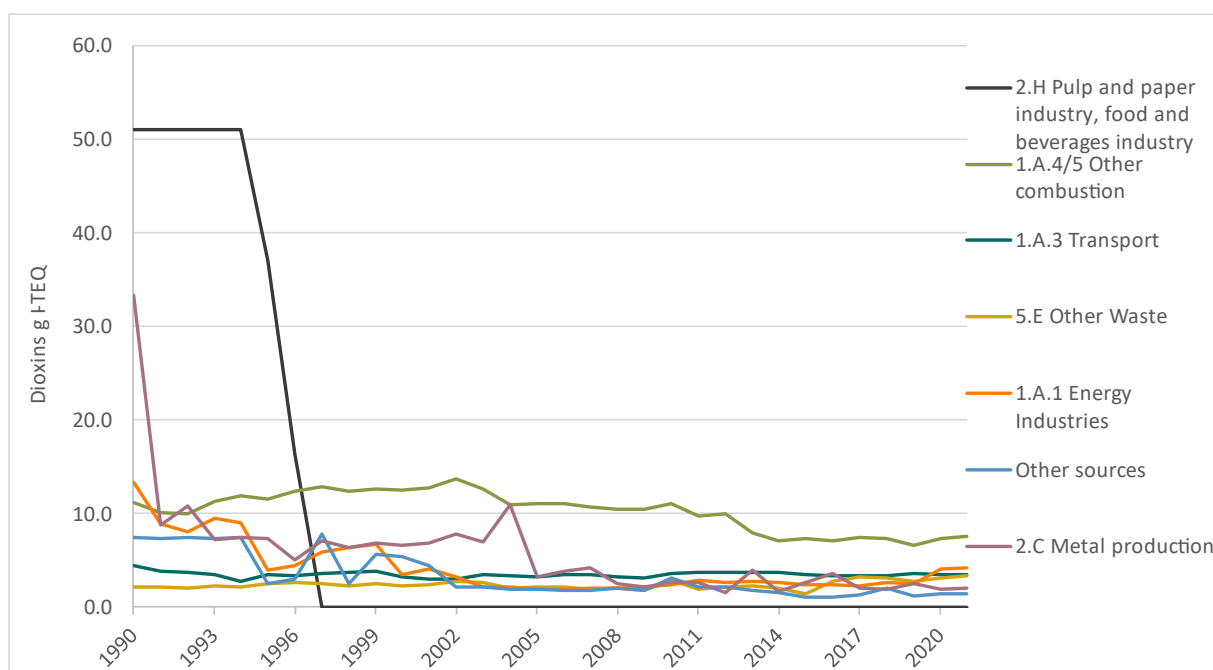
Figure 2.19. Trends in dioxins emissions, 1990-2021. Gram I-TEQ
