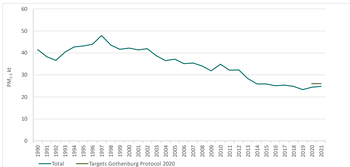
Figure 2.16. Trends in PM 2.5 emissions, 1990-2021. 1000 tonnes
