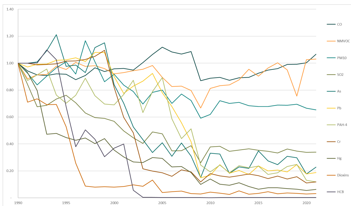
Figure 4.1. Trends for the emissions for most of long-range transboundary air pollutants from IPPU, relative to 1990
