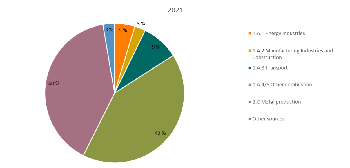
Figure 2.11. Distribution of CO emissions between emission sources, 2021. Per cent Source: Statistics Norway/Norwegian Environment Agency
