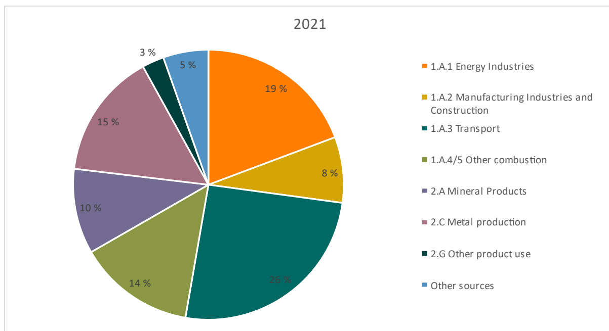
Figure 2.35. Distribution of mercury emissions between emission sources, 2021. Per cent
