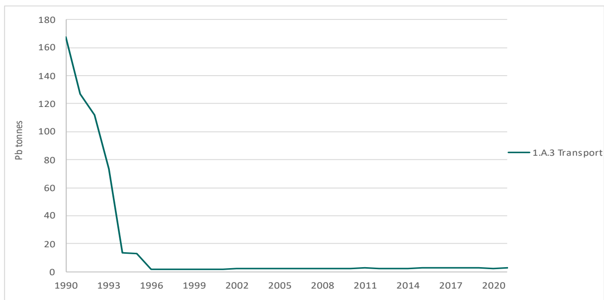
Figure 2.29. Transport, trends in lead emissions, 1990-2021. Tonnes
