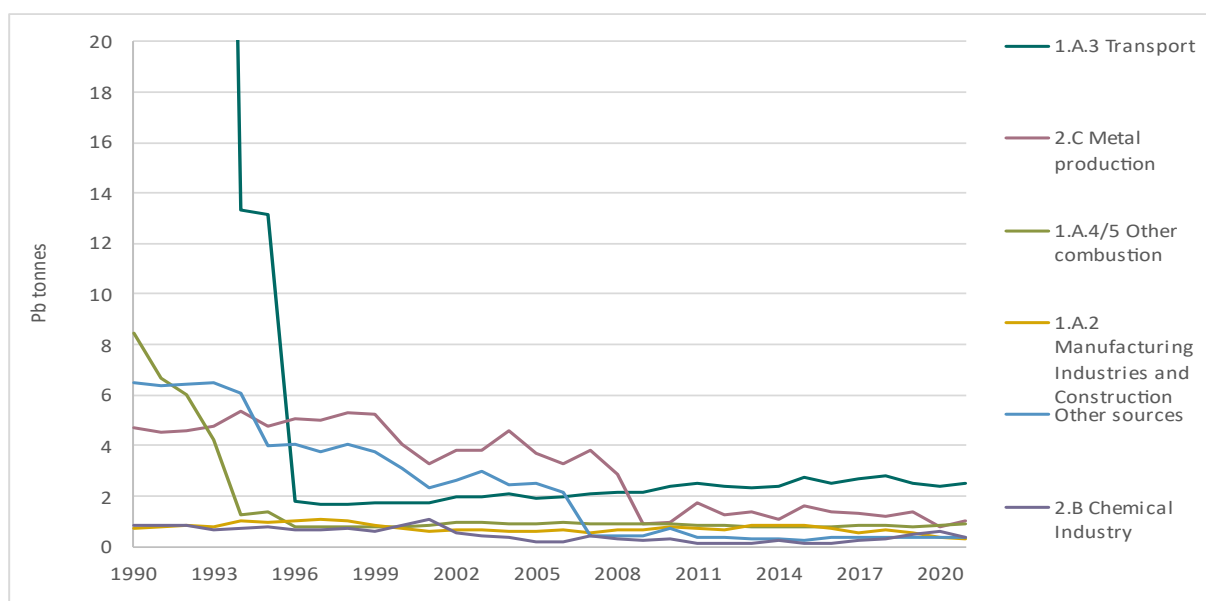
Figure 2.30. Trends in lead emissions, 1990-2021. Tonnes
