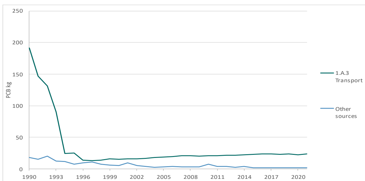
Figure 2.27. Trends in total PCB emissions, 1990-2021. Kilogram
