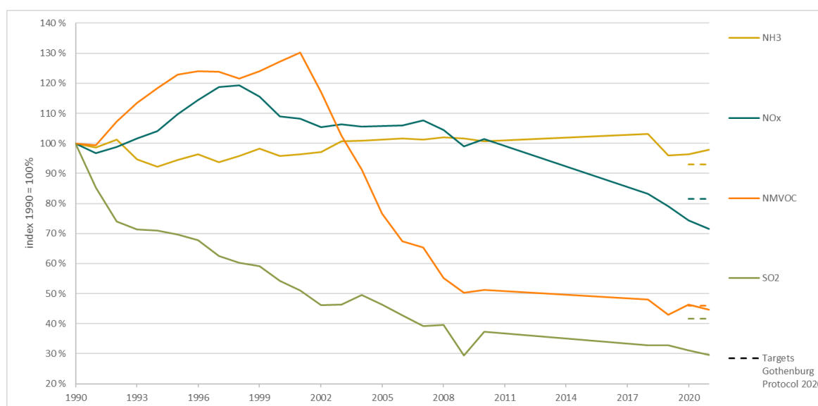
Figure 2.1. Trends in emissions for NO x , SO 2 , NH 3 and NMVOC. 1990-2021. Index 1990 = 100%
