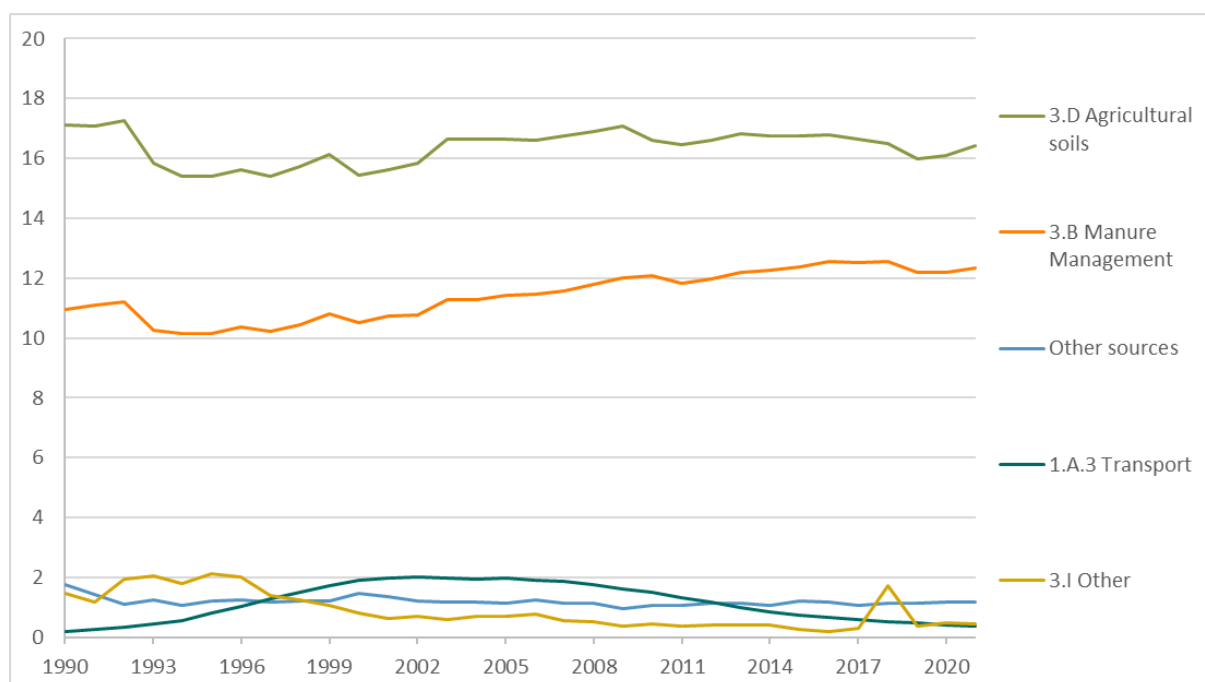
Figure 2.6. Trends in NH 3 emissions, 1990-2021. 1000 tonnes
