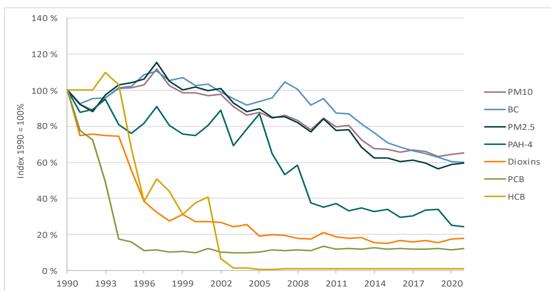
Figure 2.12. Trends in emissions for PAH-4, dioxins, PCB, HCB and BC. 1990-2021. Index 1990=100%
