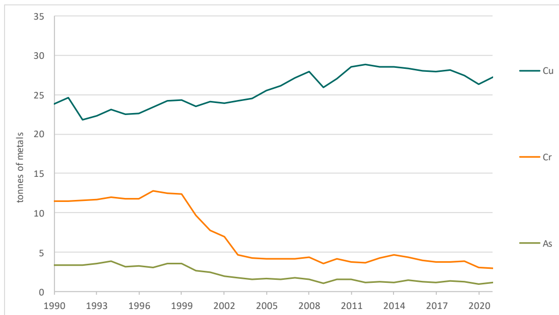
Figure 2.36. Trends in copper, chromium, and arsenic emissions, 1990-2021. Tonnes
