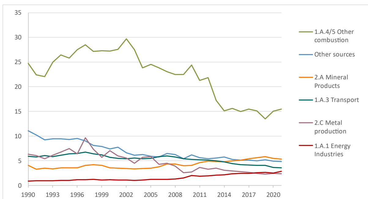
Figure 2.14. Trends in PM 10 emissions, 1990-2021. 1000 tonnes
