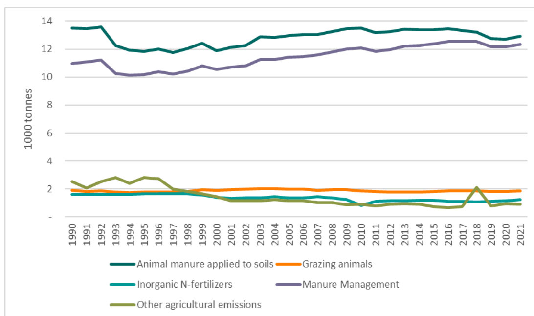
Figure 5.2 Trends for the NH 3 emissions for agricultural sources. 1000 tonnes NH 3 . 1990-2020. Source: Statistics Norway/ Norwegian Environment Agency
