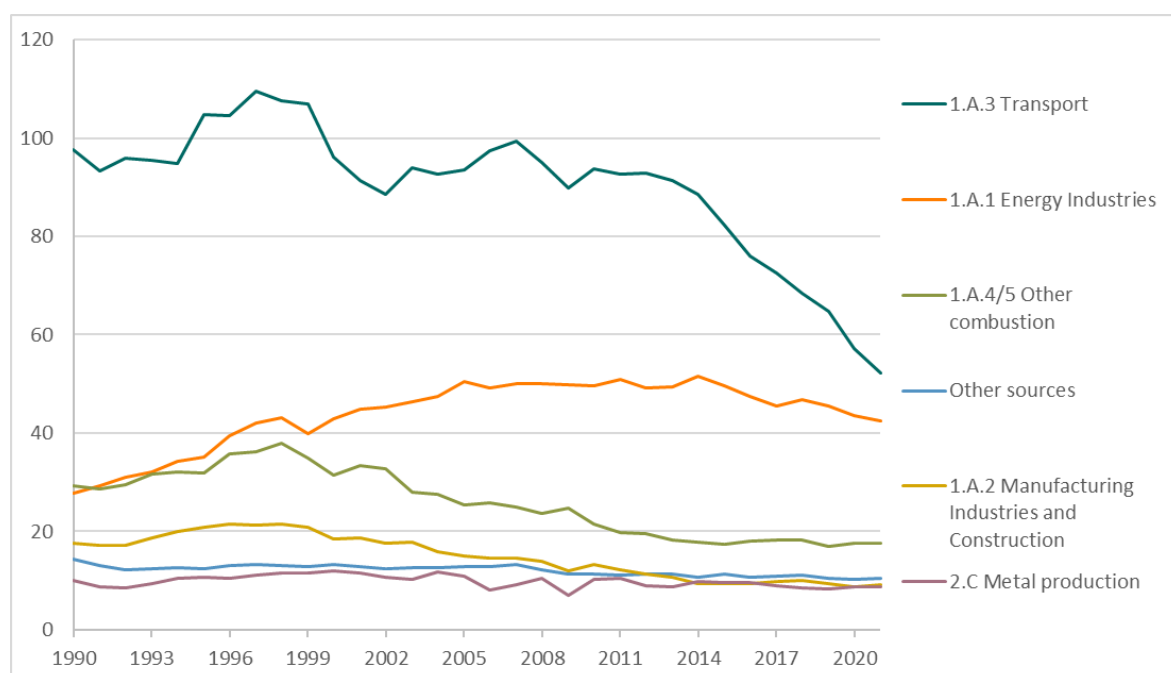
Figure 2.2. Trends in NO x emissions, 1990-2021. 1000 tonnes
