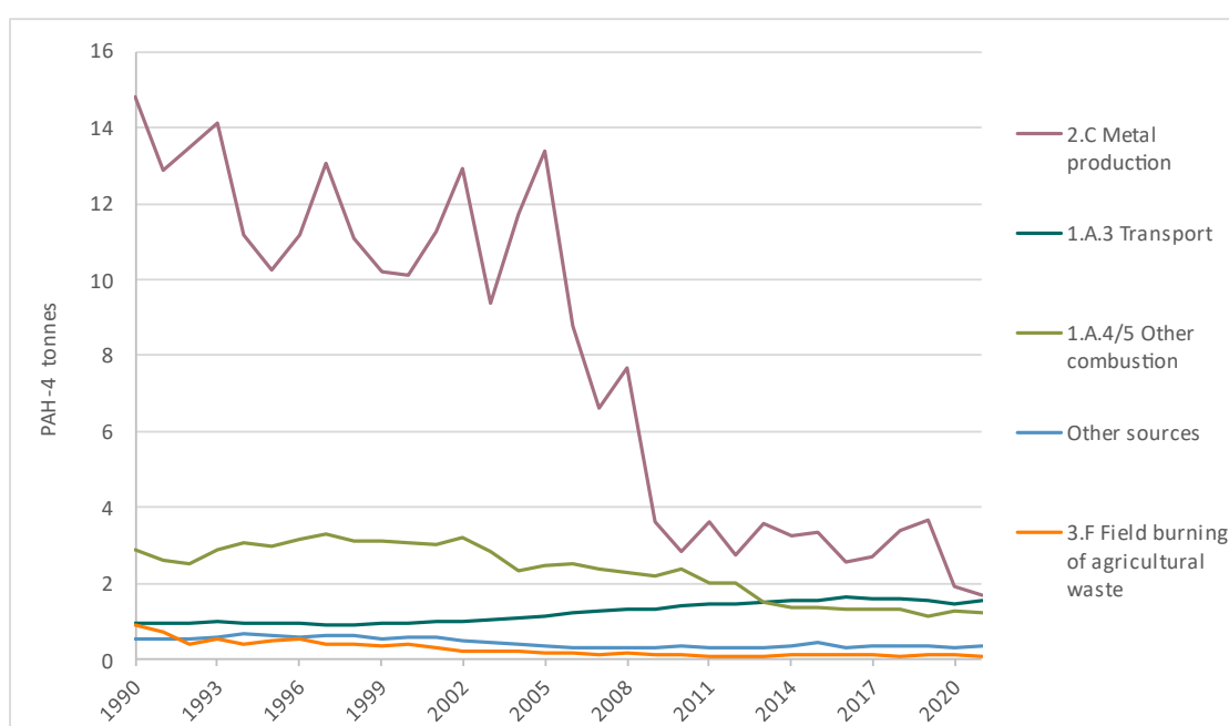
Figure 2.22. Trends in total PAH-4 emissions, 1990-2021. Tonnes
