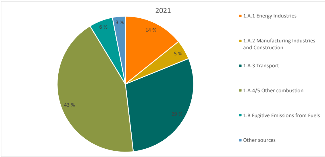
Figure 2.18. Distribution of BC emissions between emission sources, 2021. Per cent
