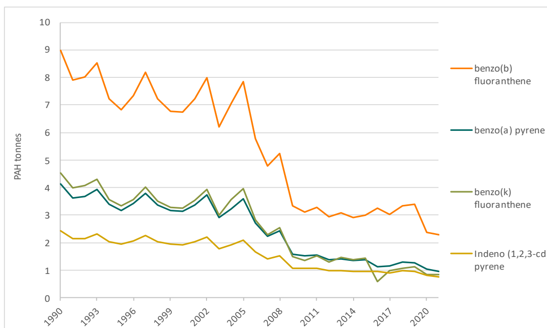
Figure 2.21. Trends in PAH emissions, benzo(a)pyrene, benzo(b)fluoranthene, benzo(k)fluoranthene and indeno(1,2,3-cd)pyrene, 1990-2021. Tonnes
