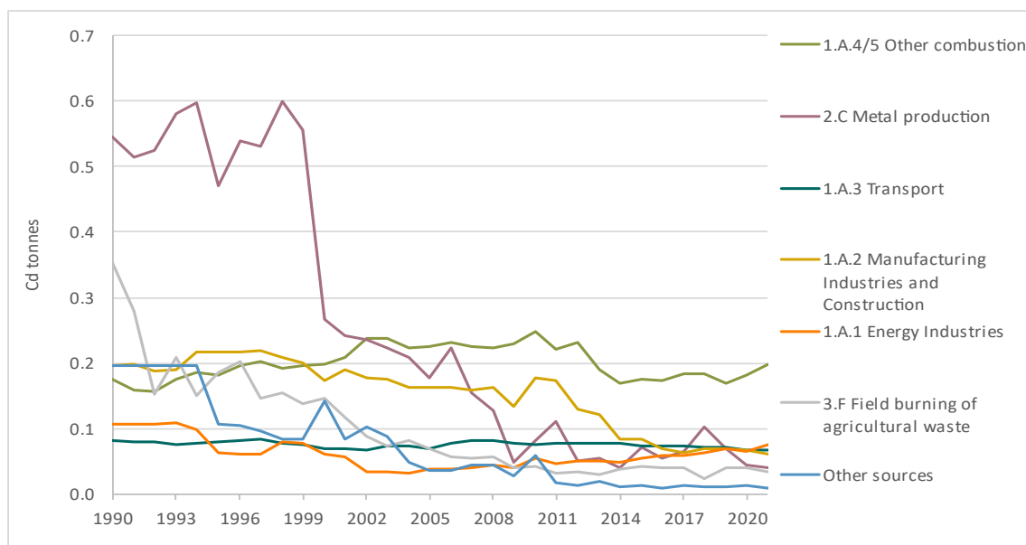
Figure 2.32. Trends in cadmium emissions, 1990-2021. Tonnes
