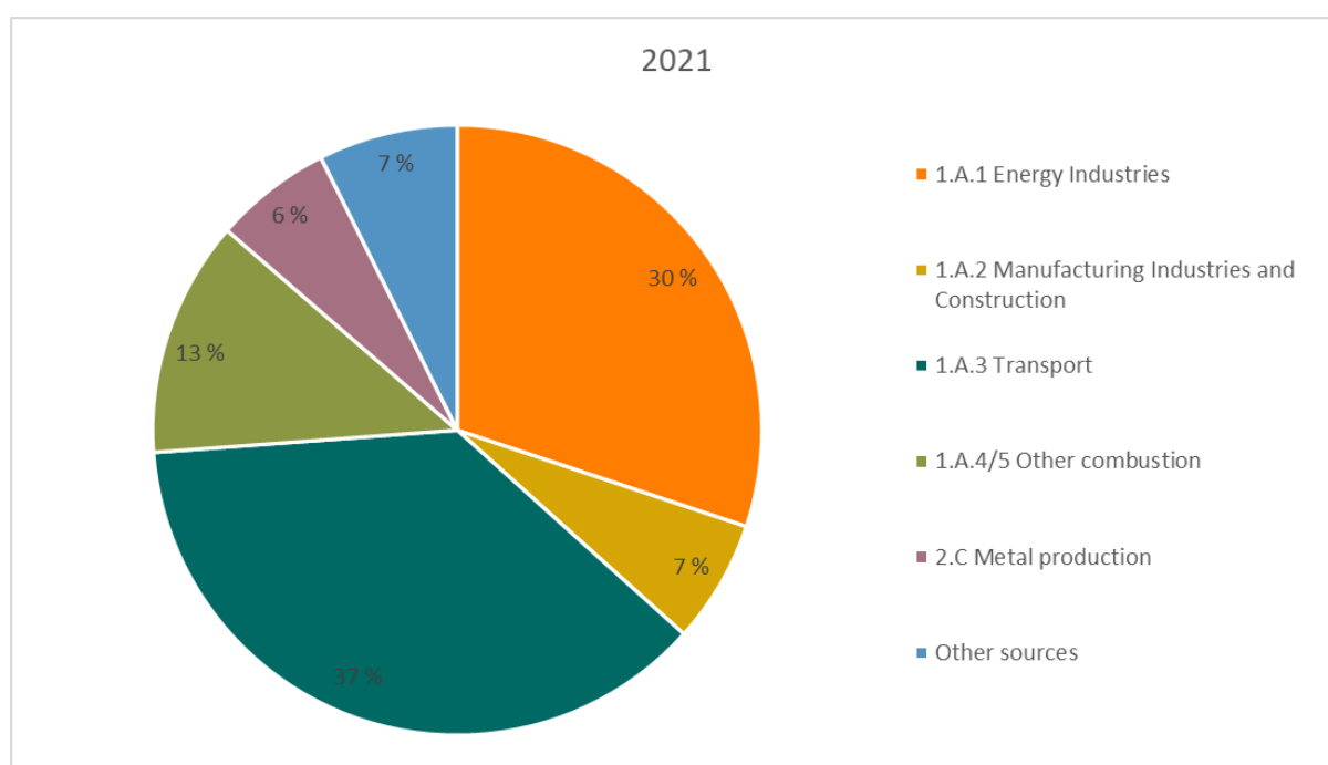
Figure 2.3. Distribution of NO x emissions between emission sources, 2021. Per cent
