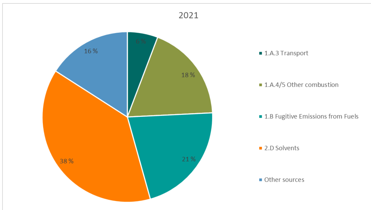
Figure 2.9. Distribution of NMVOC emissions between emission sources, 2021. Per cent
