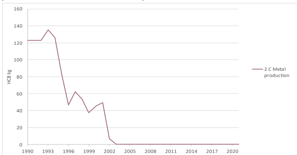
Figure 2.24. Metal industry, trends in HCB emissions, 1990-2021. Kilogram
