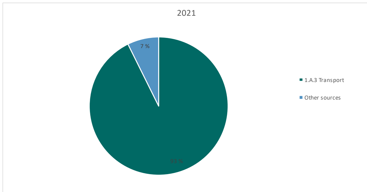
Figure 2.28. Distribution of PCB emissions between emission sources, 2021. Per cent
