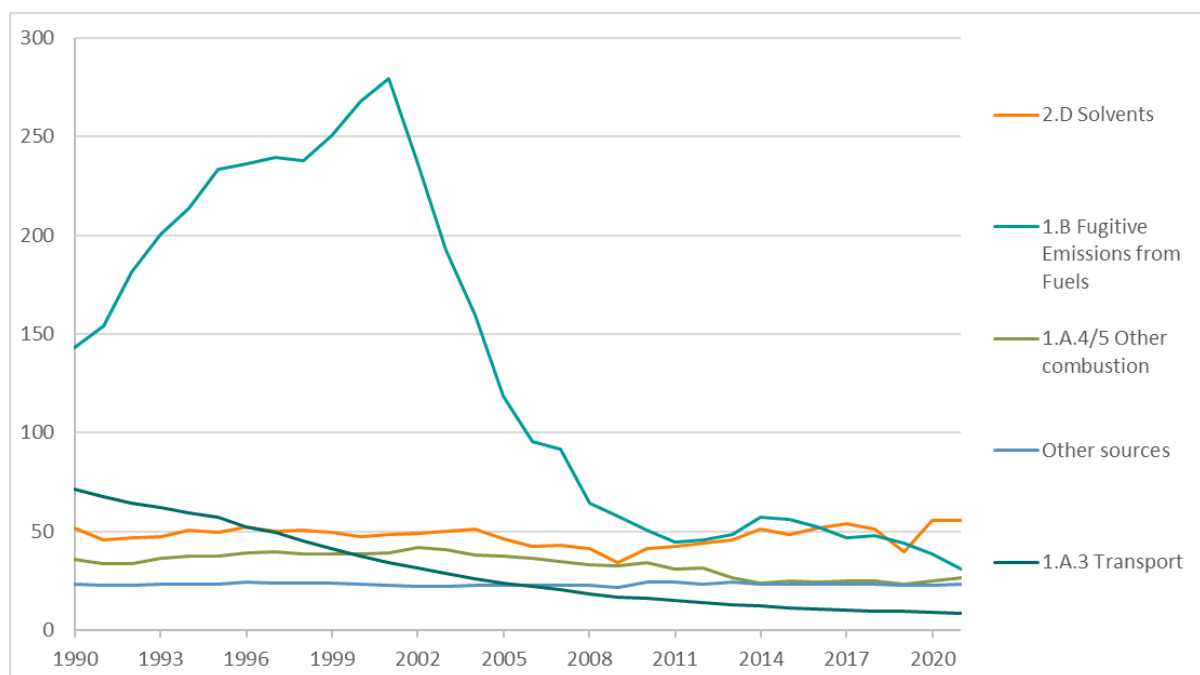
Figure 2.8. Trends in NMVOC emissions, 1990-2021. 1000 tonnes
