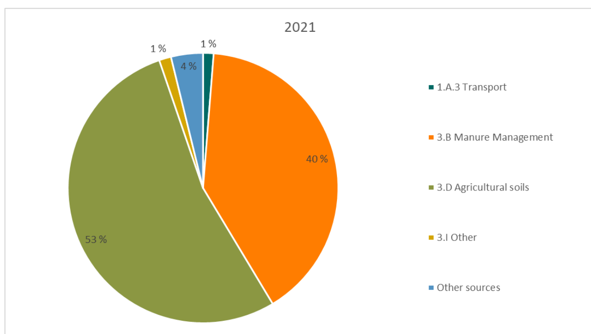
Figure 2.7. Distribution of NH 3 emissions between emission sources, 2021. Per cent
