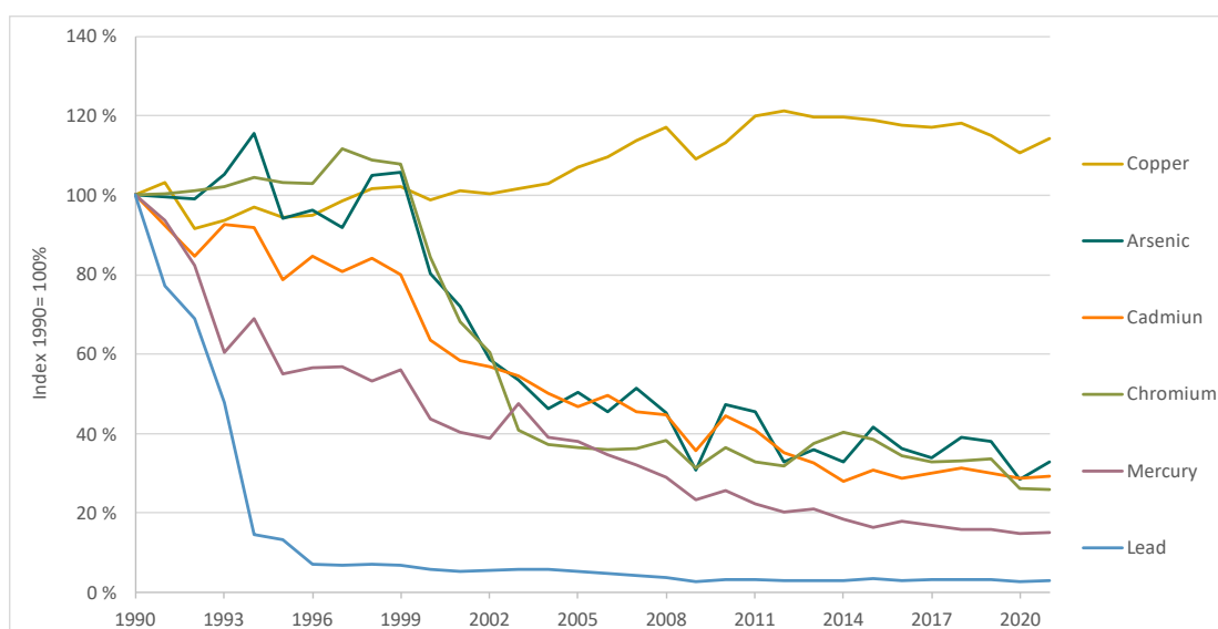
Figure 2.13 Trends in emissions for Heavy metals. 1990-2021. Index 1990=100%
