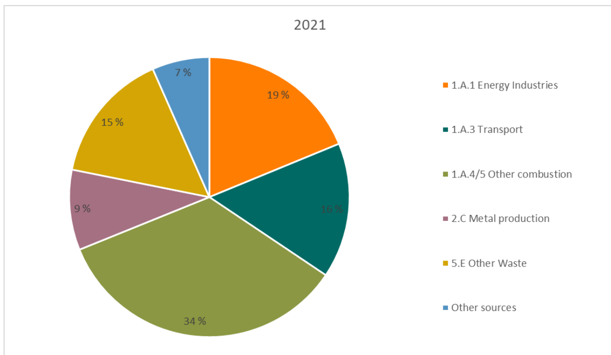
Figure 2.20. Distribution of dioxins emissions between emission sources, 2021. Per cent
