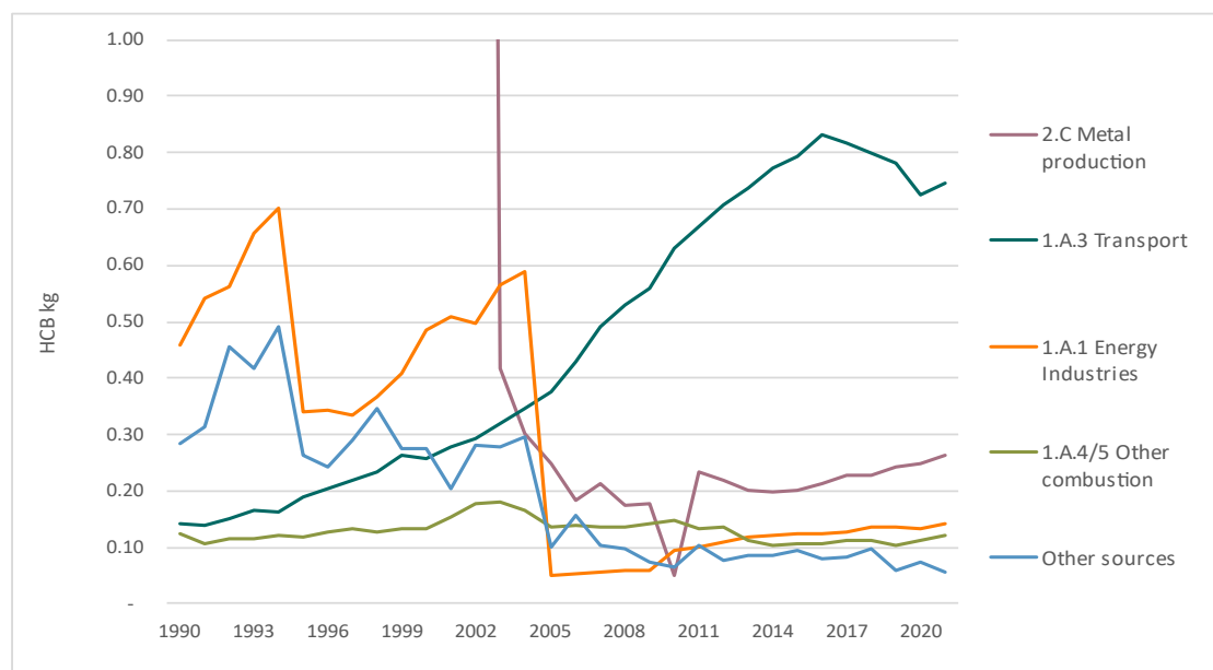
Figure 2.25. Trends in total HCB emissions, 1990-2021. Kilogram
