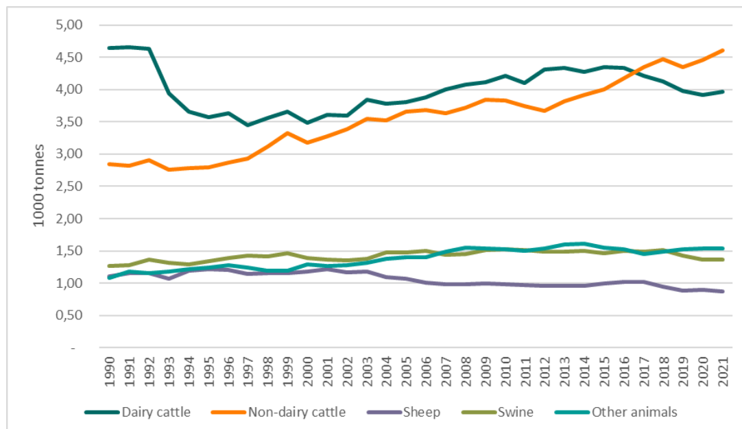
Figure 5.3 Trends for the NH 3 emissions from manure management. 1000 tonnes NH 3 . 1990-2021. Source: Statistics Norway/ Norwegian Environment Agency
