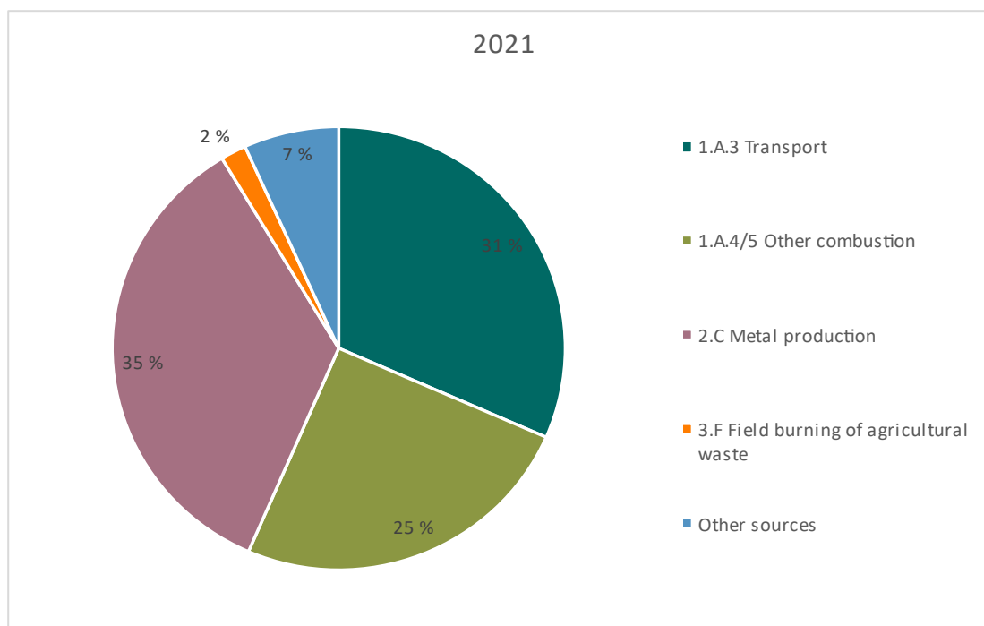
Figure 2.23. Distribution of total PAH-4 emissions between emission sources, 2021. Per cent
