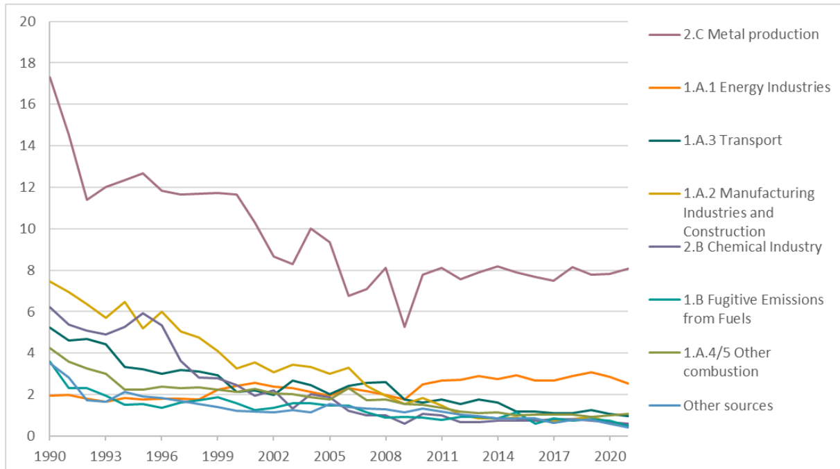
Figure 2.4. Trends in SO 2 emissions, 1990-2021. 1000 tonnes
