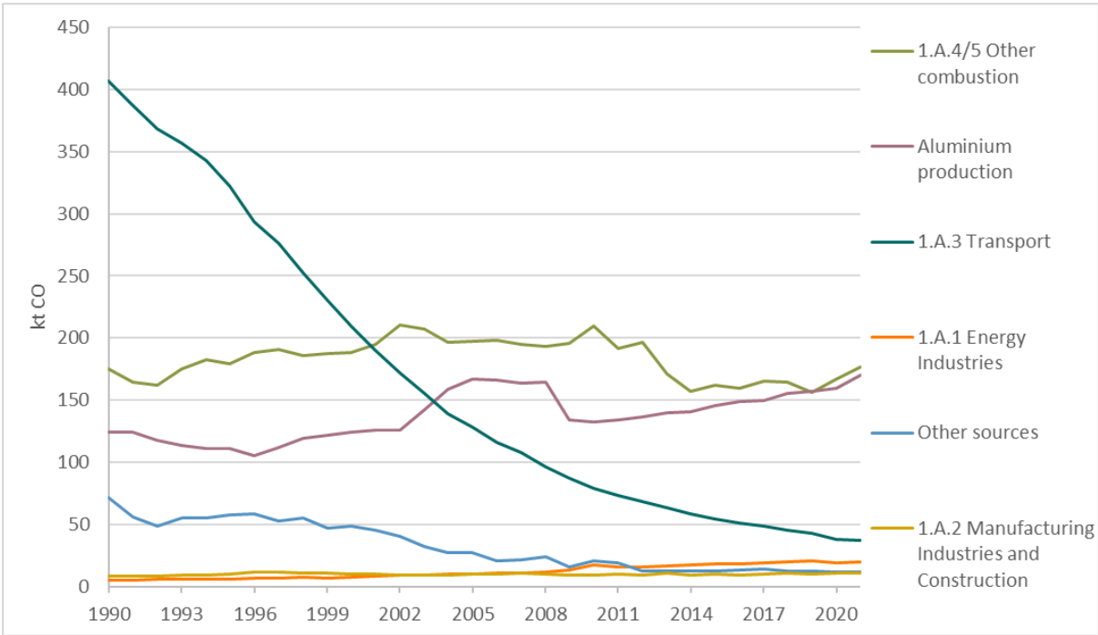
Figure 2.10. Trends in CO emissions, 1990-2021. 1000 tonnes Source: Statistics Norway/Norwegian Environment Agency
