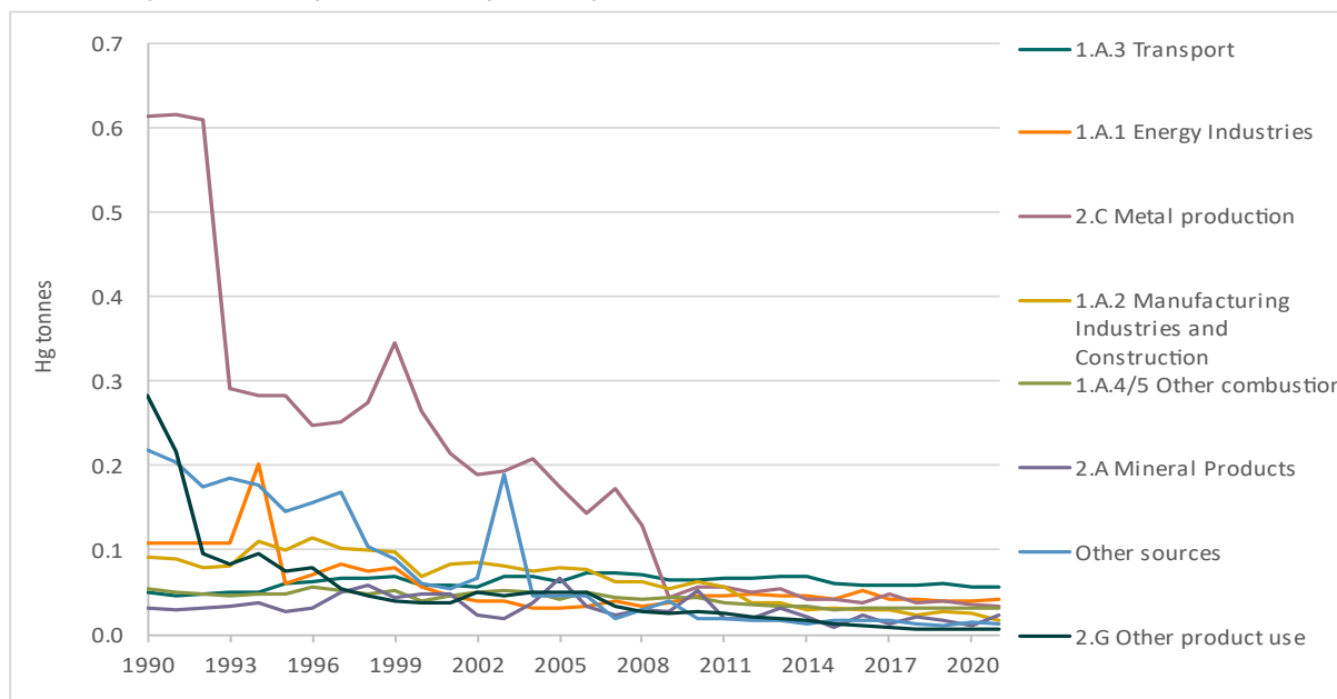
Figure 2.34. Trends in mercury emissions, 1990-2021. Tonnes
