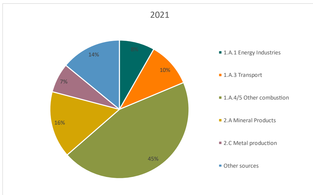
Figure 2.15. Distribution of PM 10 emissions between emission sources, 2021. Per cent
