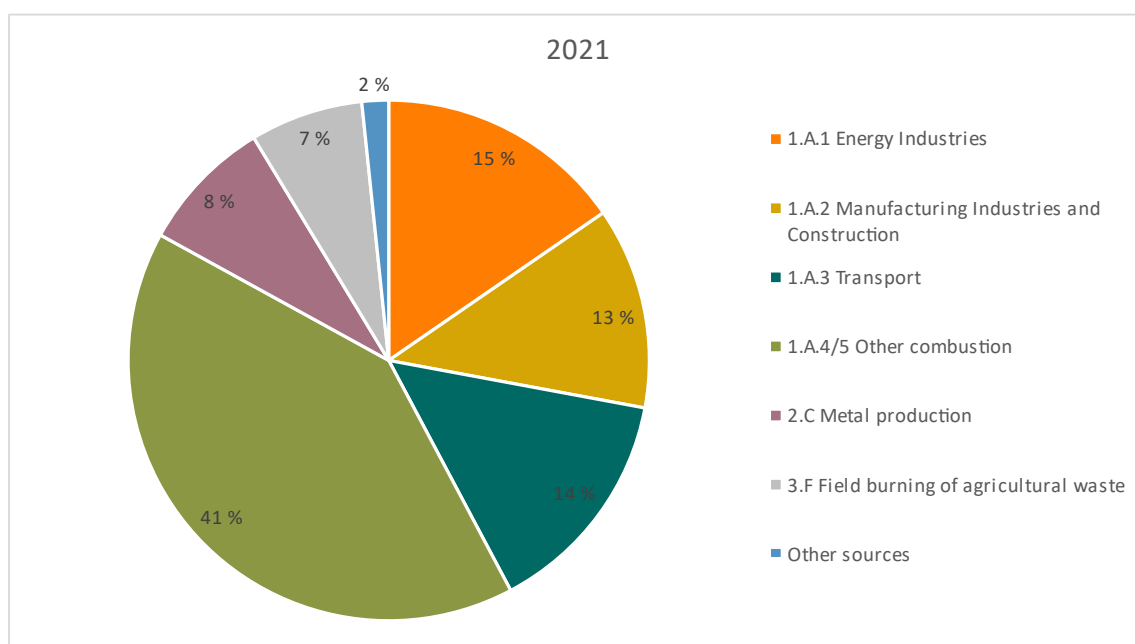
Figure 2.33. Distribution of cadmium emissions between emission sources, 2021. Per cent
