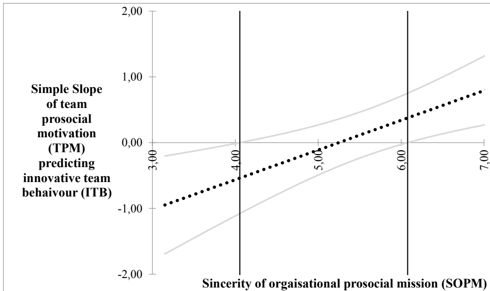
Figure 3: Johnson Newman graph
