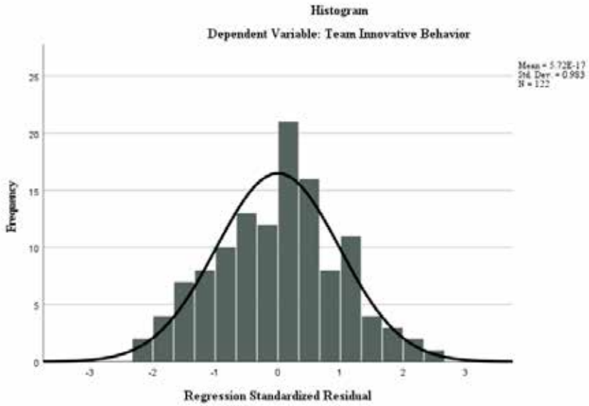
Figure 4: Normality distribution
