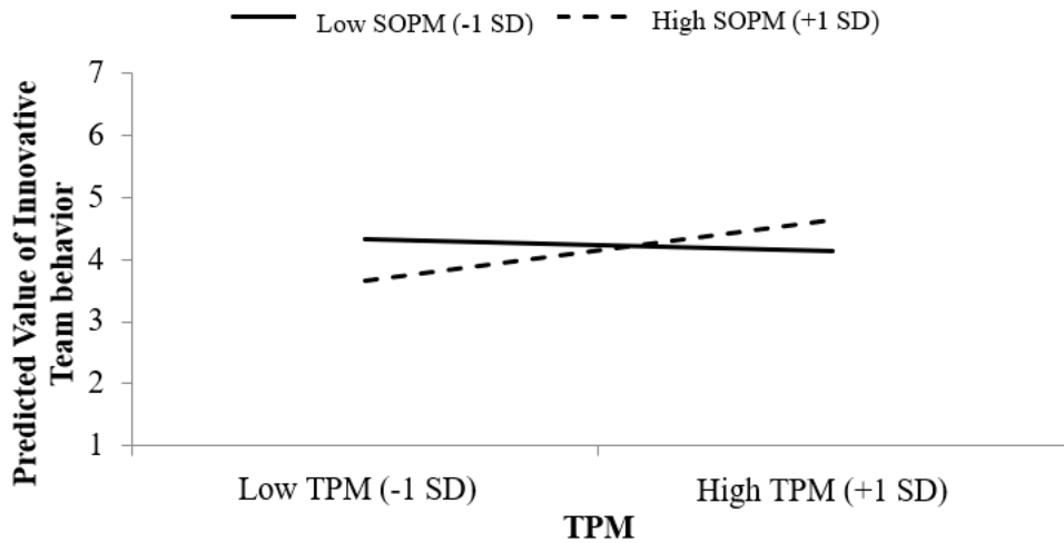
Figure 2: Plot of simple slopes
