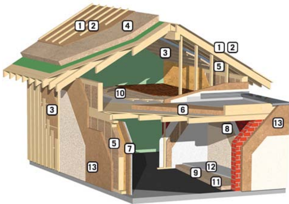
Figure 5.1 Applications for wood fibre insulation boards. The numbers indicate different product qualities adapted for the applications (Gutex, 2011).
