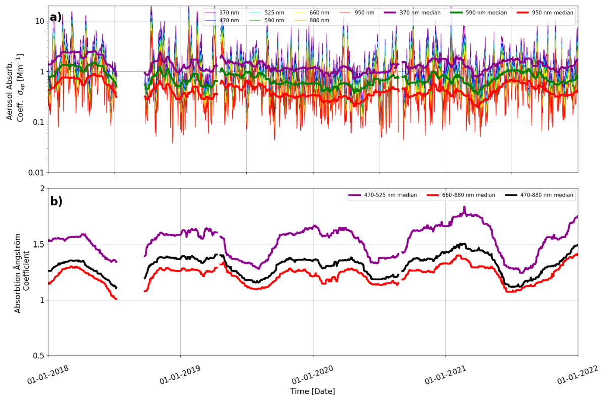
Figure 44: Time series of aerosol particle absorption coefficient \sigma_{ap} (top) and the absorption Ångström coefficient \tilde{a}_{ap} (bottom), both daily means, measured by the filter absorption photometer deployed at Birkenes in November 2017. The time series covers the years 2018 - 2021.
