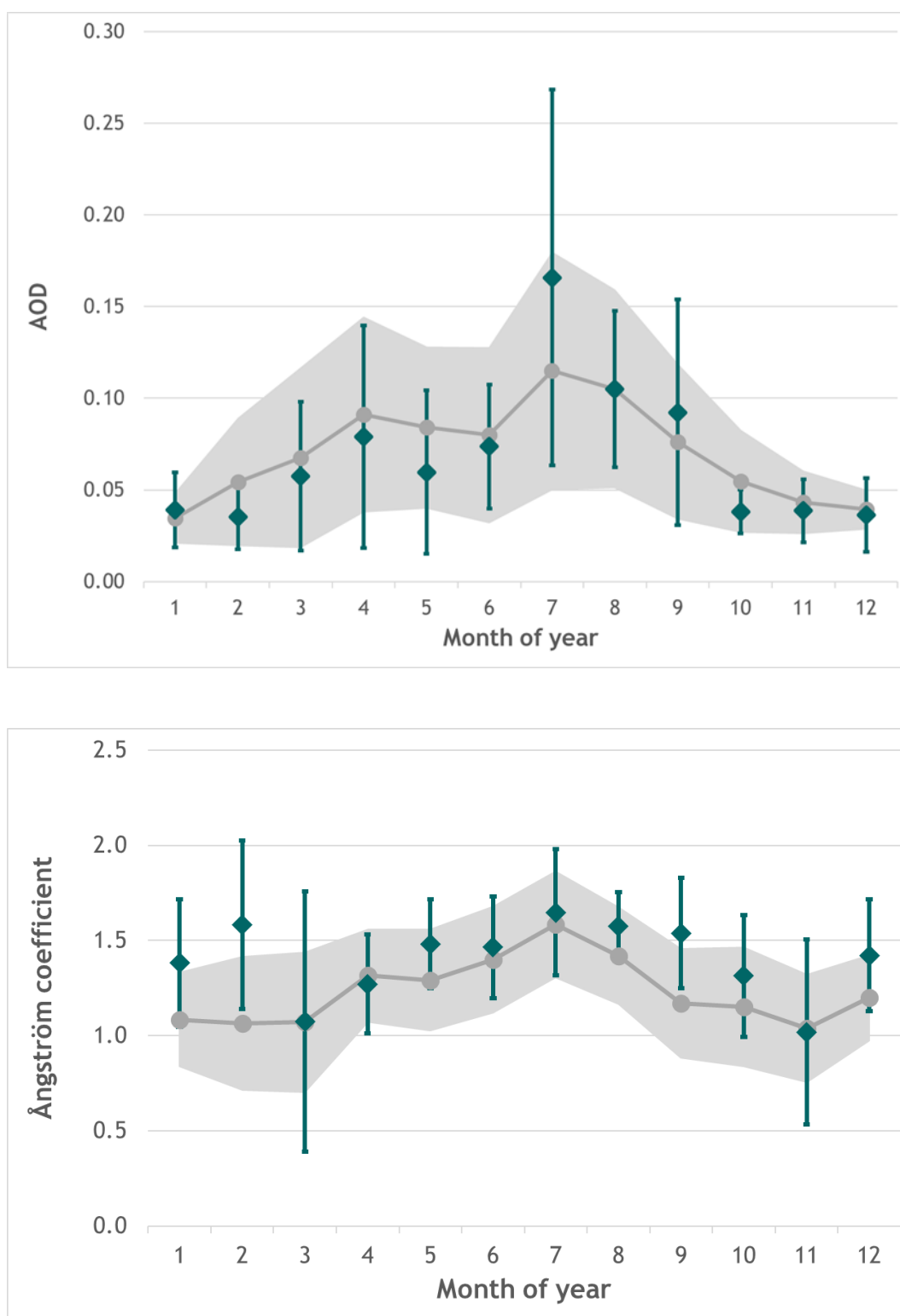
Figure 57: 2021 monthly mean aerosol optical depth (AOD) at 500 nm wavelength in the atmospheric column above Birkenes (upper panel) and (470, 800 nm) Ångström coefficient describing the AOD wavelength dependence (lower panel). Mean values and standard deviations are given. Values marked in grey are the mean and standard deviations for the 2009-2021.
