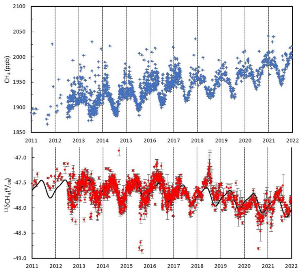
Figure 12: Long term measurements of methane concentration (CH 4 , blue) and the 13 C isotopic signature of CH 4 (δ 13 C-CH 4 , red) at the Zeppelin Observatory, Svalbard 78°N.
