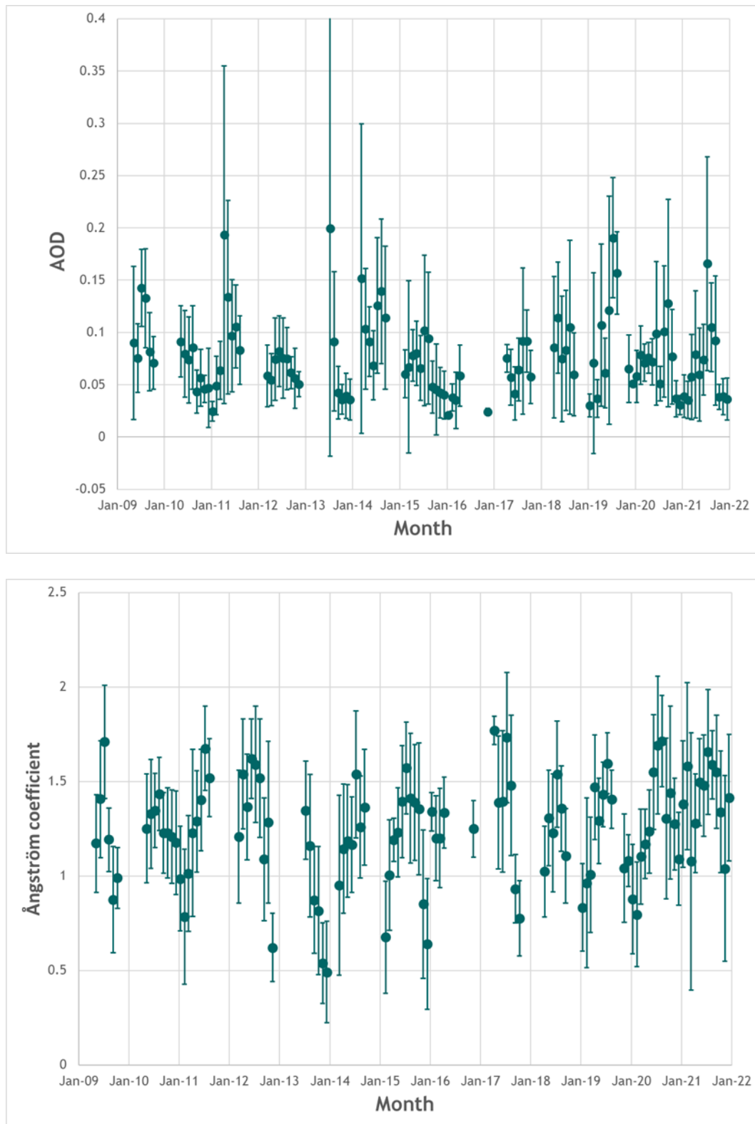
Figure 56: 2009 - 2021 time series of aerosol optical depth (AOD) at 500 nm wavelength in the atmospheric column above Birkenes (upper panel) and (470 nm, 800 nm) Ångström exponent describing the AOD wavelength dependence (lower panel). Monthly mean values and standard deviations are given.
