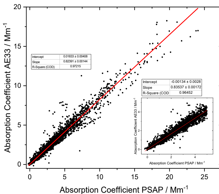
Figure 60: Comparison of particle absorption coefficient data measured the Particle Absorption Photometer (PSAP) deployed at Birkenes in 2012, and the AE33 aethalometer deployed there in 2017. The wavelength of the absorption coefficient has been interpolated to 550 nm for both instruments. The data are compared as scatter plot with regression line (red), large panel for the total range of values, small panel for values \leq 5 \text{ Mm}^{-1} .
