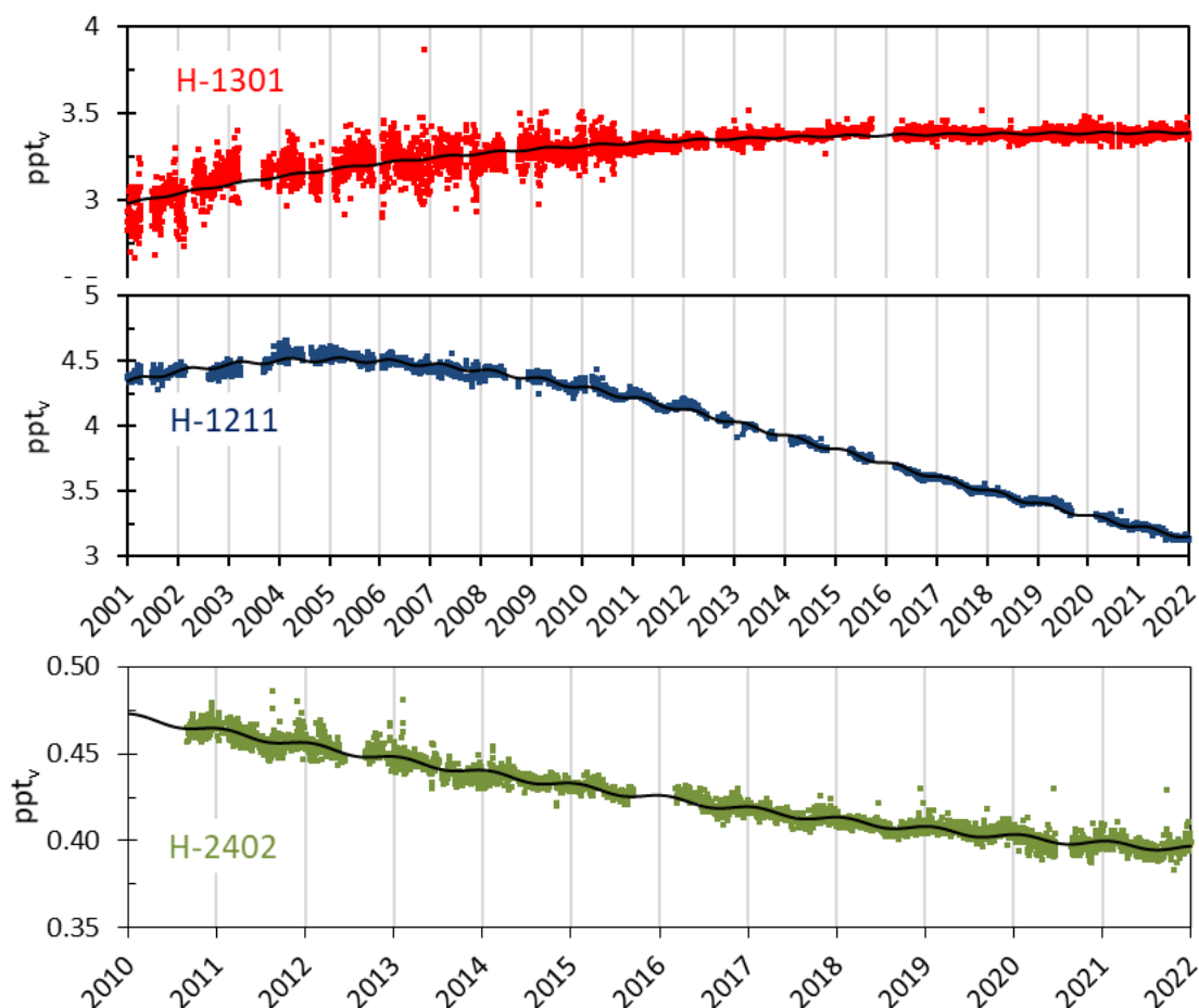
Figure 33: Daily averaged concentrations of the monitored halons at the Zeppelin Observatory. For the period 2001-2021: H-1301 (red) and H-1211 (blue). For the period 2010-2021: H-2402 (green). The solid lines are empirical fitted mixing ratios.
