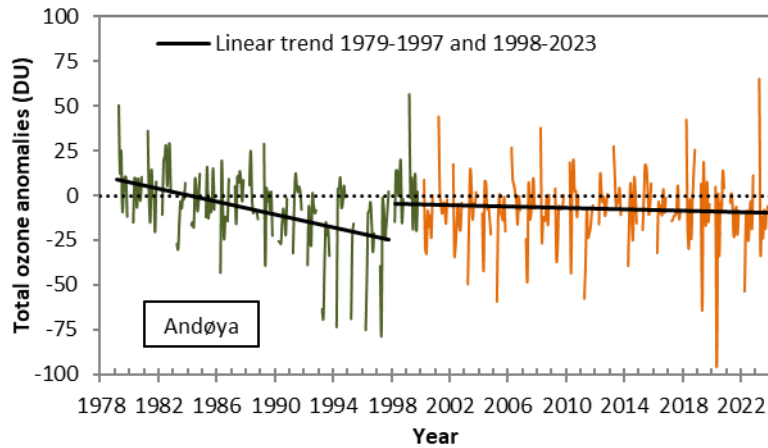
Figure 5b: Variations in total ozone at Andøya for the period 1979 to 2023 after the seasonal variations are removed. Only data for the months March to October are included. The green line represents total ozone from Tromsø, whereas the orange line represents measurements at Andøya. The trends are marked as black lines.
