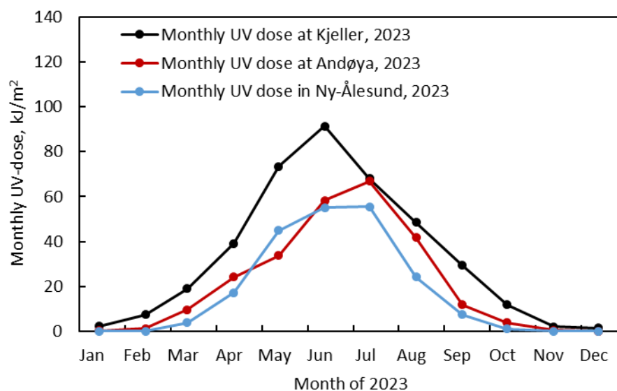
Figure 17: Monthly integrated UV doses (in kJ/m²) in 2023 measured with the GUV instruments located at Kjeller, Andøya and in Ny-Ålesund.
