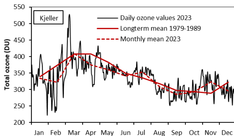
Figure 1: Daily total ozone values measured at Kjeller in 2023 (black curve). The red curve shows the long-term monthly mean values from Oslo 1979 to 1989. The red dashed line is monthly mean ozone values in 2023.
