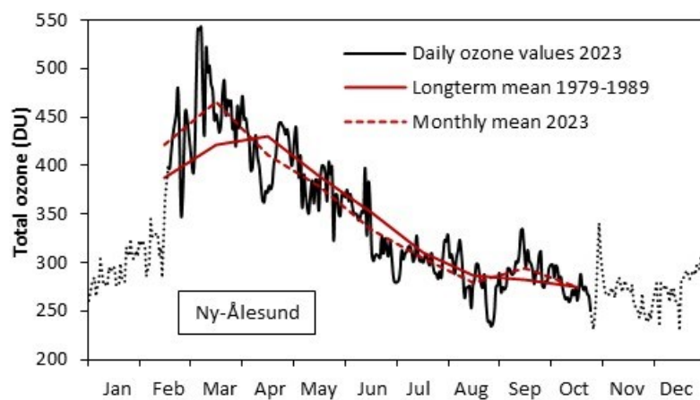
Figure 3: Daily total ozone values measured in Ny-Ålesund in 2023 by the SAOZ and GUV instruments (black curve). The red line is the long-term monthly mean values from 1979 to 1989, whereas the dashed red line is monthly mean values for 2023. The black dotted line represents GOME-2B satellite measurements.
