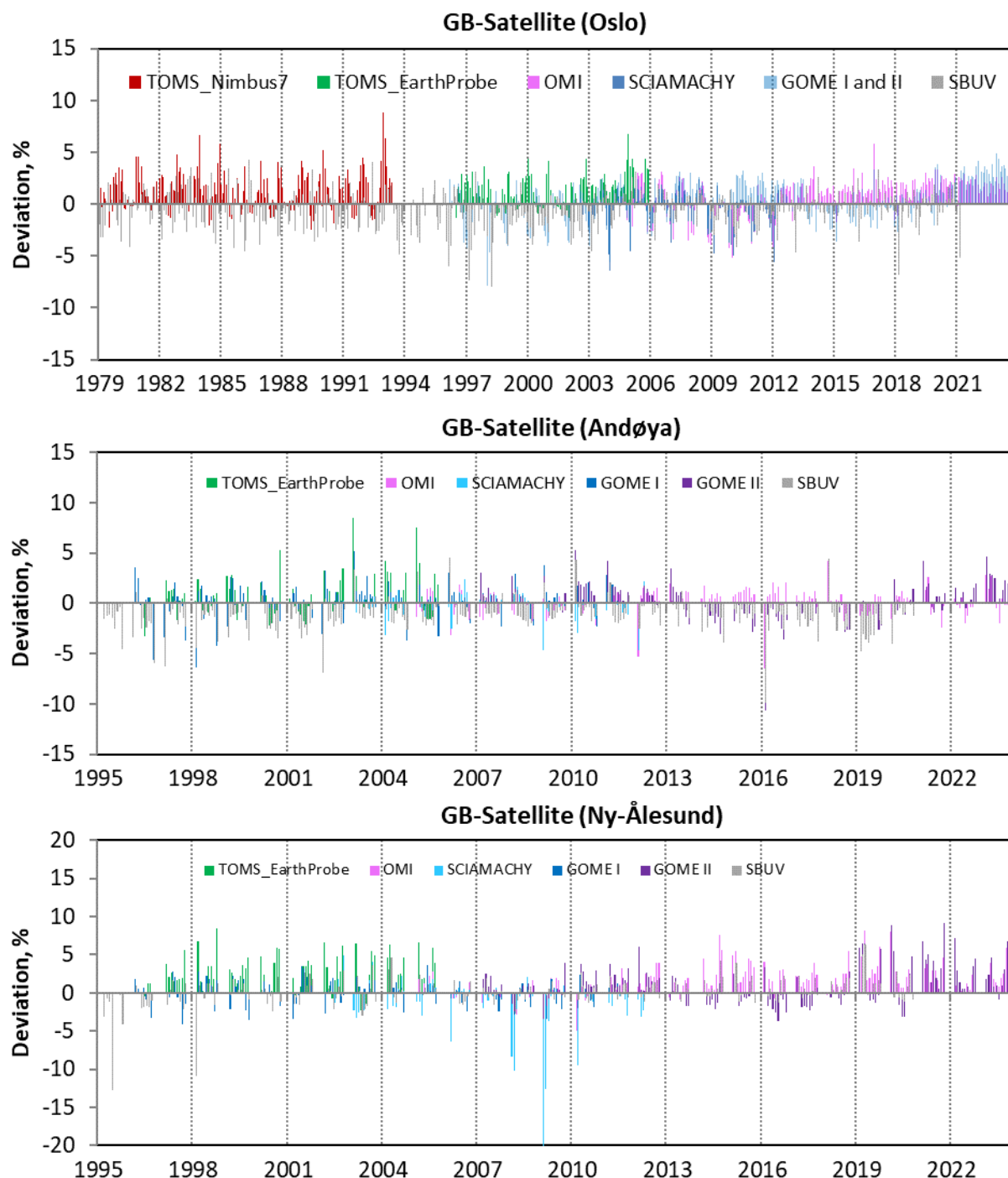
Figure 12: Difference between ground-based (GB) and satellite retrieved monthly mean ozone values from 1979 to 2023 (Oslo/Kjeller) and 1995 to 2023 (Andøya and Ny-Ålesund). Deviations are given in %. Upper panel: Oslo/Kjeller, middle panel: Andøya, lower panel: Ny-Ålesund.
