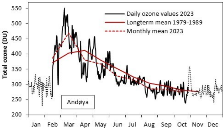
Figure 2: Daily total ozone values measured at ALOMAR, Andøya, in 2023 by the Brewer and GUV instruments (black curve). The red line is the long-term monthly mean values from 1979-1989, whereas the red dashed line is monthly mean ozone values in 2023. The black dotted line represents GOME-2B satellite measurements.
