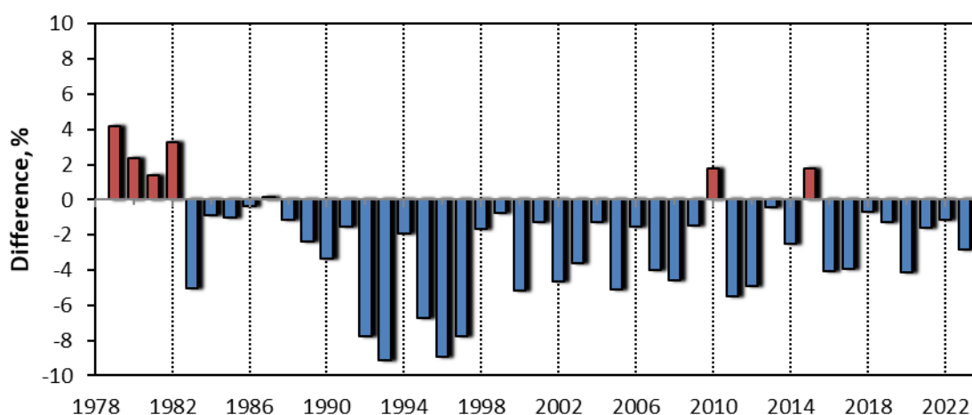
Figure 7: Percentage difference between yearly mean total ozone in Oslo/Kjeller and the long-term yearly mean 1979 to 1989. Red numbers represent positive differences, whereas blue numbers are negative differences.
