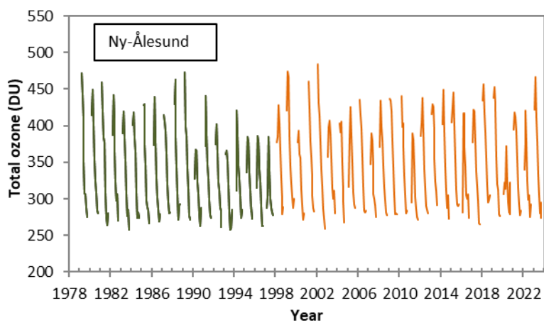
Figure 6a: Time series of monthly mean total ozone at Ny-Ålesund 1979 to 2023. The green line represents total ozone data from satellite, whereas the orange line represents measurements from ground-based instruments.
