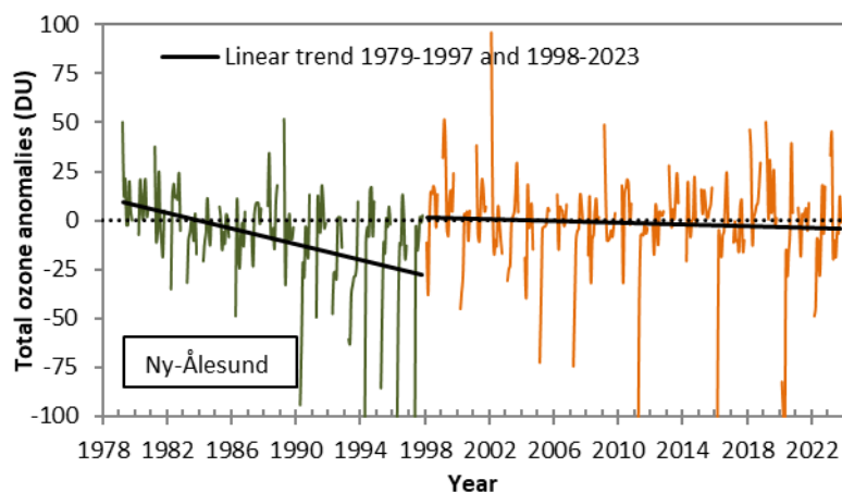
Figure 6b: Variations in total ozone at Ny-Ålesund for the period 1979 to 2023. Only data for the months March to October are included. The green line represents total ozone data from satellite, whereas the orange line represents measurements from ground-based instruments. Trends for the two periods are marked as black lines.
