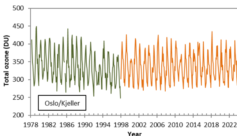
Figure 4a: Time series of monthly mean total ozone in Oslo and at Kjeller 1979 to 2023. The green line represents measurements performed with the Dobson instrument, whereas the orange line represents Brewer measurements.
