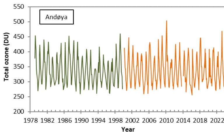
Figure 5a: Time series of monthly mean total ozone at Andøya and Tromsø 1979 to 2023. The green line represents total ozone from Tromsø, whereas the orange line represents measurements at Andøya.
