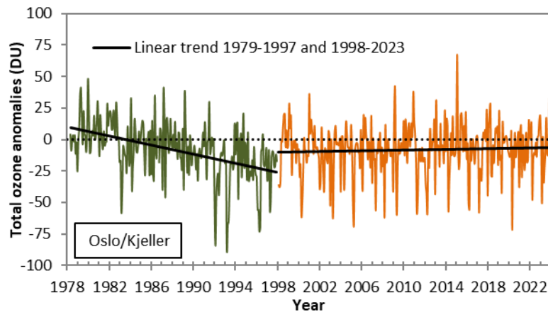
Figure 4b: Variation in total ozone over Oslo/Kjeller for the period 1979 to 2023 after the seasonal variations have been removed. The green line represents measurements performed with the Dobson instrument, whereas the orange line represents Brewer measurements. Trend lines are marked as black lines.
