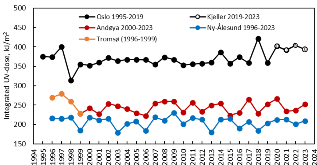
Figure 18: Annual integrated UV doses (in kJ/m 2 ) in Oslo, at Andøya/Tromsø and in Ny-Ålesund for the period 1995–2023.
