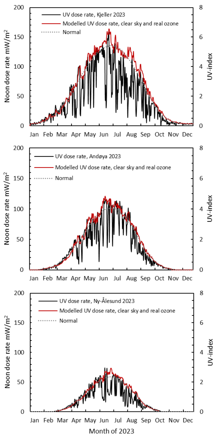
Figure 15: Hourly averaged UV dose rate measured at local noon ( \pm 0.5 hour) in 2023. Upper panel: Kjeller. Middle panel: Andøya. Lower panel: Ny-Ålesund.
