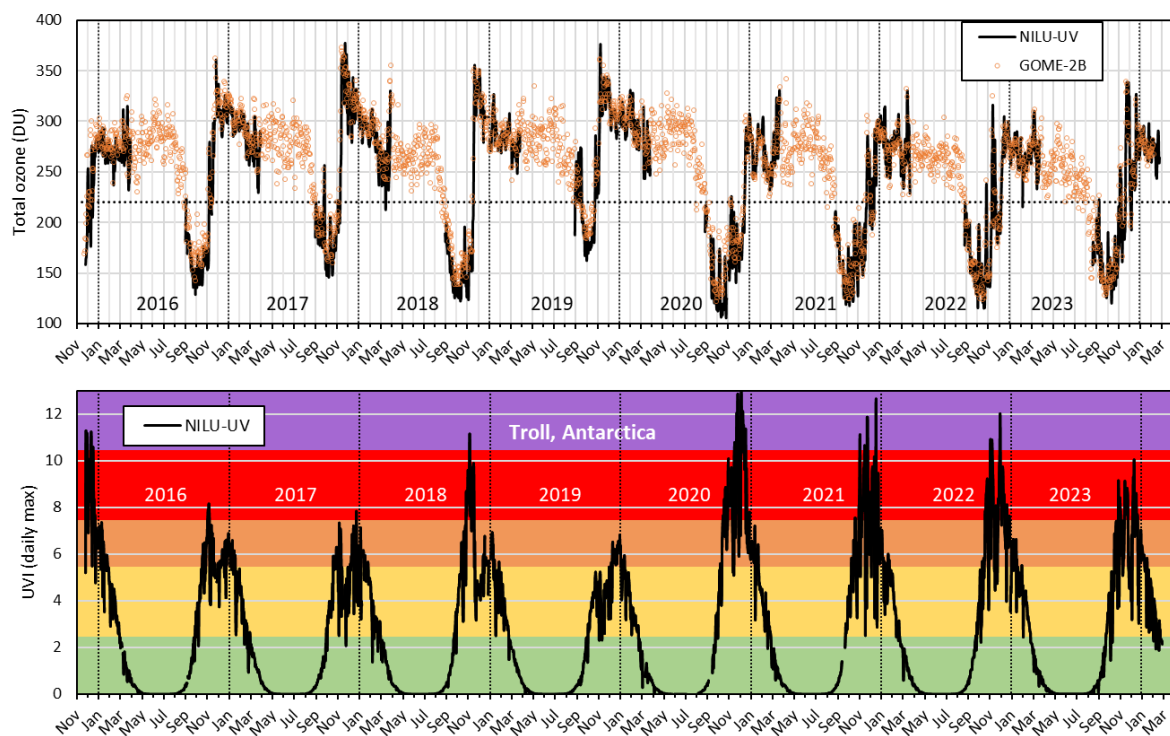
Figure 10: Upper panel: Total ozone from NILU-UV and GOME-2B from November 2015 to March 2024. Lower panel: Noon time UVI from NILU-UV for the same period. The green, yellow, orange, red, and ultraviolet colours represent the UVI categories low, moderate, high, very high, and extreme, respectively)
