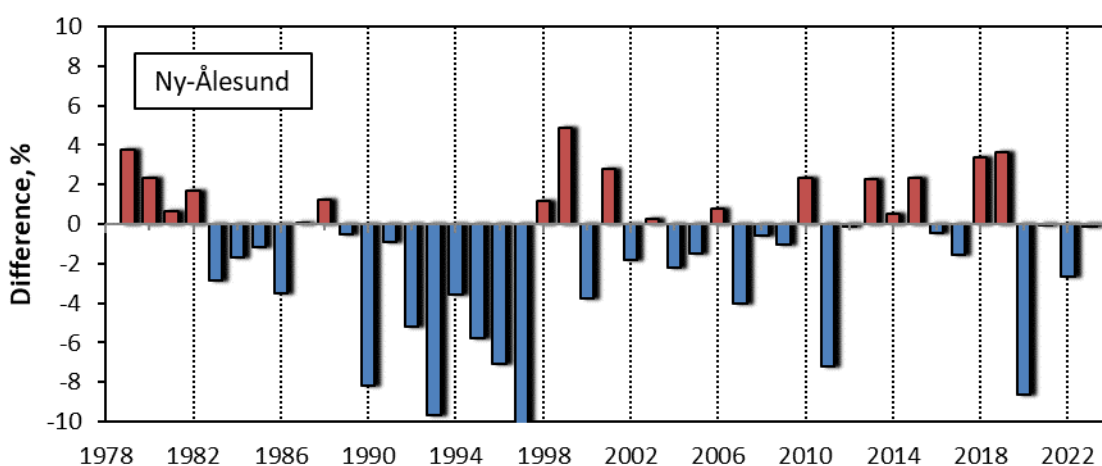
Figure 9: Percentage difference between yearly mean total ozone in Ny-Ålesund and the long-term yearly mean 1979-1989 for the months March-October.
