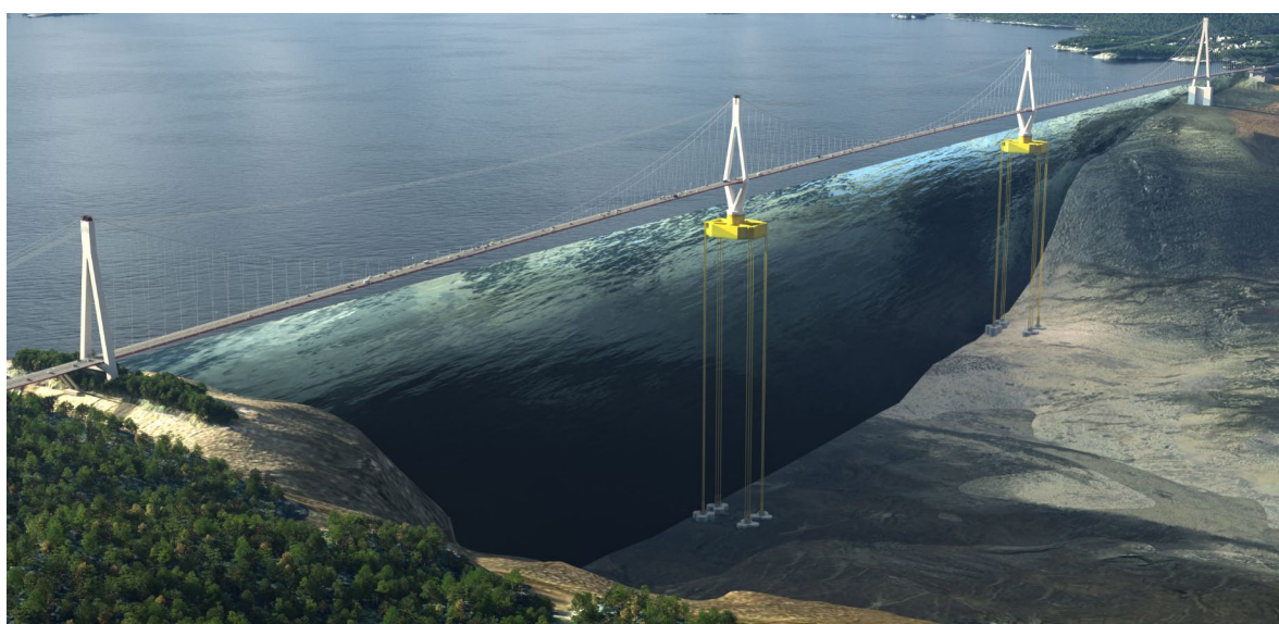
Figure 5. Suspension bridge on TLP for Bjørnafjord – underwater view (from Statens Vegvesen).
