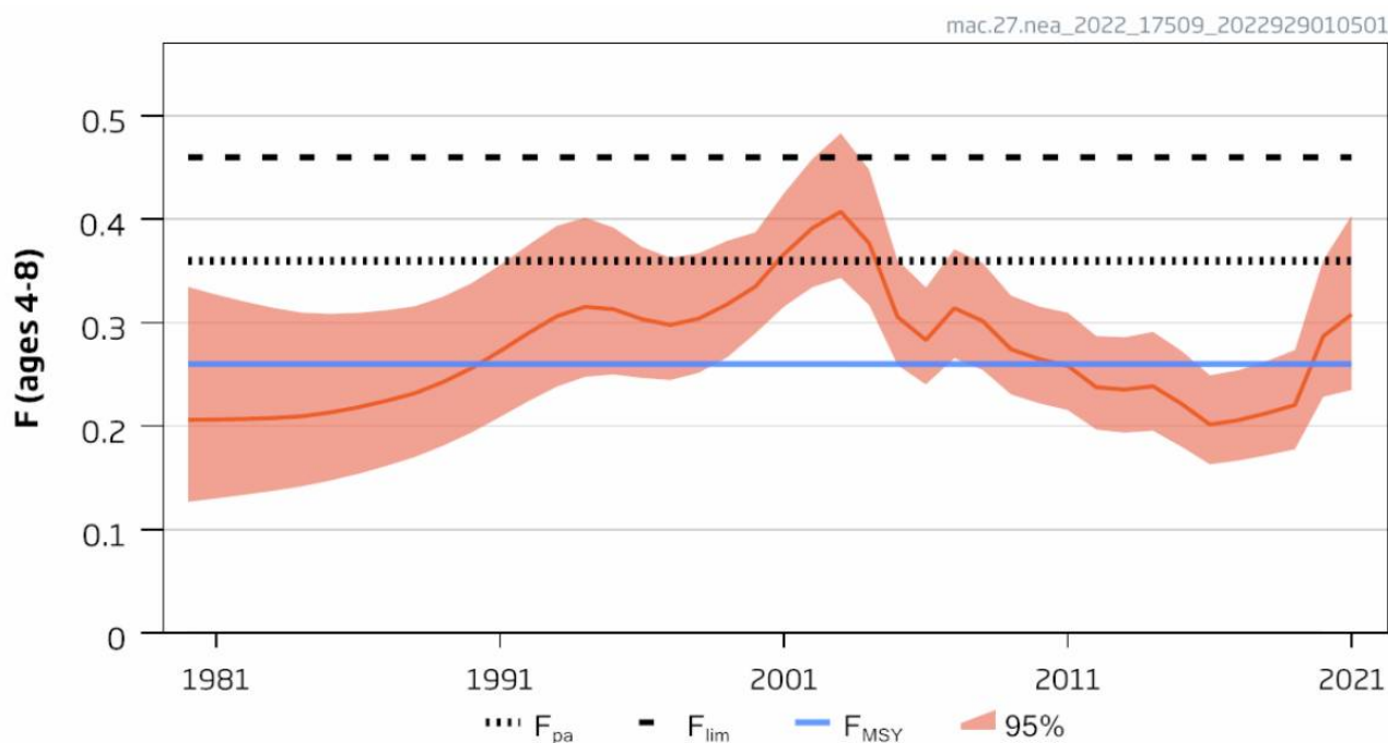
Figure 7.3.4 Fishing mortality of mackerel in the Northeast Atlantic and adjacent waters for ages 4-8 years indicated by the red line with 95% confidence intervals indicated by the red shaded area. The reference points F_{pa} (precautionary reference point for fishing mortality), F_{lim} (a critical threshold of fishing mortality, above which recruitment overfishing and stock collapse is possible) and F_{MSY} (fishing mortality consistent with achieving maximal sustainable yield) are indicated by horizontal lines. Source: ICES (2022c).
