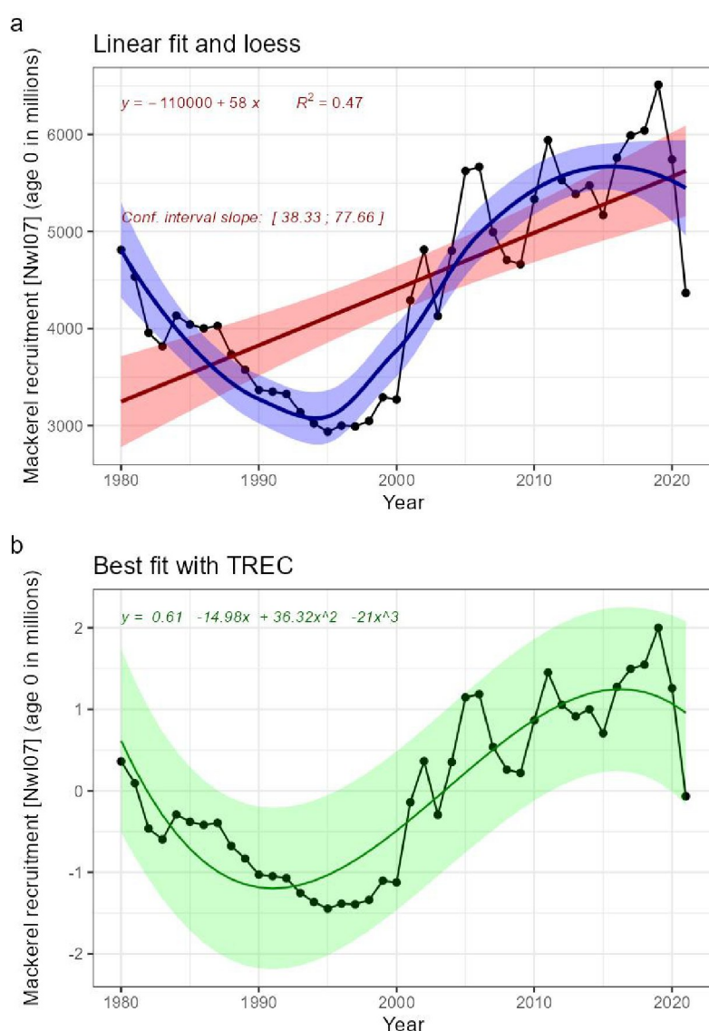
Fig.7.1: Indicator time series and fitted trends. A) linear trend fitted with Least-square method (not adapted for short time series) in red, and loess in blue, for information. B) Best fitted trend using the first steps of a TREC analysis on scaled time series
