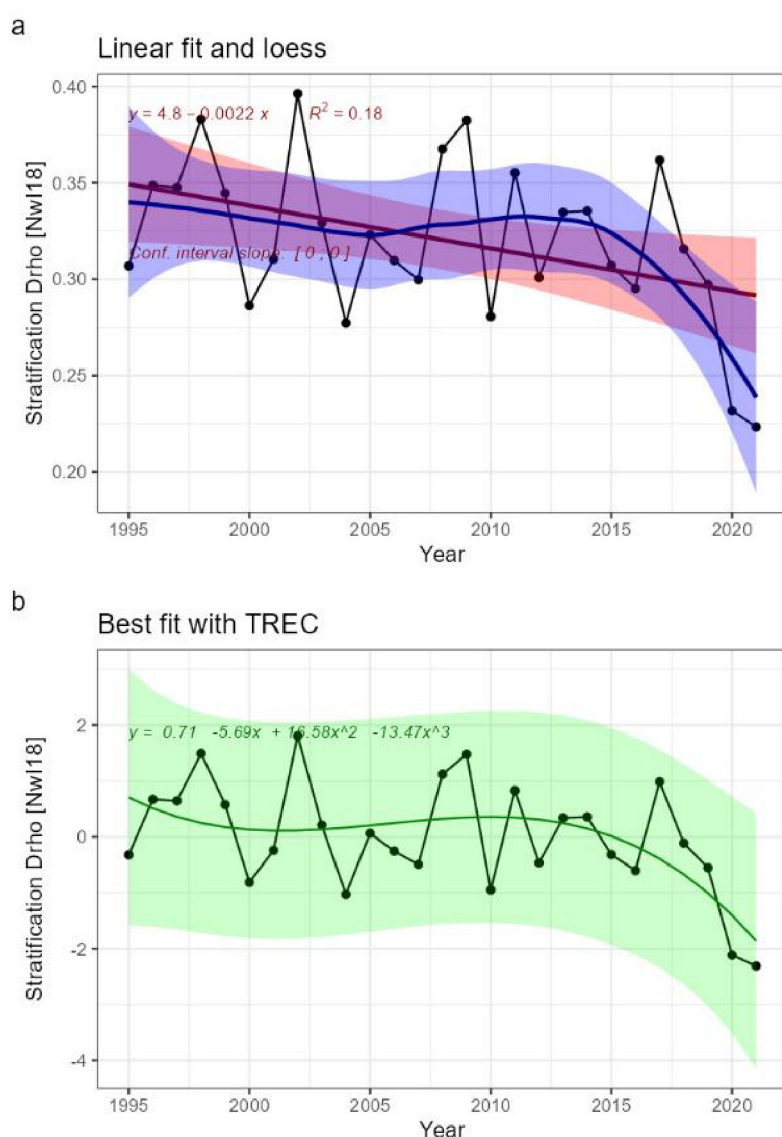
Fig.18: Indicator time series and fitted trends. A) linear trend fitted with Least-square method (not adapted for short time series) in red, and loess in blue, for information. B) Best fitted trend using the first steps of a TREC analysis on scaled time series
