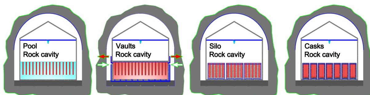
Figure 4-12. Rock cavern.
