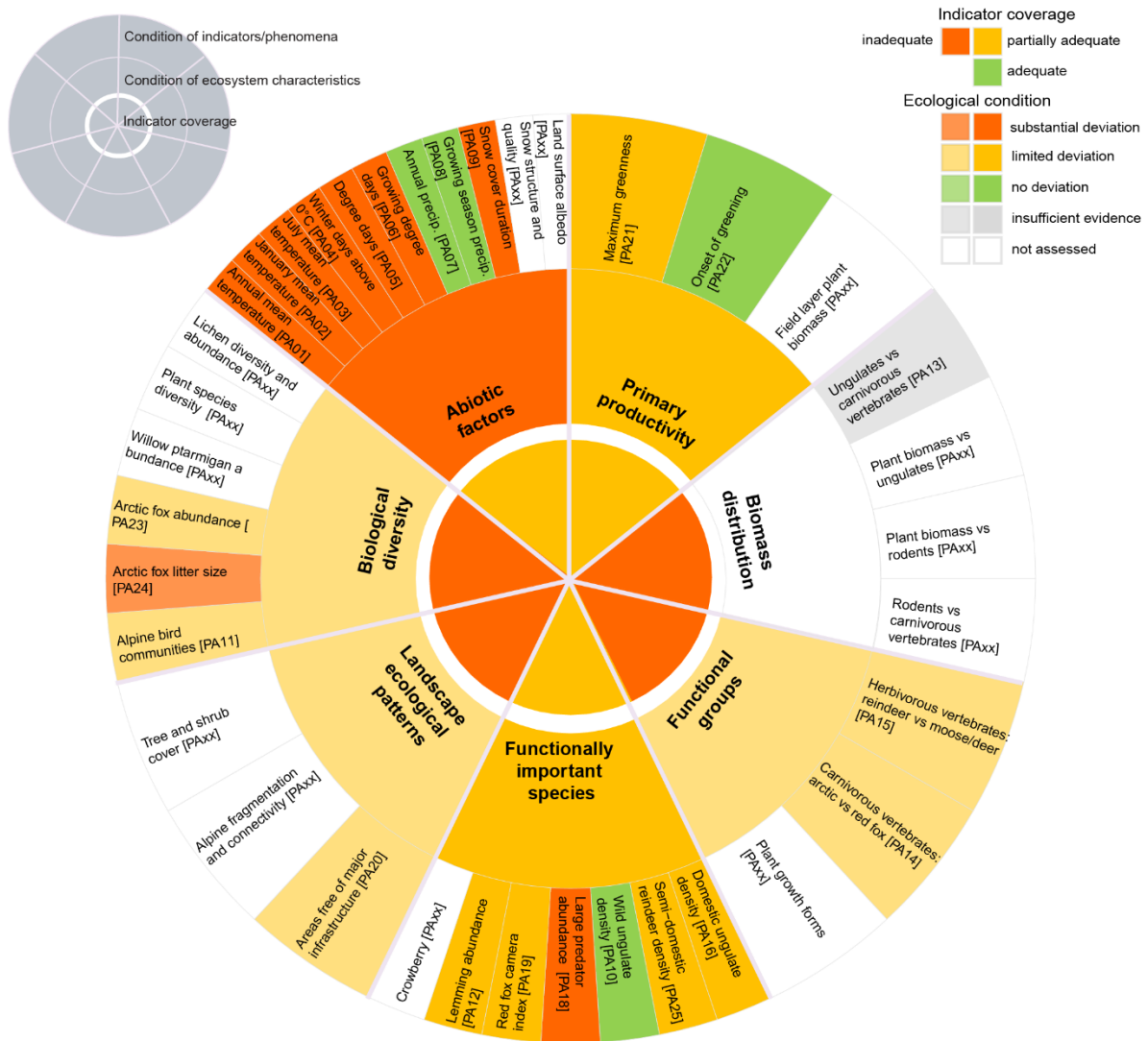
Figure 7.3.2. A graphical summary of the assessment of ecological condition of alpine ecosystems. The outer ring shows the assessment of ecological condition at the level of the individual indicators with associated phenomena ID in square brackets. Indicators which the scientific panel have recommended for inclusion ( Table 7.7 ), but which are not included in the pilot assessment, are shown in white to illustrate the perceived most important deficiencies in the current indicator set. The middle ring shows the assessment at the level of ecosystem characteristics, indicating deviation from the reference condition, and the innermost circle shows the quality of indicator coverage. Assessment based on inadequate indicator coverage is further highlighted by paler shading in ecological characteristics and their corresponding indicators.
