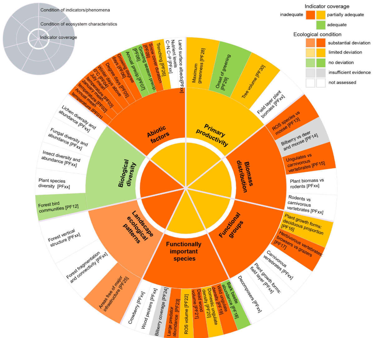
Figure 7.2.2. A graphical summary of the assessment of ecological condition of forest ecosystems. The outer ring shows the assessment of ecological condition at the level of the individual indicators with associated phenomena ID in square brackets. Indicators which the scientific panel have recommended for inclusion (Table 7.7), but which are not included in the pilot assessment, are shown in white to illustrate the perceived most important deficiencies in the current indicator set. The middle ring shows the assessment at the level of ecosystem characteristics, indicating deviation from the reference condition, and the innermost circle shows the quality of indicator coverage. Assessment based on inadequate indicator coverage is further highlighted by paler shading in ecological characteristics and their corresponding indicators.
