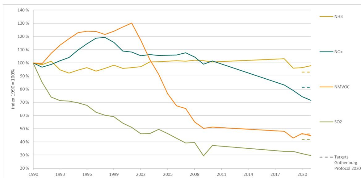
Figure 2.1. Trends in emissions for \text{NO}_x , \text{SO}_2 , \text{NH}_3 and NMVOC. 1990-2021. Index 1990 = 100%
