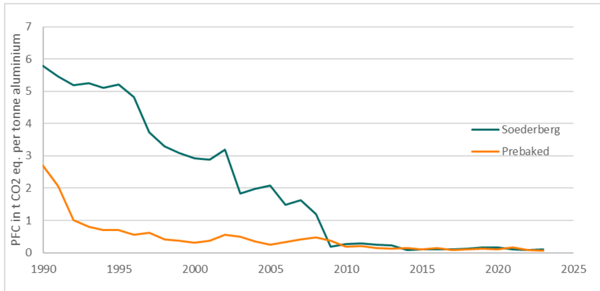
Figure 4.5: PFC in tonne CO 2 equivalent per tonne primary aluminium. Source: Norwegian Environment Agency.
