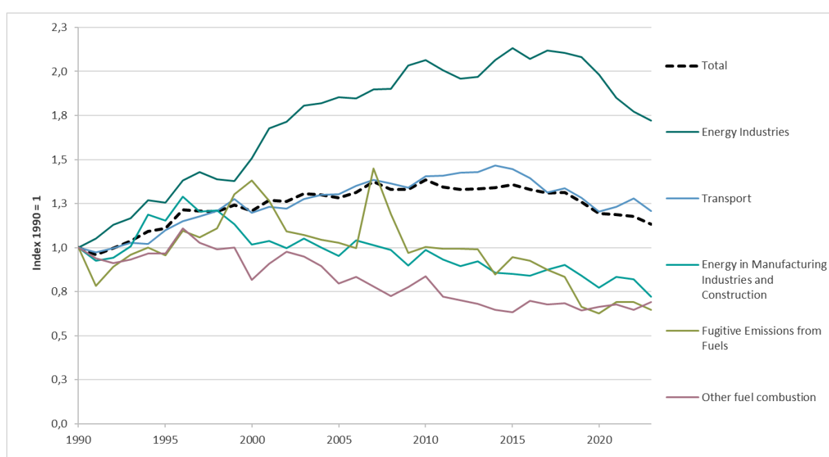
Figure 2.6: Development in emissions of greenhouse gases, relative to 1990, for the main sub-sectors within the energy sector, 1990-2023. Index 1990 = 1. Source: Statistics Norway/Norwegian Environment Agency.
