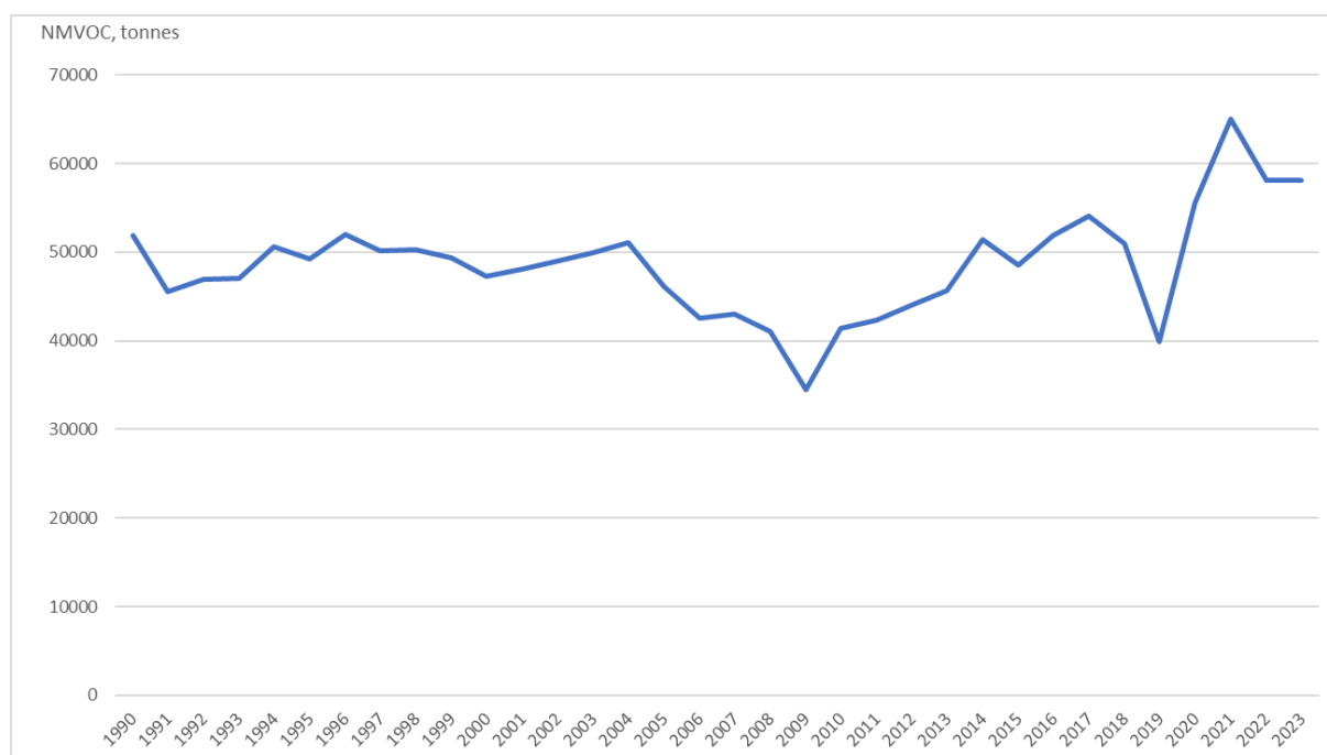
Figure 4.6: Emissions from solvent use illustrating inter-annual changes, emissions in tonnes NMVOC. Source: Statistics Norway.
