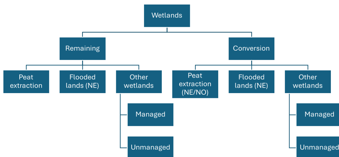
Figure 6.29: Reporting structure under Wetlands. The notation key NE “not estimated” is used for flooded land as reporting is not mandatory for this category. The notation key NO means “not occurring”, which is the case of peat extraction in mineral soils.
