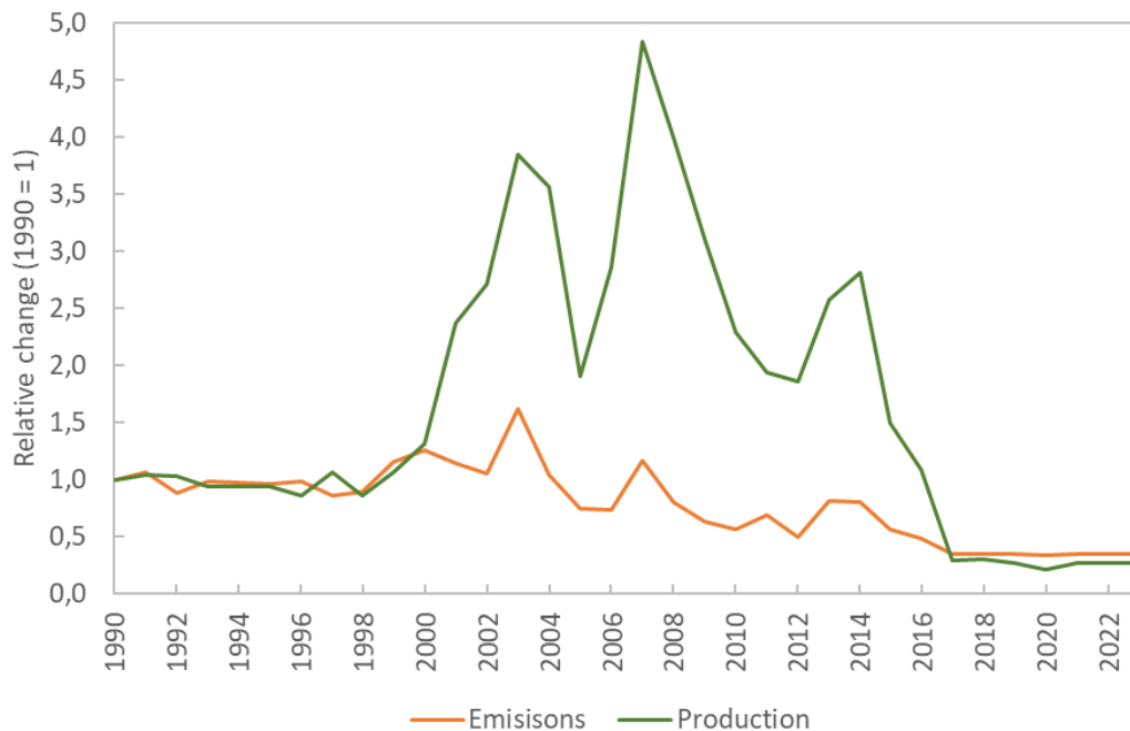
Figure 3.16: Relative change in coal production in Norway and related GHG emissions. Excluding emissions from abandoned underground mines. 1990=1.
