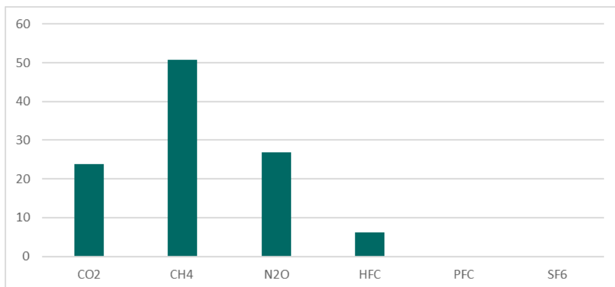
Figure 10.3: Difference in total emissions for 2022 per gas, excluding LULUCF, between latest and previous submission. 1000 tonnes CO 2 equivalents.
