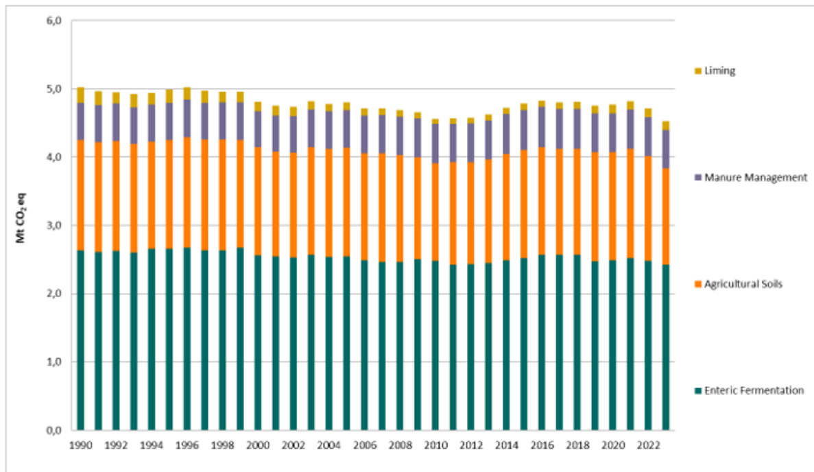
Figure 2.9: Total greenhouse gas emissions (Mtonnes CO 2 eq.) in the agriculture sub-sectors in Norway, 1990-2023. Source: Statistics Norway/Norwegian Environment Agency.
