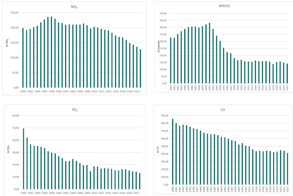
Figure 2.24: Emissions (ktonnes) of NO x , NMVOC, SO 2 , and CO in Norway, 1990-2023. Source: Statistics Norway/ Norwegian Environment Agency.
