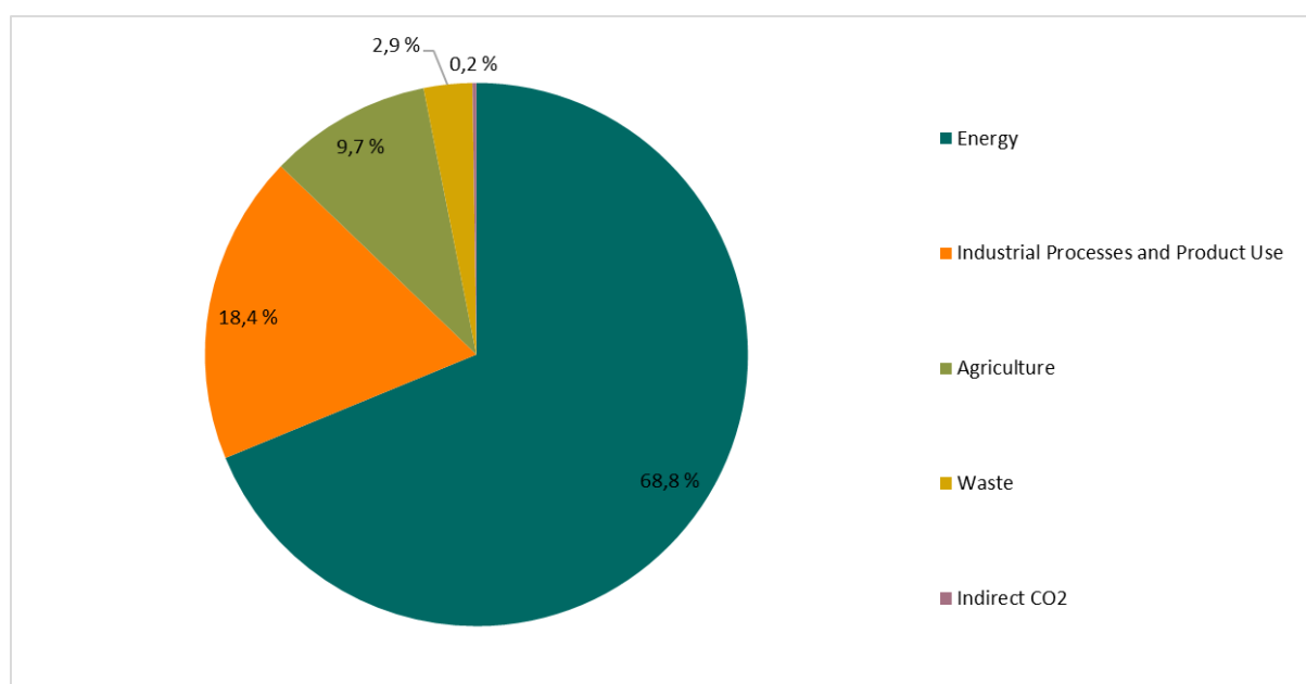
Figure 2.3: Distribution of GHG emissions (without LULUCF) in Norway in 2023 by sector. Indirect CO 2 emissions is also shown. Source: Statistics Norway/Norwegian Environment Agency.
