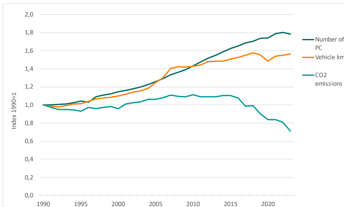
Figure 3.14: Relative change to 1990 in number of passenger cars, CO 2 emissions and vehicle kilometres. Index 1990=1. Source: Statistics Norway/Norwegian Environment Agency.
