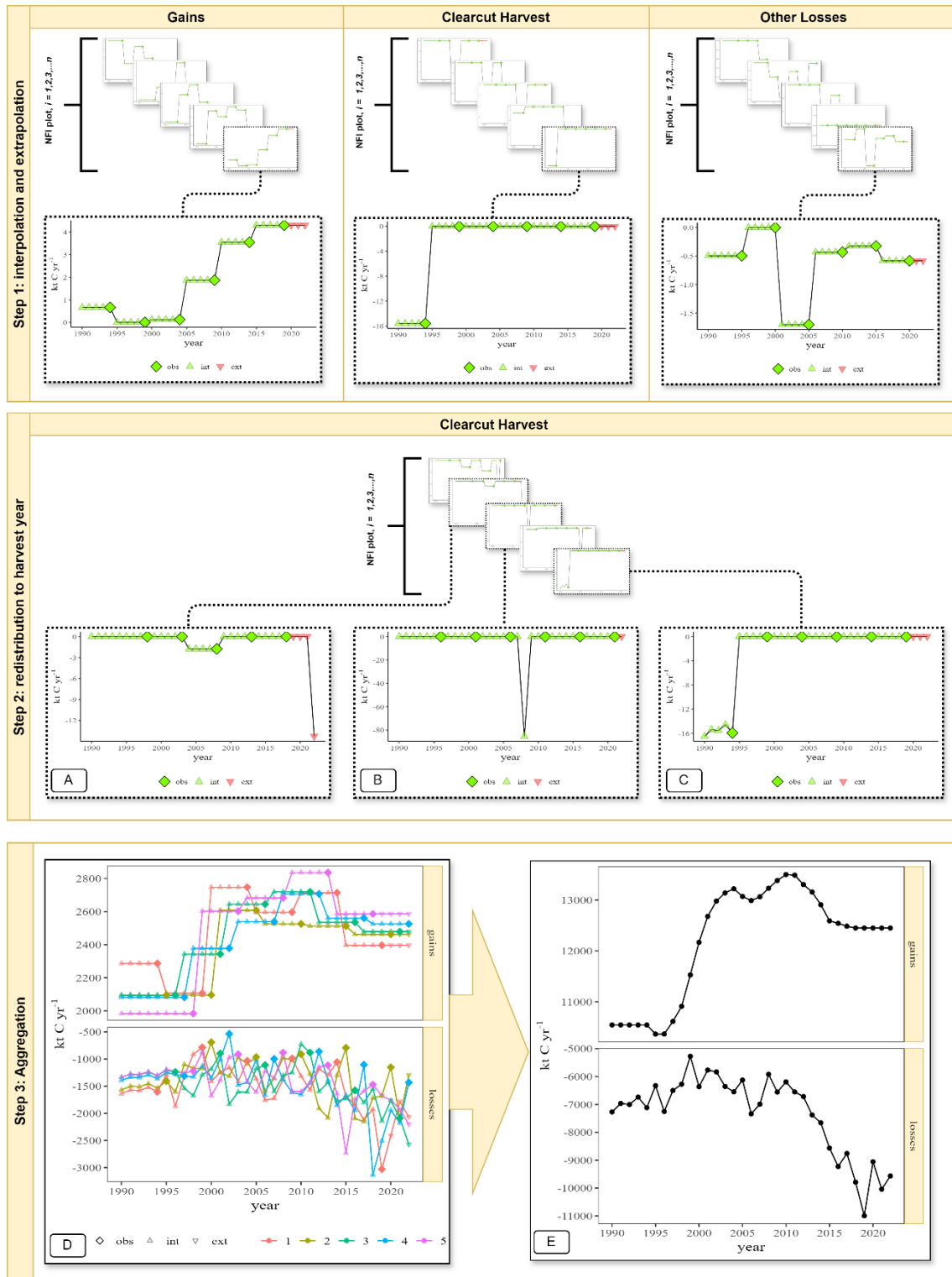
Figure 6.18: Workflow of interpolation-extrapolation processing steps. Step 1: linear interpolation (green triangles) is applied to observation (green diamonds) gains and losses for each NFI plot between each observation (green diamonds). Extrapolation (red upside-down triangle) is the average of the last 5 years (gains and other losses), except for plots with observed clearcut harvest in the time series, either from NFI registrations or Global Forest Change (GFC). In case of GFC detected loss, estimated biomass loss is calculated for the plot in the extrapolation period. Step 2: Living biomass losses
