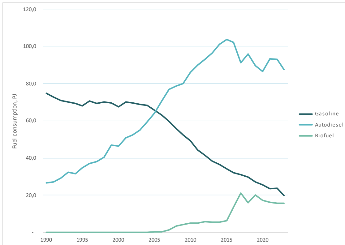
Figure 3.15: Consumption of gasoline, diesel and biofuel for road transportation. PJ. Source: Statistics Norway.
