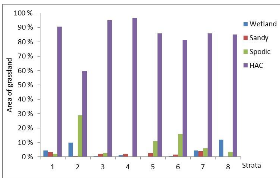
Figure 6.28: Distribution of soil types in intensive grassland areas for the eight strata. The IPCC soil types are high-activity clay soils (HAC): leptosols, fluvisol, phaeosem, albeluvisol, luvisol, umbrisol, cambisol, regosol; wetland soils: gleysols; sandy soils: arenosols; and spodic soils: podzol.
