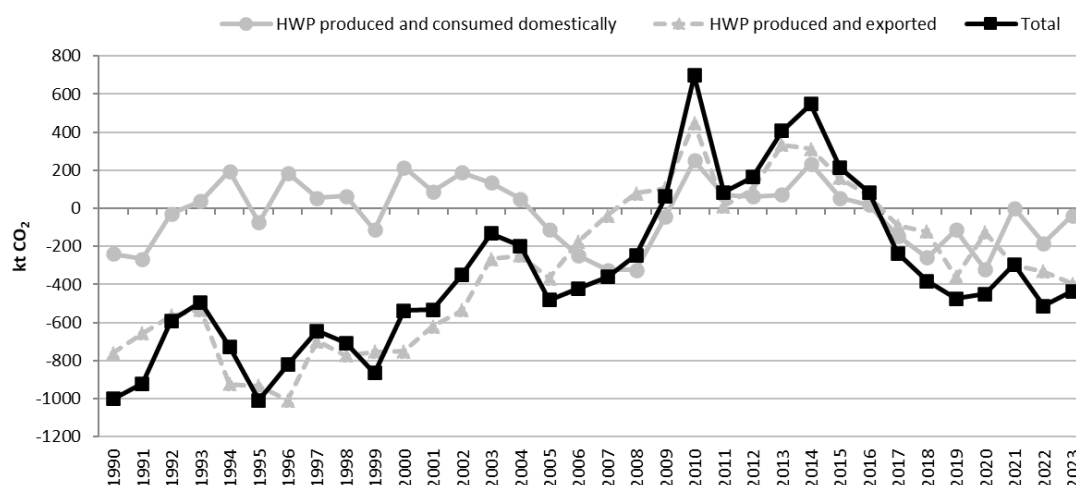
Figure 6.32: CO 2 emissions and removals in HWP (kt CO 2 ). Source: Norwegian Institute of Bioeconomy Research.
