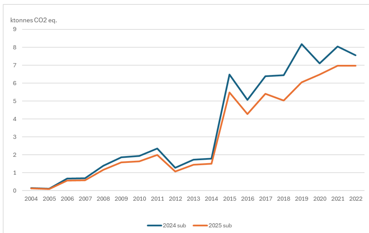
Figure 10.3: Recalculations illustrated for total emissions (kt CO 2 equivalents per year) estimated for 5B2a Anaerobic digestion of Municipal solid waste in the latest submission compared to the previous submission.
