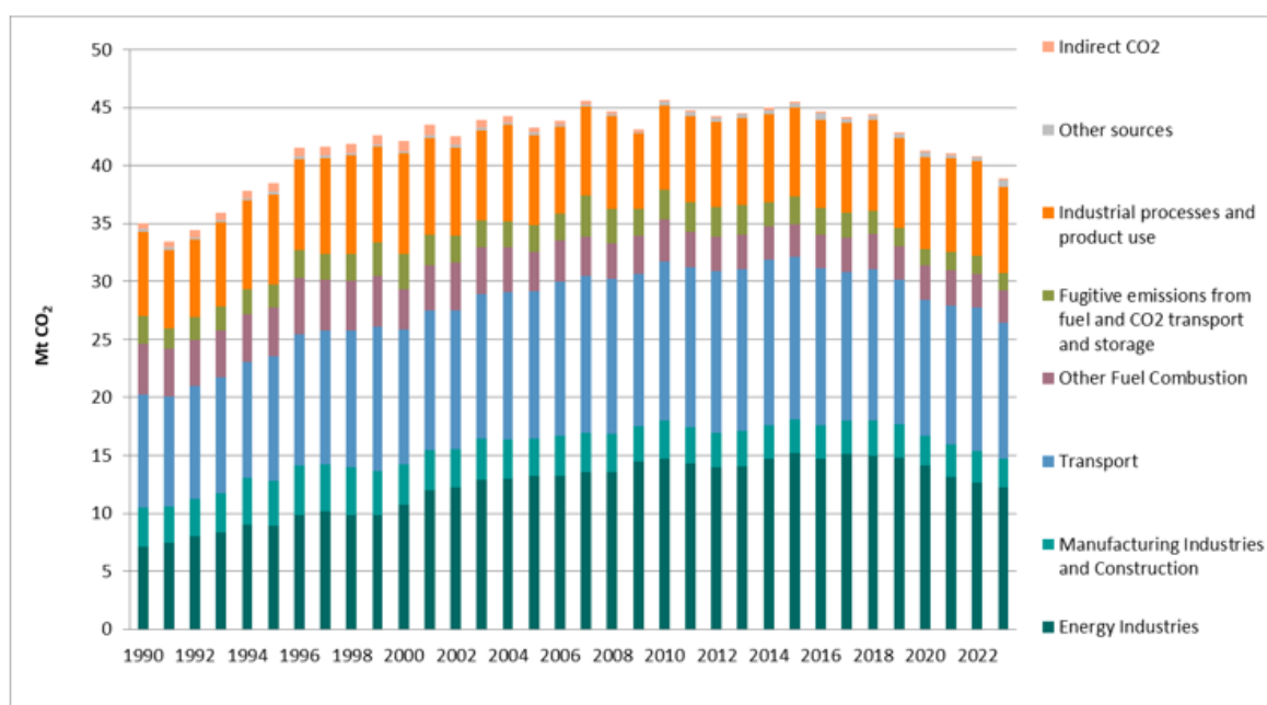
Figure 2.16: CO 2 emissions (Mtonnes) in Norway, 1990-2023. Source: Statistics Norway/Norwegian Environment Agency.
