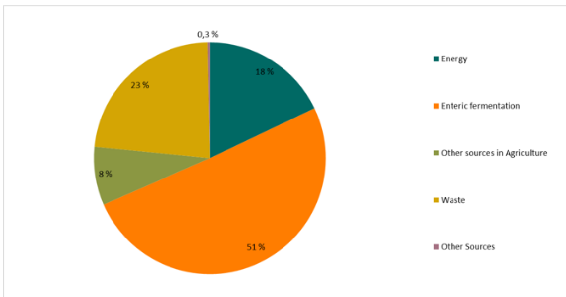
Figure 2.17: Distribution of Norwegian CH 4 emissions by major sources in 2023. Source: Statistics Norway/Norwegian Environment Agency.
