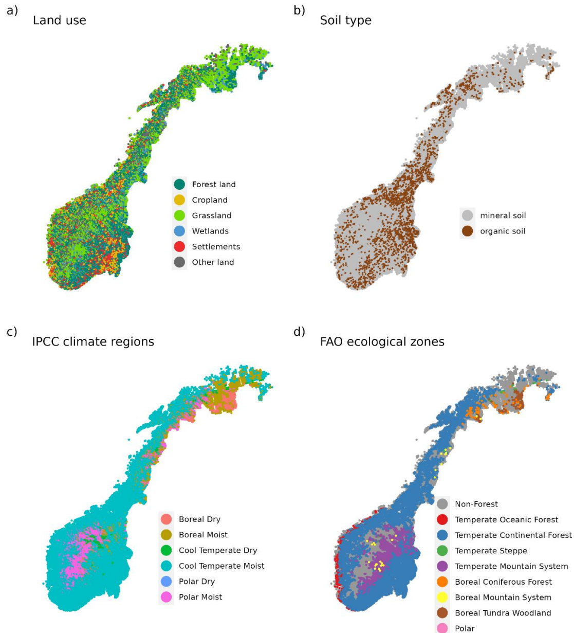
Figure 6.16: Map overview of NFI plot stratification: a) Current Land use categories; b) soil types; c) IPCC climate regions; d) FAO ecological zones for forest lands. The visual representation of each plot on the maps is altered to ensure the visibility of all categories, as the plotting order affects the visibility.
