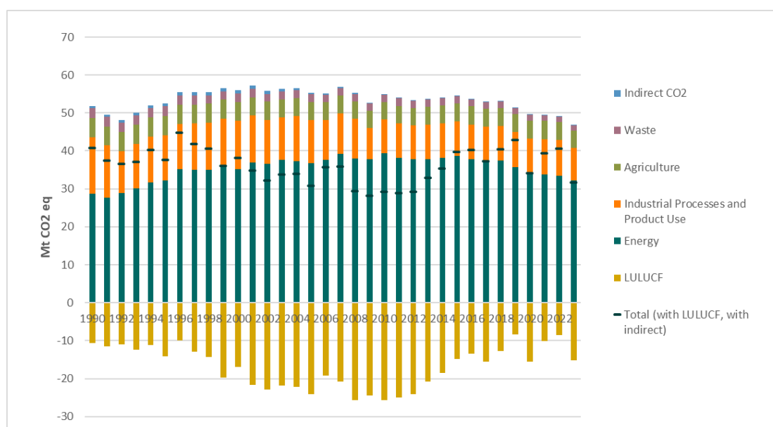
Figure ES.1: Total emissions of greenhouse gases by sources, and removals from LULUCF in Norway, 1990-2023 (Mtonnes CO 2 equivalents). Source: Statistics Norway/Norwegian Environment Agency/Norwegian Institute of Bioeconomy Research.
