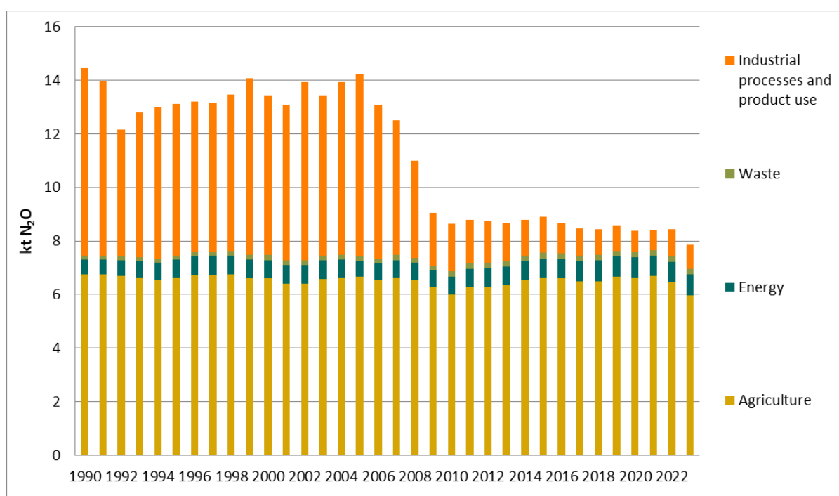
Figure 2.20: N 2 O emissions in Norway, 1990-2023, without LULUCF. Source: Statistics Norway/Norwegian Environment Agency.
