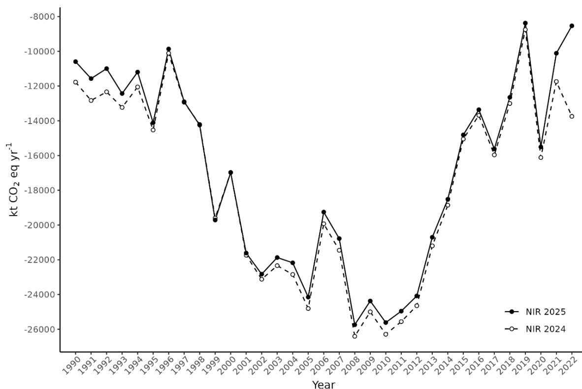
Figure 10.1: Recalculations illustrated for total emissions (kt CO 2 equivalents per year) estimated for the LULUCF sector in the latest submission compared to the previous submission.
