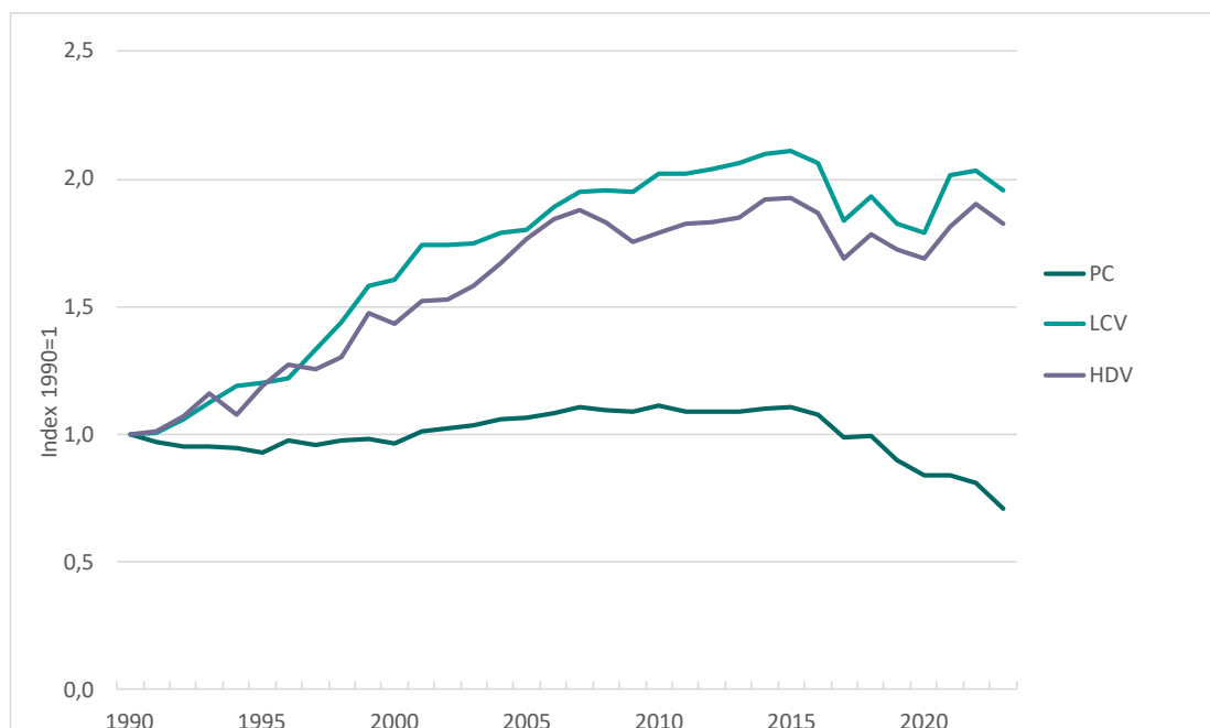
Figure 3.12: Relative change to 1990 in total CO 2 emissions from PC, LCV and HDV. Index 1990=1. Source: Statistics Norway/Norwegian Environment Agency.
