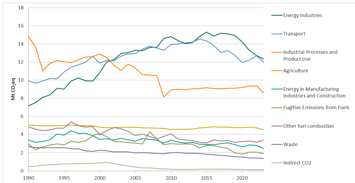
Figure 2.4: Development of emissions of all GHG (Mtonnes CO 2 eq.) from the different sectors (without LULUCF) 1990-2023. Indirect CO 2 emissions is also shown. Source: Statistics Norway/Norwegian Environment Agency.
