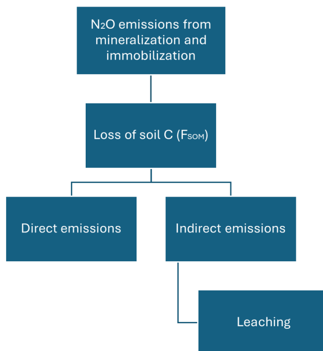
Figure 6.34: Reporting structure for Direct and Indirect N 2 O emissions from nitrogen mineralization and immobilization.
