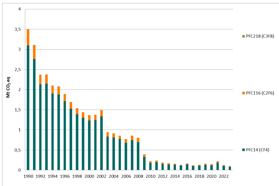
Figure 2.21: Emissions (million tonnes CO 2 eq) of PFCs in Norway, 1990-2023. Source: Statistics Norway/Norwegian Environment Agency.
