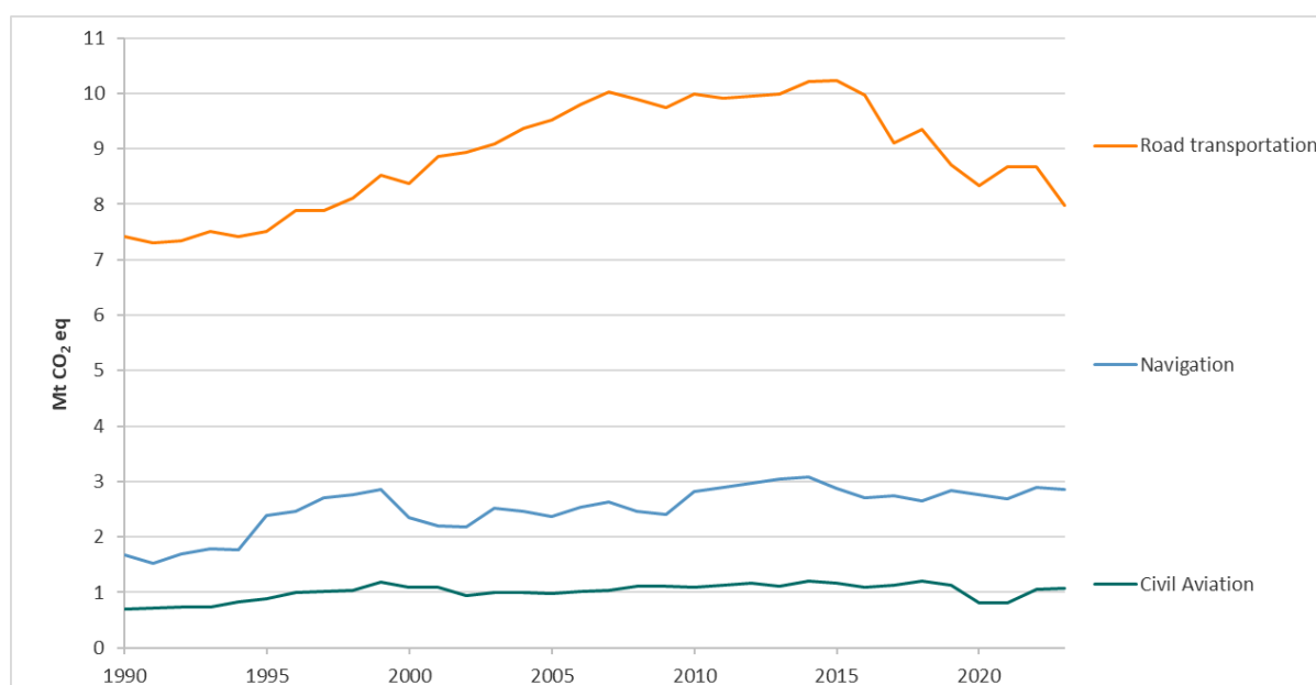
Figure 2.7: Emissions in million tonnes CO 2 equivalents from the most important modes of transport, 1990-2023. Source: Statistics Norway/Norwegian Environment Agency.
