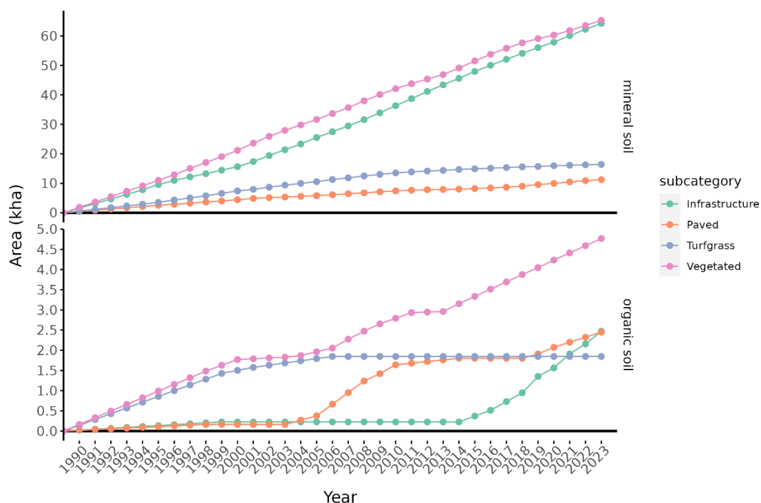
Figure 6.31: Cumulative land-use change area to settlement subcategories since 1990 (excluding 20-year transition rule to remaining category). The area separation between mineral and organic soil is based what the soil of the area was originally classified as before the conversion, and not the classification after land-use change.
