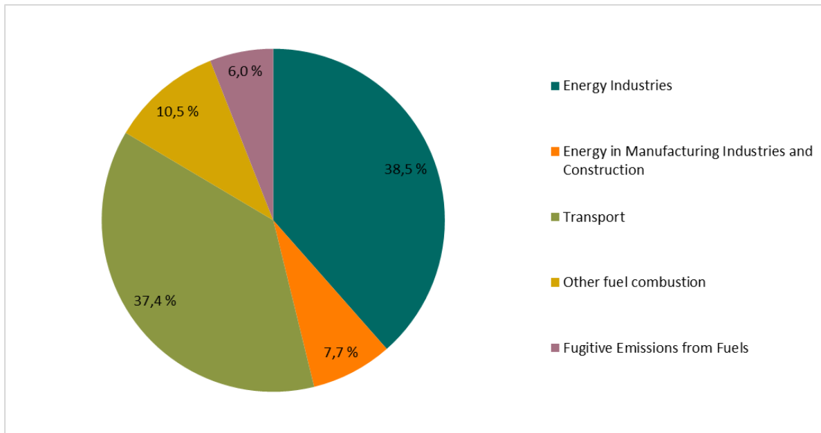
Figure 2.5: Greenhouse gas emissions in 2023 from the energy sector distributed among the different main source categories. Source: Statistics Norway/Norwegian Environment Agency.
