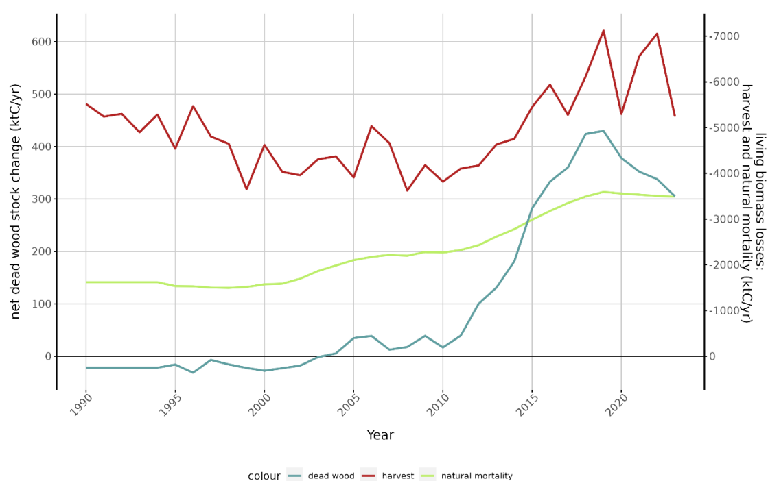
Figure 6.22: Temporal dynamics in natural mortality, harvest residues and Yasso07-simulated carbon stocks in the dead wood pool.
