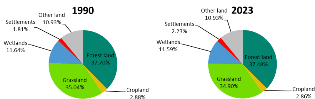
Figure 6.11: Area distribution of the IPCC land-use categories for 1990 and the latest reporting year. Source: Norwegian Institute of Bioeconomy Research.
