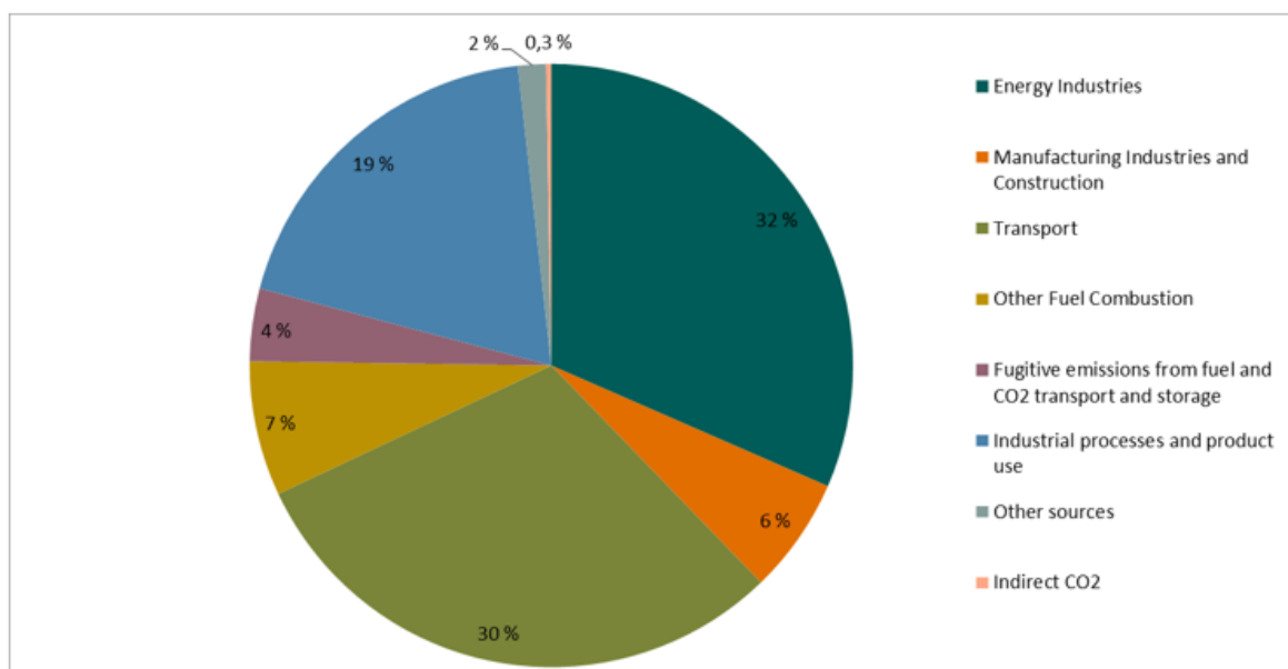
Figure 2.15: Distribution of CO 2 emissions in Norway by various source categories in 2023 (by mass).
