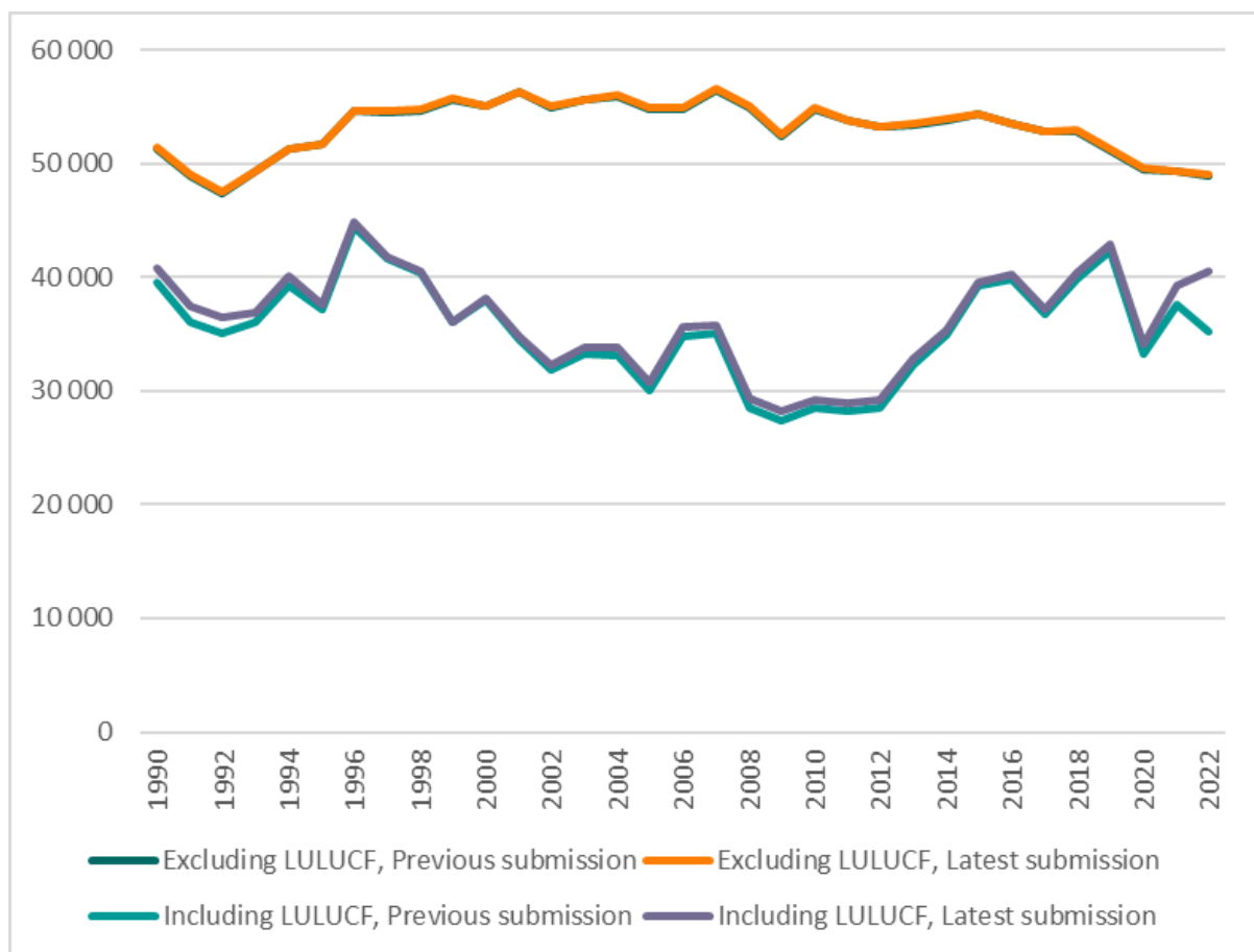
Figure 10.2: Total emissions with and without LULUCF. Previous and latest submission. 1000 tonnes CO 2 equivalents.
