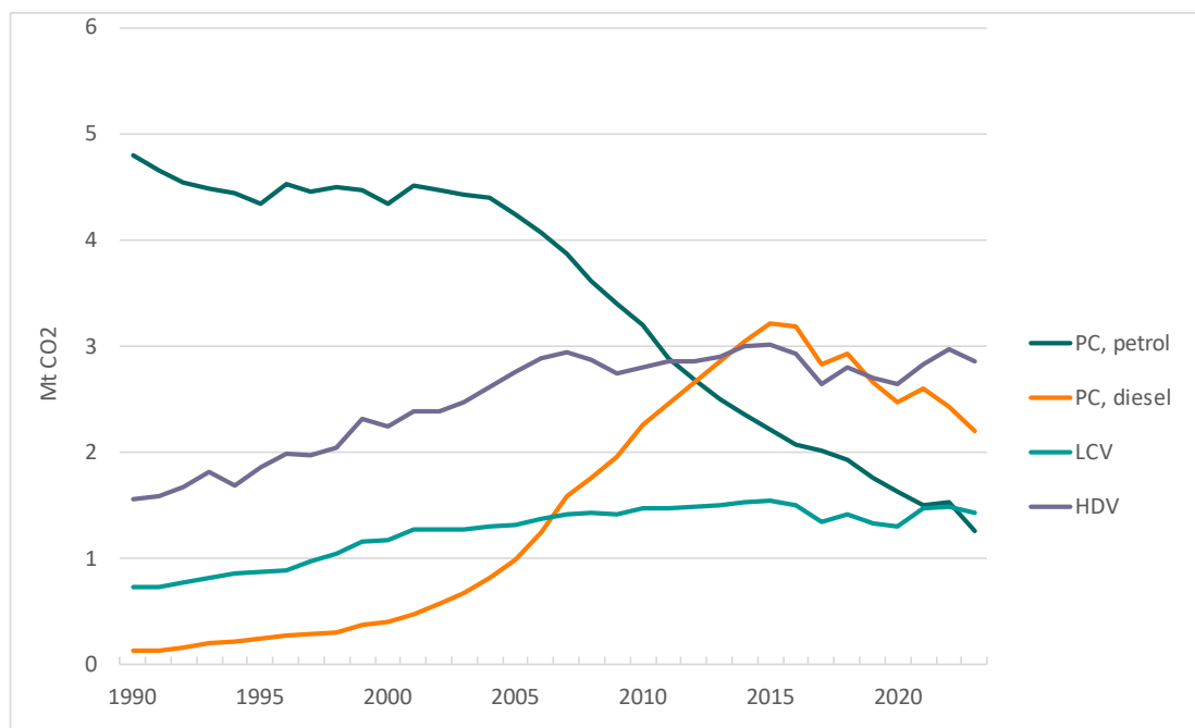
Figure 3.10: Emissions of CO 2 . PC petrol and diesel, LCV and HDV. Million tonnes. Source: Statistics Norway/Norwegian Environment Agency.
