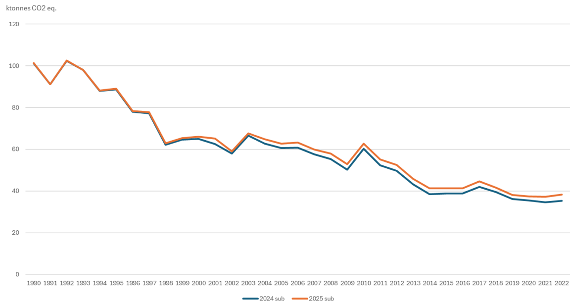
Figure 10.5: Recalculations illustrated for total emissions (kt CO 2 equivalents per year) estimated for 5D2 Industrial wastewater in the latest submission compared to the previous submission.
