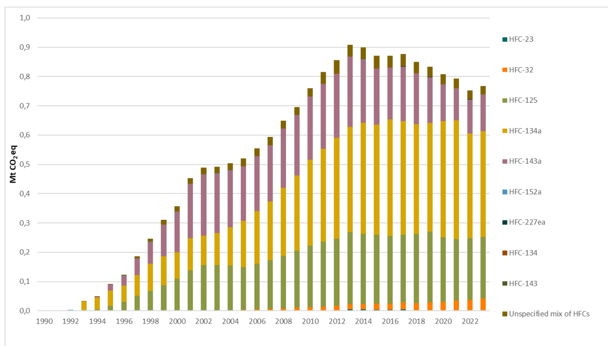
Figure 2.23: Emissions of HFCs (Mtonnes CO 2 eq.) in Norway, 1990-2023. Source: Statistics Norway/Norwegian Environment Agency.
