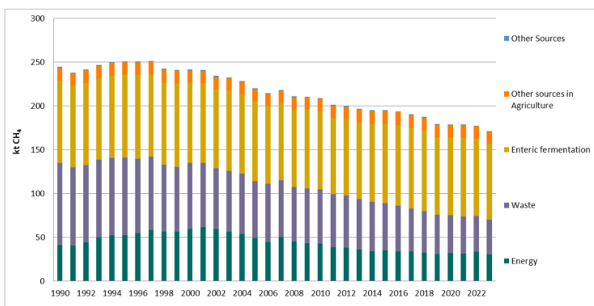
Figure 2.18: CH 4 emissions (ktonnes) in Norway, 1990-2023, without LULUCF. Source: Statistics Norway/Norwegian Environment Agency.
