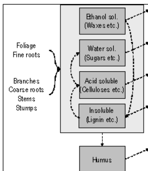
Figure 6.19: Flow diagram for chemical soil carbon pools in Yasso07. Fluxes significantly different from 0 are indicated by the arrows (Liski et al. 2009).
