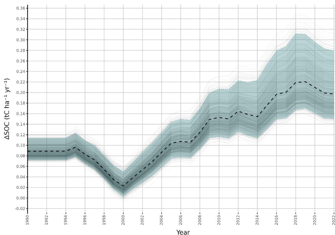
Figure 6.20: Uncertainty for CSC for SOC derived Monte Carlo simulations ( n = 1000 , faint grey lines). The cyan band indicates the 95% confidence interval derived for each year from the 2.5 th and 97.5 th percentile of the 1000 simulations. The dashed line indicated the mean of the 1000 simulations.
