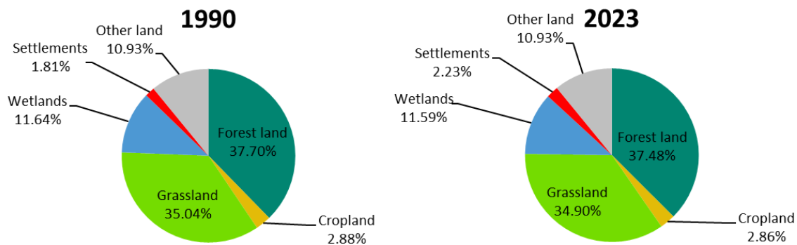
Figure 2.10: Area (%) distribution between the IPCC land-use categories, 1990 and 2023. Source: The Norwegian Institute of Bioeconomy Research.
