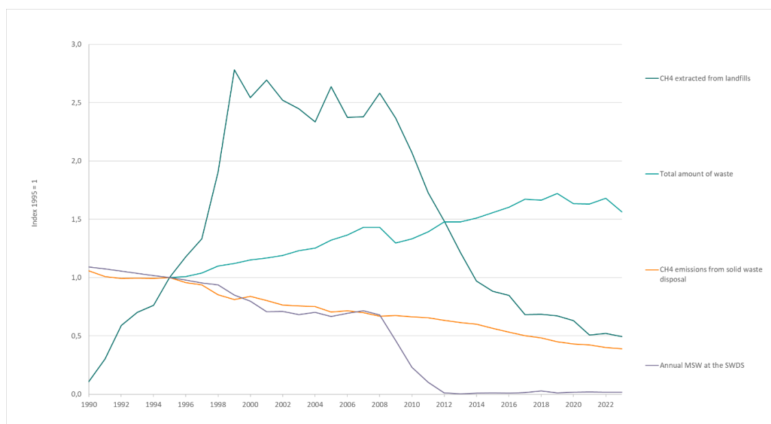
Figure 7.1: Relative change in methane emissions from solid waste disposal, annual MSW at the SWDS, methane extracted from landfills and total amount of waste generated in Norway. 1990-2023 Index 1995 = 1. Source: Statistics Norway/Norwegian Environment Agency.
