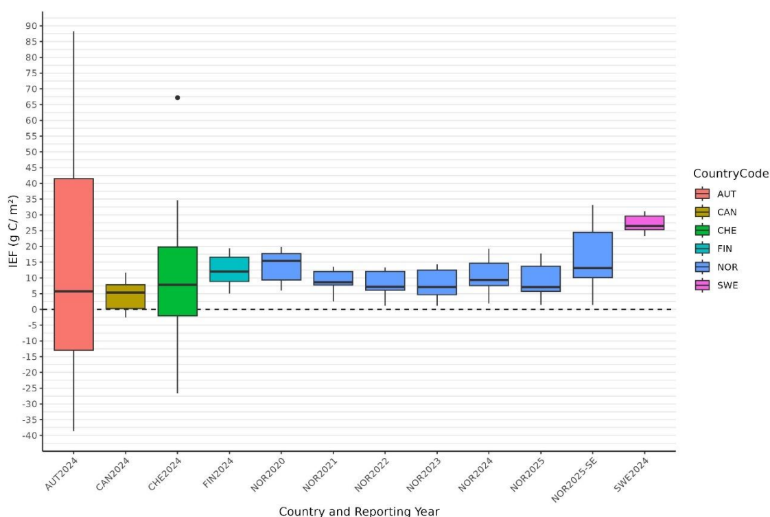
Figure 6.21: Boxplot of the sum of implied emission factors (IEF) 51 for dead wood, litter and mineral soil for forest land remaining forest land from CRT tables for the countries Austria (AUT), Canada (CAN), Switzerland (CHE), Finland (FIN), Sweden (SWE) and Norway (NOR). Except for Sweden and Canada, all countries presented use the Yasso model (v07 or v20), in varying degree, for dead wood, litter and mineral soil CSC. Canada uses a carbon budget model, CBM-CFS3 (Kurz 2009), and Sweden uses soil and dead wood measurements. Each boxplot consists of IEF for all the years for a given reporting year (the number after the country abbreviation). For Norway reporting years 2020, 2021, 2022, 2023, 2024 and 2025 are presented for the whole country, and south-eastern Norway only for the year 2025.
