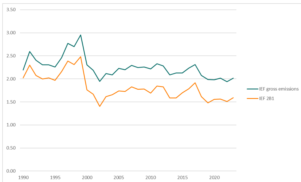
Figure 4.3: IEF for process emissions of CO 2 from ammonia production (tonne CO 2 /tonne ammonia).
