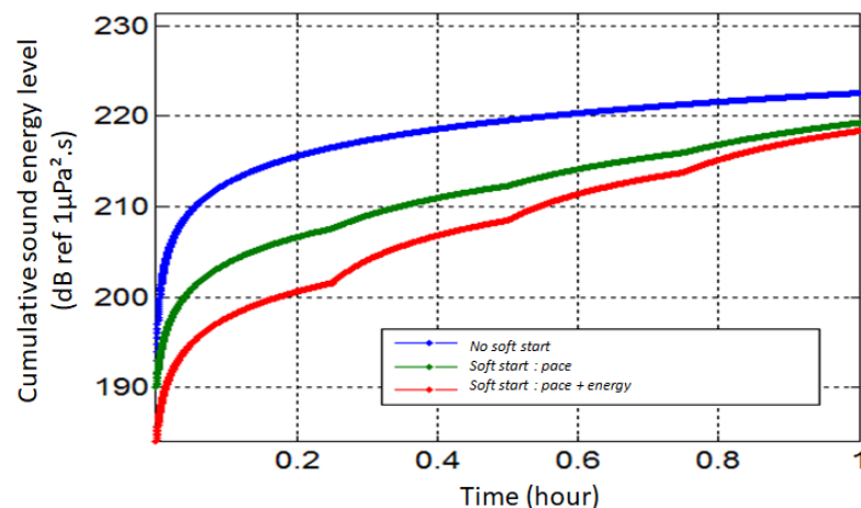
Figure 40: Theoretical comparison of the cumulative noise effects of a soft start of the work during the first hour of the construction site: without soft start (blue), soft increase in the rate (green) and soft increase in the rate and energy of the blows (red).
