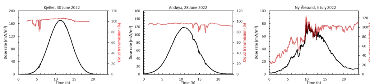
Figure 16: UV dose rates (left axis, black curves) and cloud transmission (right axis, red curves) during the days of maximum UVI at Kjeller (left panel), Andøya (middle panel) and Ny-Ålesund (right panel) in 2022. A cloud transmission of 100% represents clear sky conditions, whereas cloud transmissions of 20-30% represent heavy clouds.
