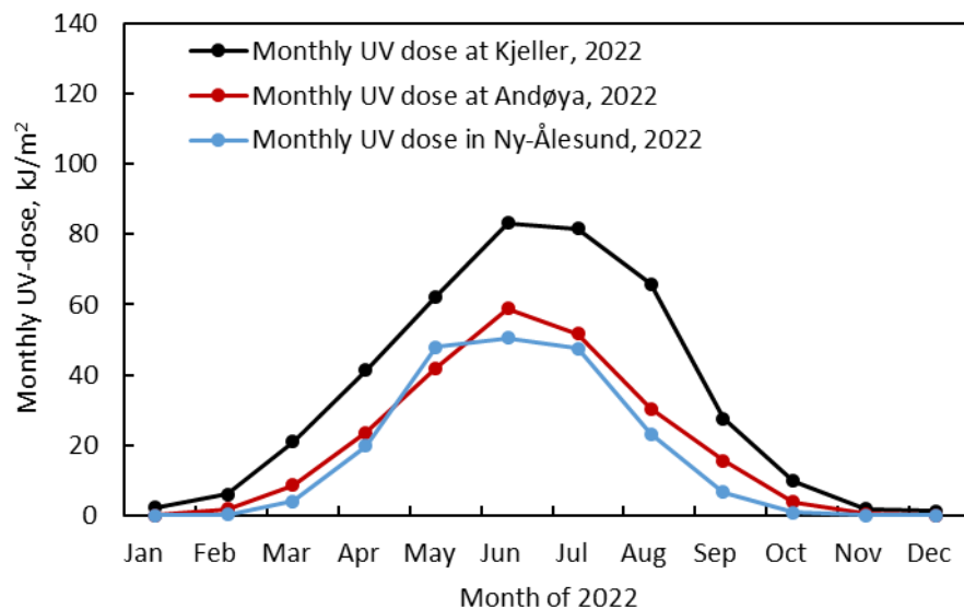
Figure 17: Monthly integrated UV doses (in kJ/m 2 ) in 2022 measured with the GUV instruments located at Kjeller, Andøya and in Ny-Ålesund.
