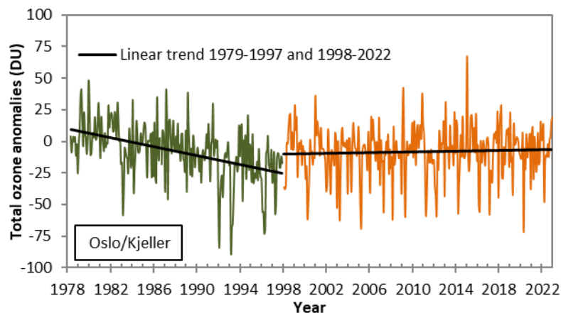
Figure 4b: Variation in total ozone over Oslo/Kjeller for the period 1979 to 2022 after the seasonal variations have been removed. The green line represents measurements performed with the Dobson instrument, whereas the orange line represents Brewer measurements. Trend lines are marked as black lines.
