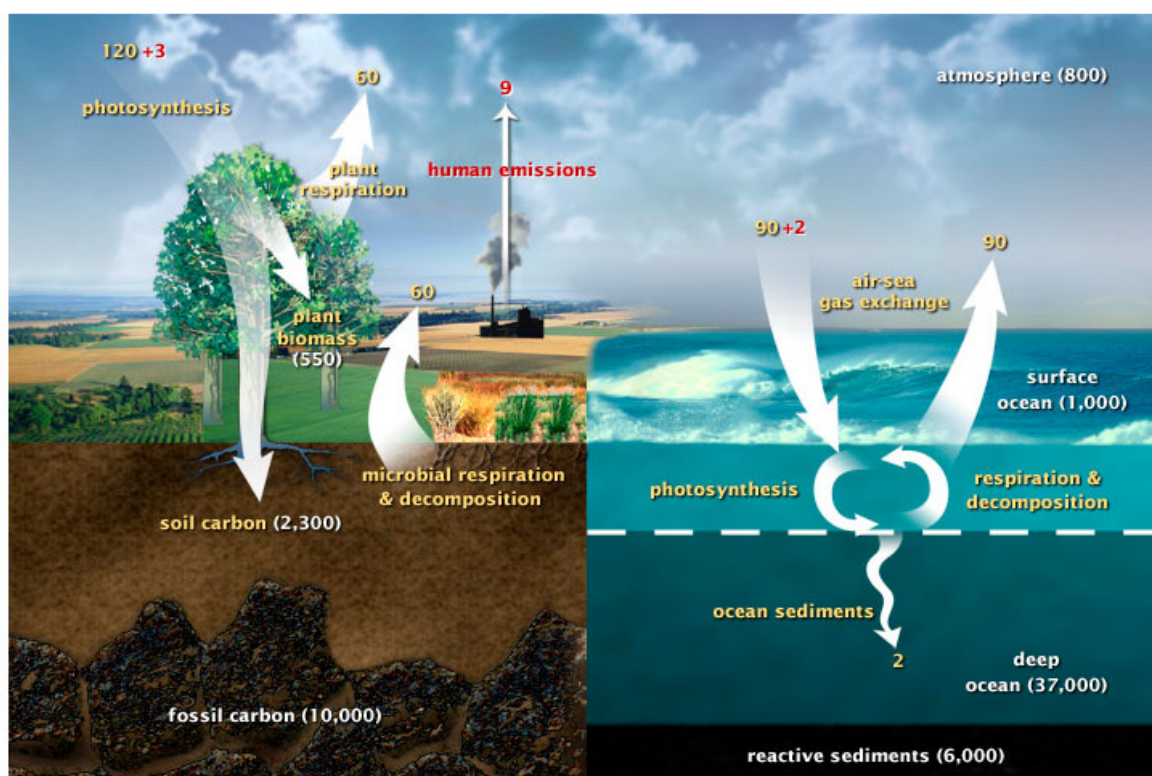
Figur 4.1 Karbonsirkulasjonen. ( https://earthobservatory.nasa.gov/features/CarbonCycle# )
