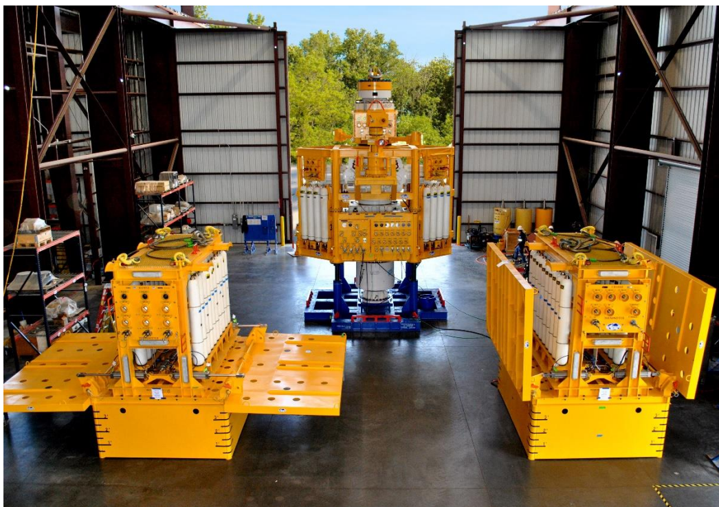
Figure 10 Trendsetter Arctic Class 18 ¾" 15,000 psi drill through Mudline Closure System (Courtesy of Trendsetter Engineering)
