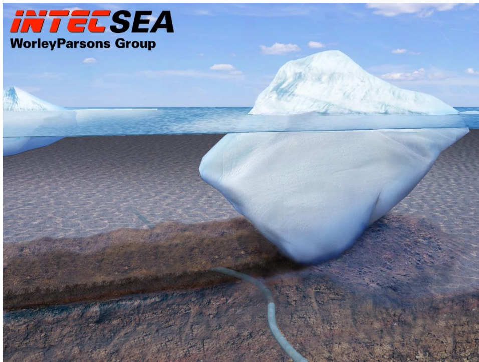
Figure 12 Iceberg scour (Courtesy of INTECSEA)
