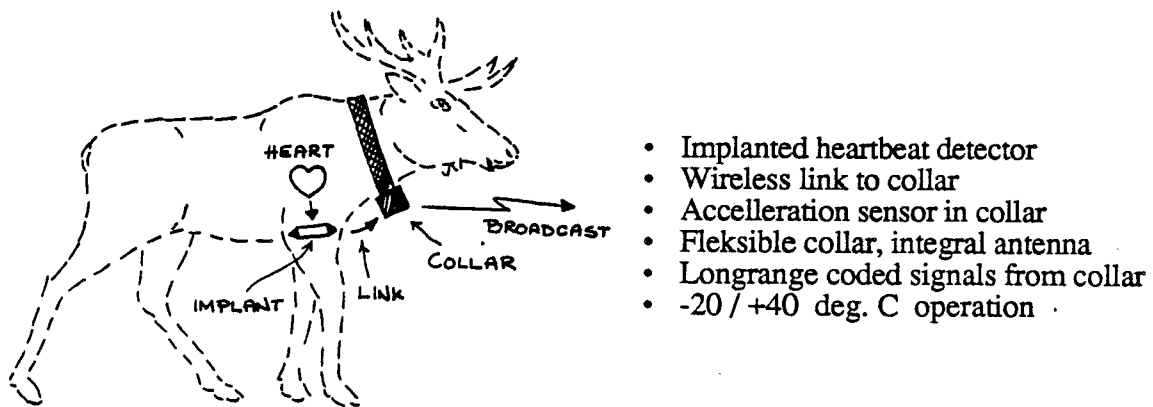
FIGURE 1. TRE-5 SYSTEM
