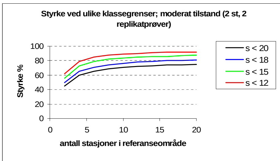
Figure 11. Results of power analysis for number of species (S) of soft-bottom fauna per 0.1 m 2 as a function of number of stations in a reference area. The different lines show different good/moderate boundaries. The analysis is based on two replicate samples from two stations in an impacted site, which is in accordance to the minimum requirements in Norwegian Standard method for sublittoral soft-bottom fauna.
