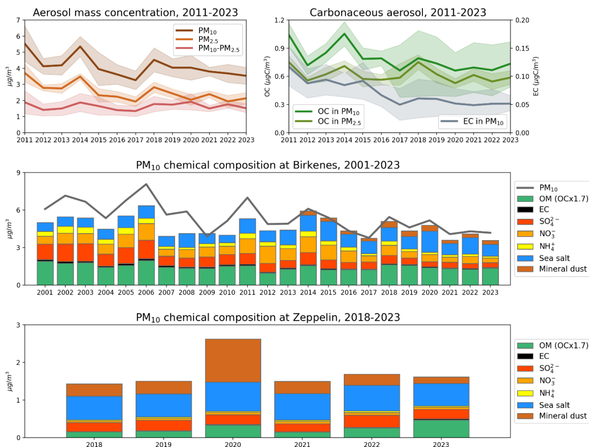
Figure 5.2: Trends for PM 10 , PM 2.5 , and PM 10-2.5 (upper left) and carbonaceous aerosol (OC and EC) (upper right) averaged for Birkenes Observatory, Hurdal and Kårvatn (2011 – 2023). Mass closure for PM 10 at Birkenes (middle panel) (2001 - 2023), and Zeppelin (lower panel) (2018 – 2023).
