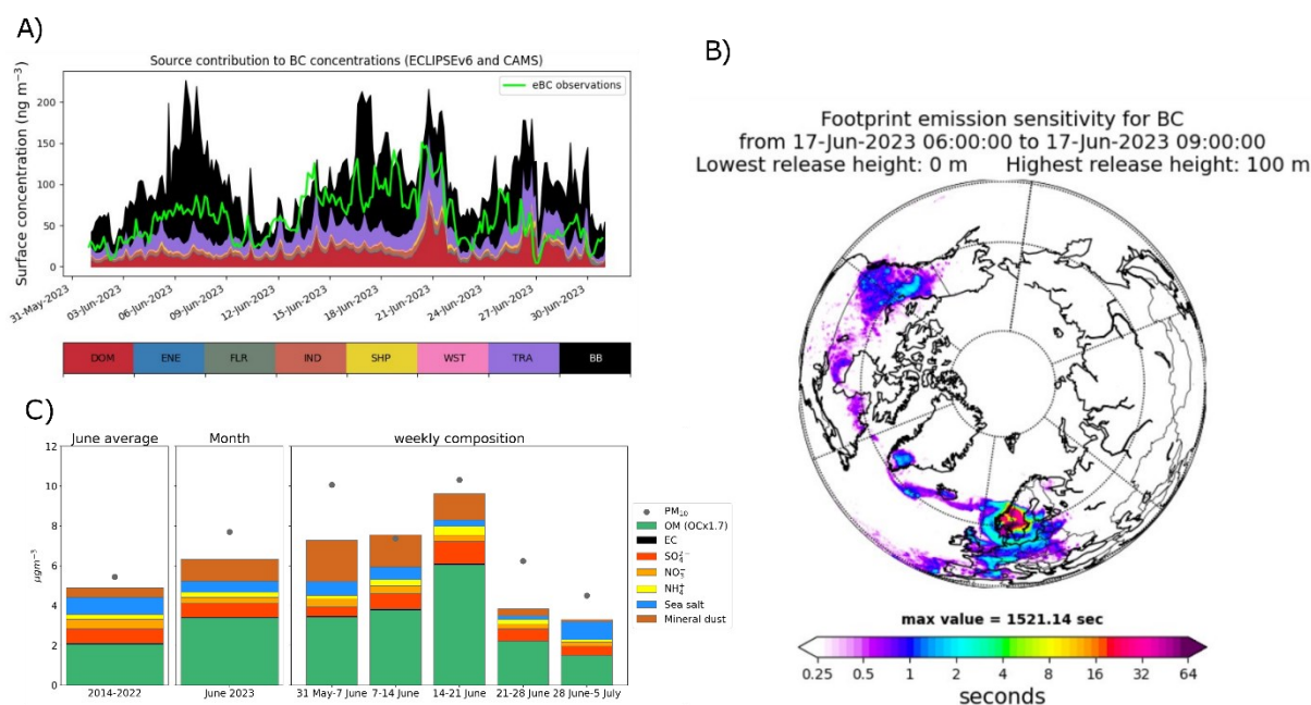
Figure 4.3: Observed concentrations of equivalent black carbon (eBC) and BC emitted from various sources (DOM = Domestic; ENE = Energy; FLR = Flaring; IND = Industry; SHP = Shipping; WST = Waste; TRA = Traffic; BB = Wild fires) calculated by FLEXPART for Birkenes June 2023 (panel A); Flexpart footprint of the airmasses arriving 17 June at Birkenes calculated with the Flexpart model (Pisso et al., 2019). The unit (second) shows the residence time in the surface layer (100 m) of the air masses arriving at the actual date (panel B); Mean chemical composition of PM 10 at Birkenes for: June 2014 – 2022 (panel C, left), June 2023 (panel C, middle), and for 31 May to 5 July 2023 (panel C, right).
