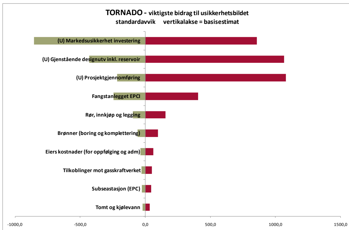
Figur 3 Tornadodiagram investeringskostnader
