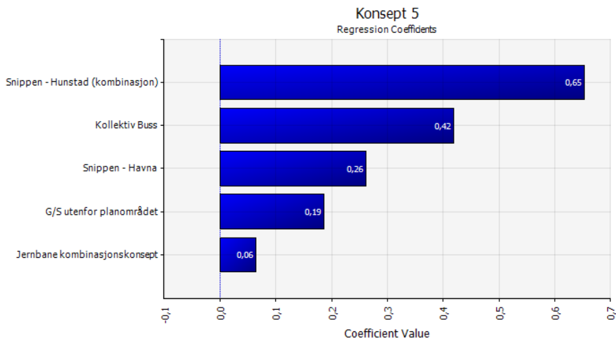
Figur 13: Tornado Konsept 5
